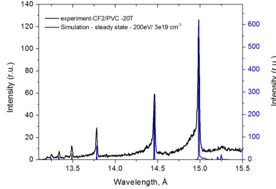
Figure 2.18.: Best fit of the X-ray spectrum measured near the obstacle (PVC target, the stream being generated from a CF2 target) in the case of a magnetic field strength of B = 20 T and as obtained by the PrismSPECT code in steady-state mode for an electron temperature of 200 eV, or 2.32 MK.
