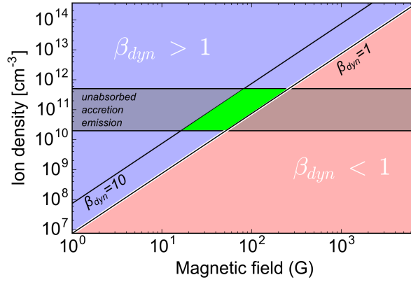
Figure 2.11.: Dynamic- \beta variation as a function of the magnetic field and the ion density, for a CTTS accretion column with free fall velocity of 500 \text{ km s}^{-1} . The red filled-in part represents the area for which the couple magnetic field - ion density gives a \beta_{dyn} < 1 , while the blue filled-in zone represents the region for which \beta_{dyn} > 1 . The separation line, \beta_{dyn} = 1 , is represented by the white diagonal. Additional black diagonals display the \beta_{dyn} = 1 and \beta_{dyn} = 10 experimental range. The horizontal gray rectangle highlights the 2 \times 10^{10} - 5 \times 10^{11} \text{ cm}^{-3} density range, corresponding to the observable accretion emission due to the non-absorption of their shocked emissions, through sinking into the chromospheric material (following the study of Ref. Sacco et al. (2010) - see text). The green area represents the CTTS ion density and the magnetic field modeled by the experiment – this leads to an accessible magnetic field strength range of 20 – 200 G.
