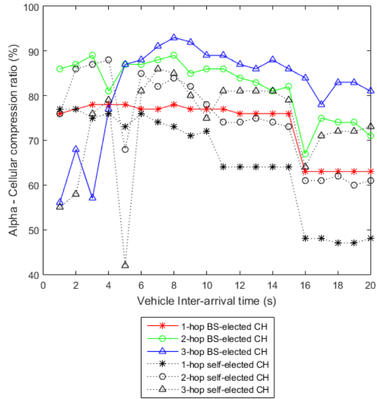
Figure 5.14: Global data compression ratio: Comparison between CH self-appointment and BS-based CH selection algorithms, for different maximum numbers of hops.
