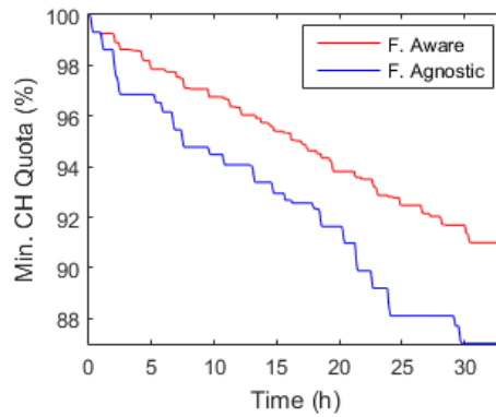
Figure 7.6: Minimum available cellular quota among the vehicles having served as CH during the simulation.
