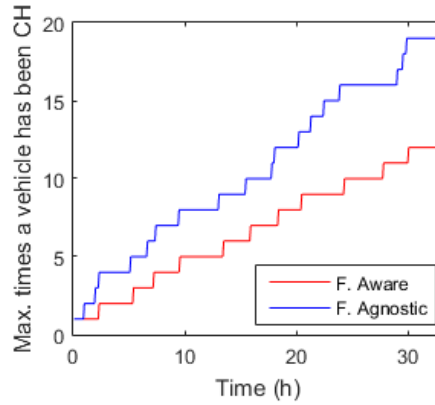
Figure 7.3: Maximum number of times that any one vehicle has served as CH in function of time.
