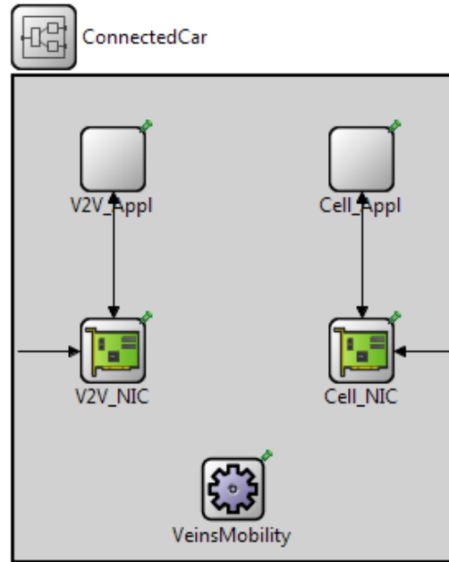
Figure 4.2: Visualization of the components of a Connected Car NED file.
