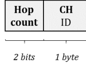
Figure 5.8: Structure of the Join messages
