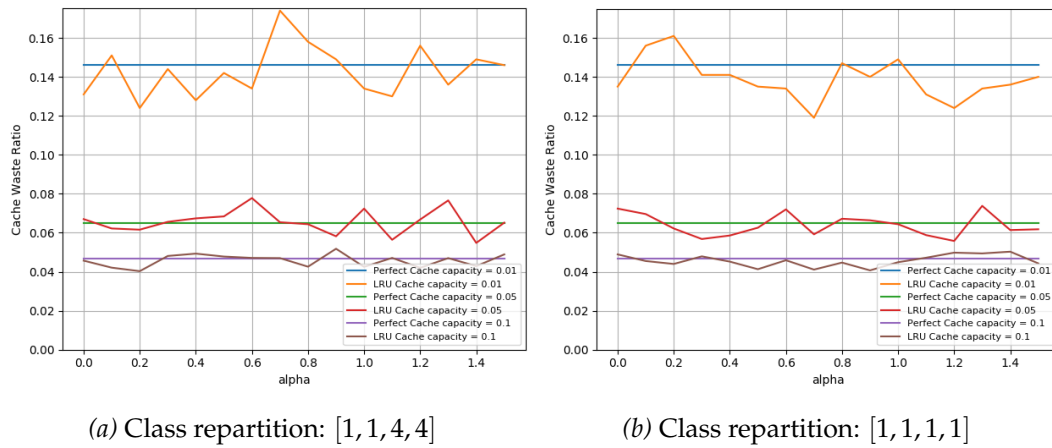
Figure 5.4: Cache waste ratio for various class repartitions and cache capacities. Results are shown for LRU and perfect cache, only when fragment caching.
