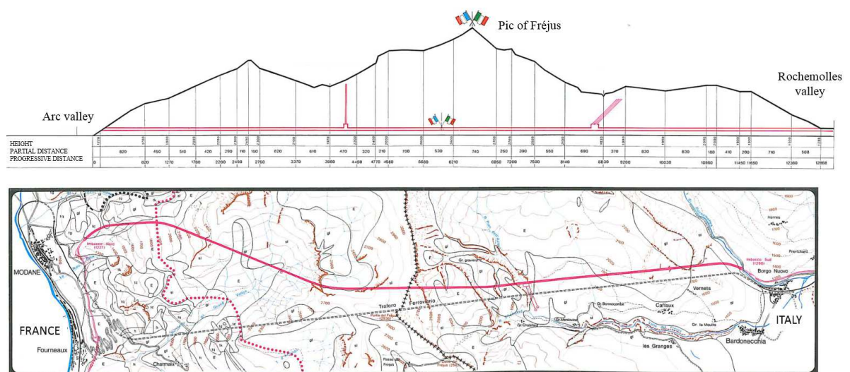
Fig. 5.1 Track alignment in red (bottom) and longitudinal profile (top) of the road tunnel after SITAF (1982) [the railway tunnel is shown by the discontinuous grey line]
