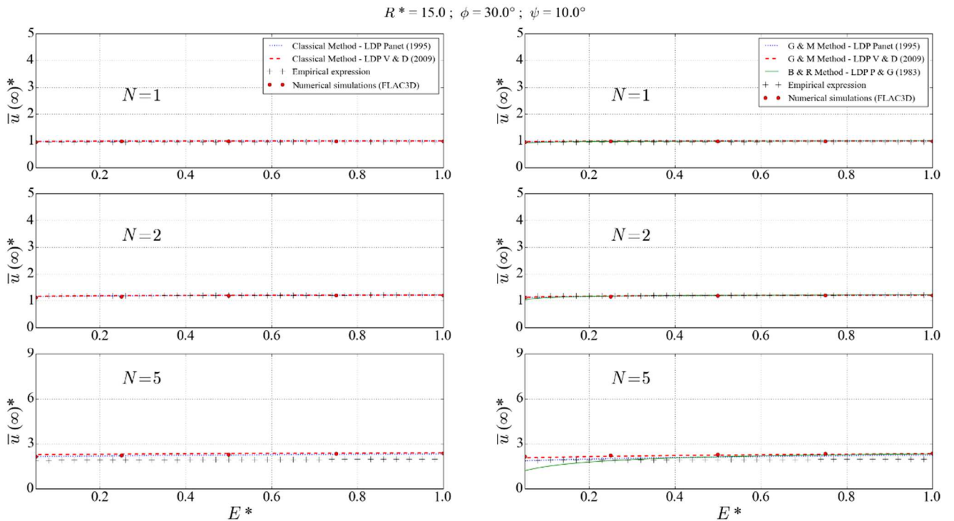
Comparison of \bar{u}(\infty)^* between the different approaches when R^*=15 and \phi=30^\circ for non-associate plasticity ( \psi = \phi/3 ). Classical methods on the left column and implicit methods on the right column
