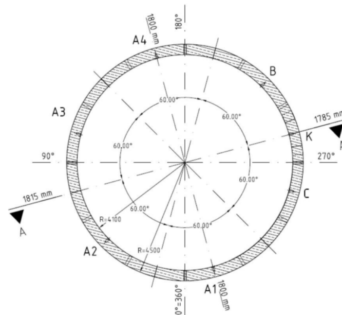
Fig. 6.5 Geometric characteristics of a ring of the lining installed in the safety gallery
