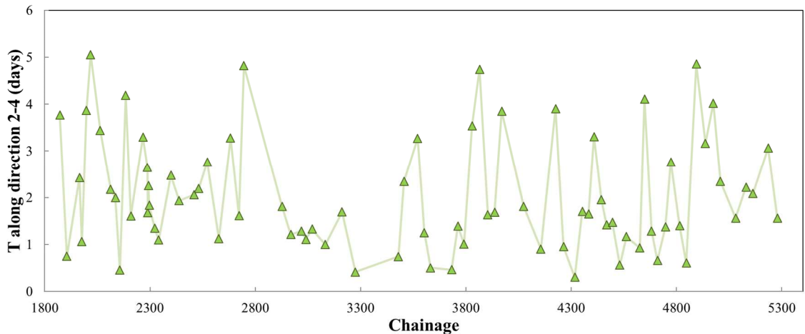
Fig. 5.13 Evolution of T along direction 2-4 along the road tunnel after De la Fuente et al., (2017)
