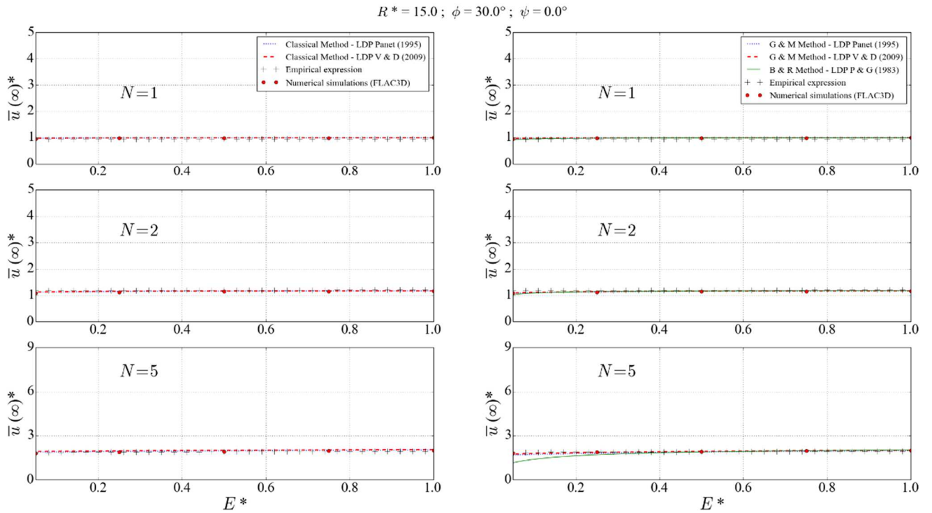
Comparison of \bar{u}(\infty)^* between the different approaches when R^*=15 and \phi=30^\circ for incompressible plasticity ( \psi = 0 ). Classical methods on the left column and implicit methods on the right column
