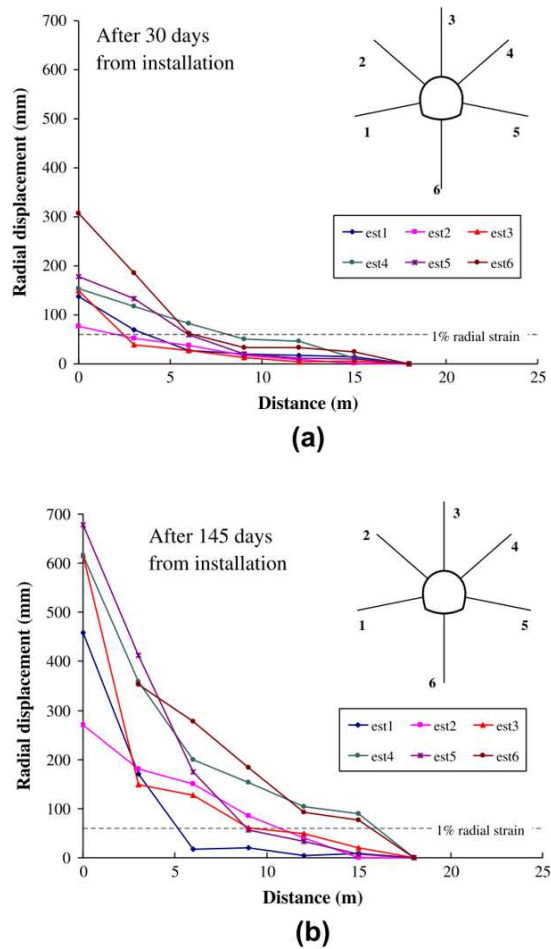
Fig. 1.13 Radial displacements from multi-point borehole extensometers installed at chainage 1330 m in Saint-Martin-la-Porte access adit after (a) 30 and (b) 145 days from installation after Bonini & Barla (2012)
