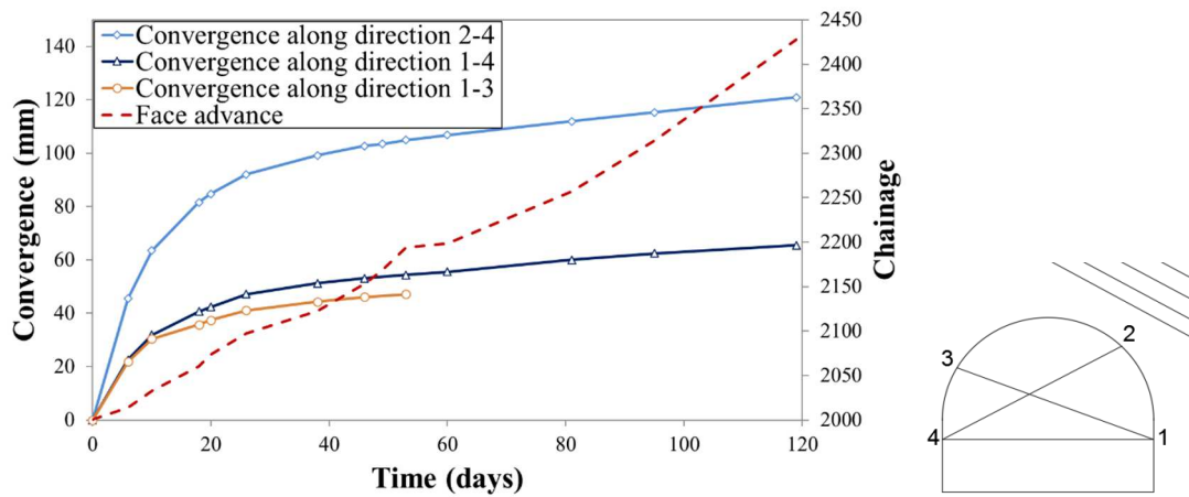
Fig. 5.8 Convergence curves and schematic position of the targets in section 13 (chainage 1998)
