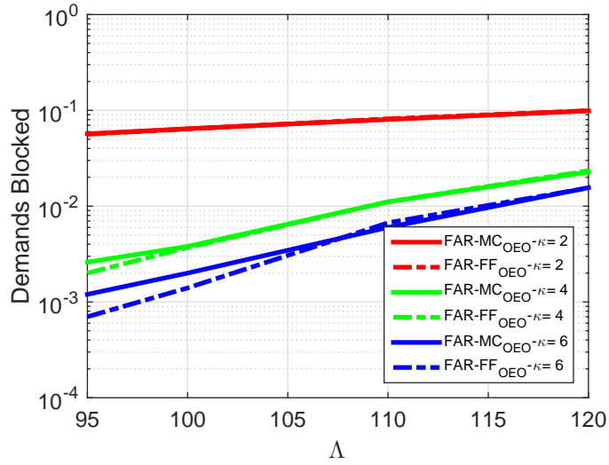
Figure 5.5: Blocking versus arrival rate ( \Lambda ) using \text{FAR-FF}_{\text{OEO}} and \text{FAR-MC}_{\text{OEO}} heuristics at different \kappa .
