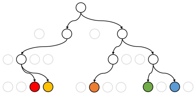
(b) Octree
