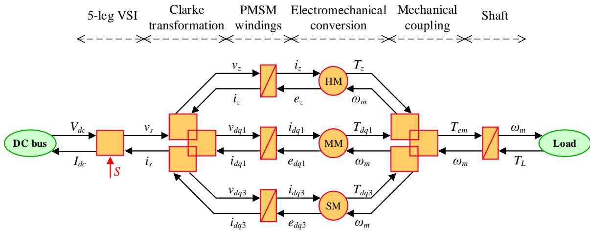
Figure 2.21. EMR for a five-phase PMSM.
