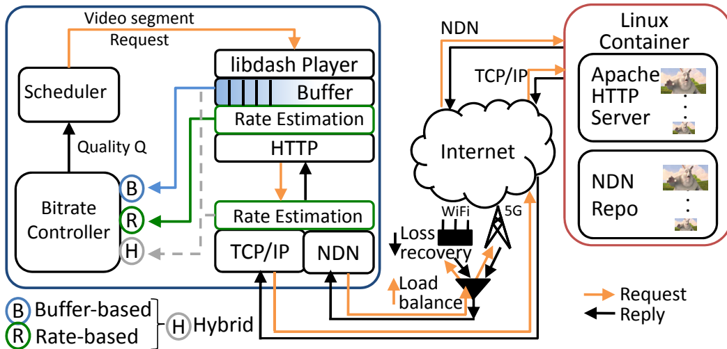
Figure 3.1: Synoptic of the DAS video streaming architecture used for the ICP/NDN vs TCP/IP comparison.
