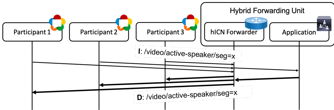
Figure 5.5: hICN-RTC architecture: downlink message exchange
