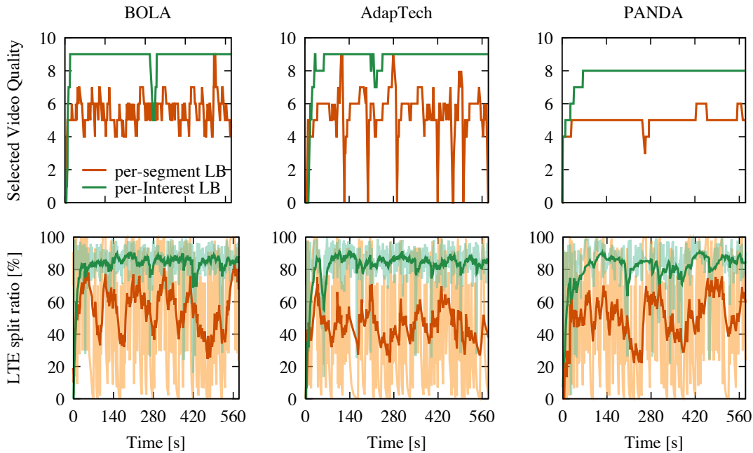
Figure 3.11: In-network support: load-balancing among WiFi and LTE interfaces. Top plots show the instantaneous requested quality for segment vs Interest-level load balance. Bottom plots show the percentage of segments vs Interest packets aired over the LTE interface using EWMA smoothing.
