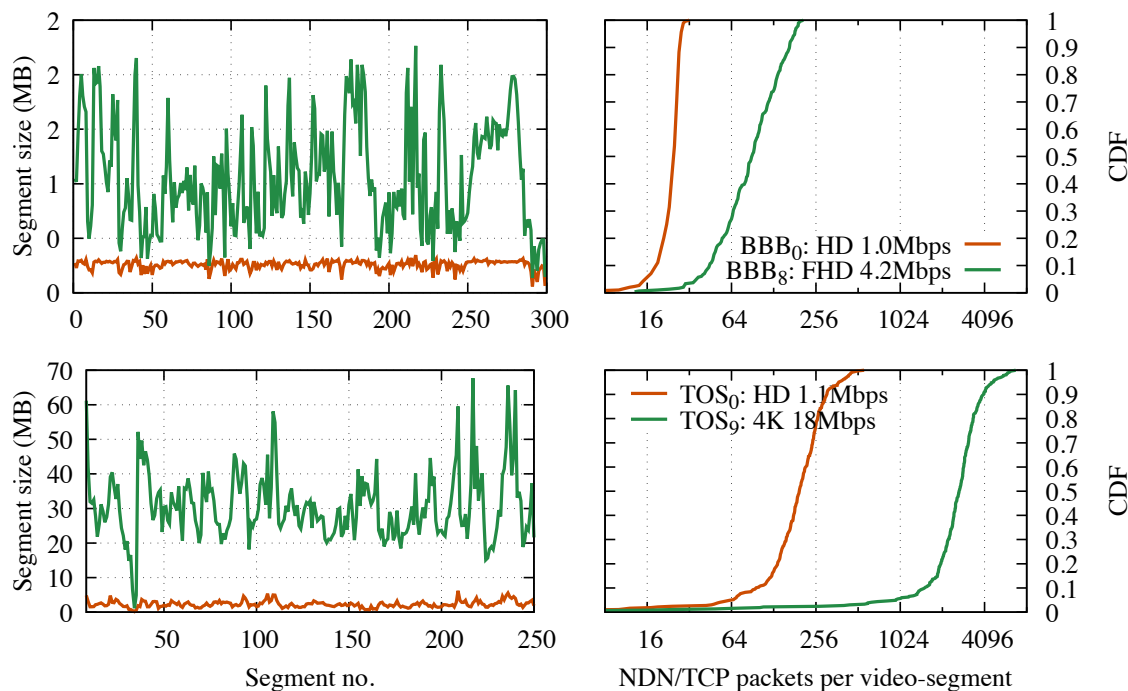
Figure 3.2: Highest and lowest quality representations for the BBB (top) and TOS (bottom) video: temporal evolution of video segment size (left) and cumulative distribution function of the number of TCP/NDN messages per video-segment (right).
