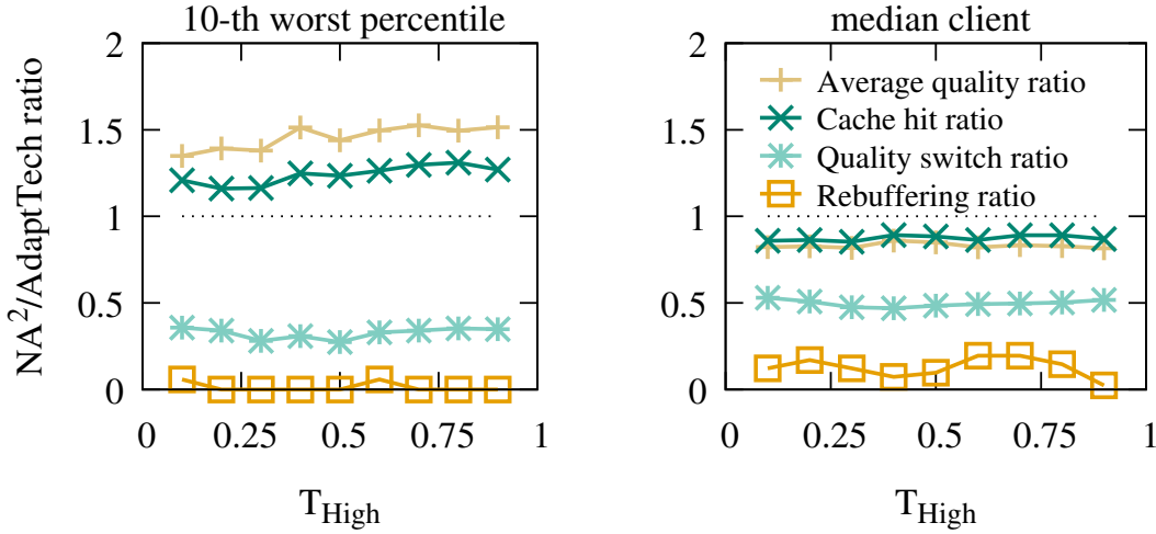
Figure 4.4: Sensitivity analysis: ratio of Network Aware vs Network blind performance for the 10-th worst percentile of clients (left) and for the median client (right).
