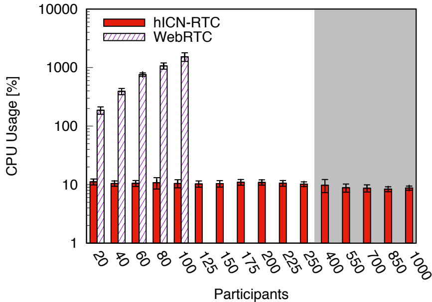
Figure 5.11: CPU usage.
