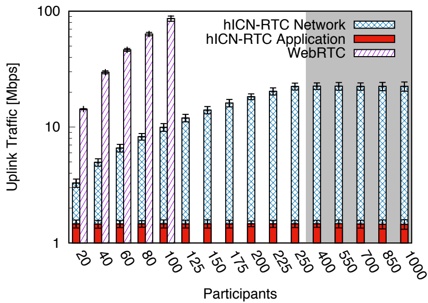
Figure 5.9: Uplink traffic.
