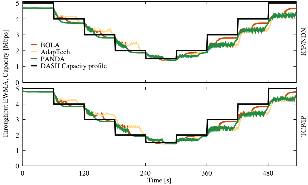
Figure 3.3: Time evolution of the estimated throughput for the three selected strategies (EWMA smoothed version) and DASH capacity profile.
