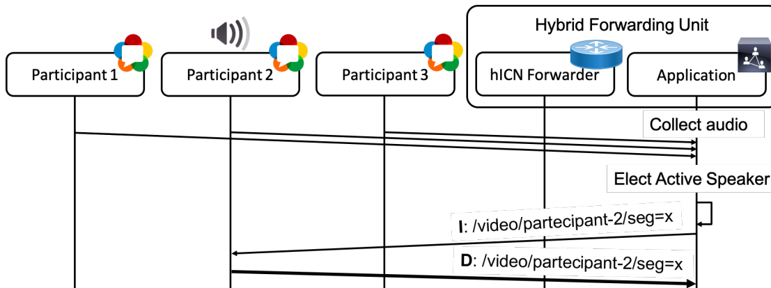
Figure 5.4: hICN-RTC architecture: uplink message exchange
