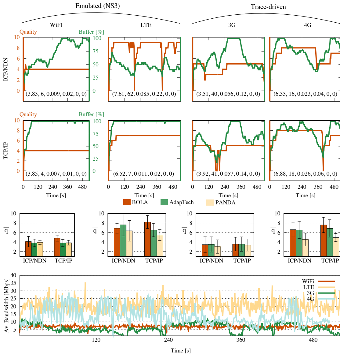
Figure 3.10: Access technologies: Emulated NS3 Wi-Fi and LTE (left columns) vs Trace-Driven 3G/4G (right columns). Top picture reports the AdapTech case as an example, annotated with (\bar{q}, \#QS, f_{QS}, |\Delta(QS)|, R, RTIME) performance details. Middle bar charts report average quality (with 95% CI over 10 runs) for all DAS strategies. Plot in the bottom row illustrates the available bandwidth with the different access technologies and emulation techniques.
