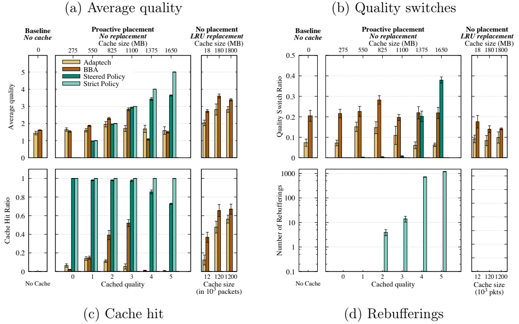
Figure 4.1: Design space at a glance: plots (a)-(d) show a key performance metric, with different subplots for different scenarios, i.e., baseline (left), proactive placement without replacement (middle) and no placement with LRU replacement (right). The bottom x-axis reports the quality cached at the router (in the proactive placement scenario) or the cache size in number of data packets (in the LRU replacement scenario), while the top x-axis reports the equivalent cache size in MB (both scenarios).
