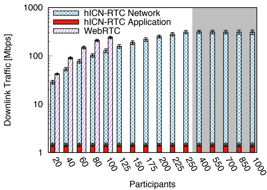
Figure 5.10: Downlink traffic.
