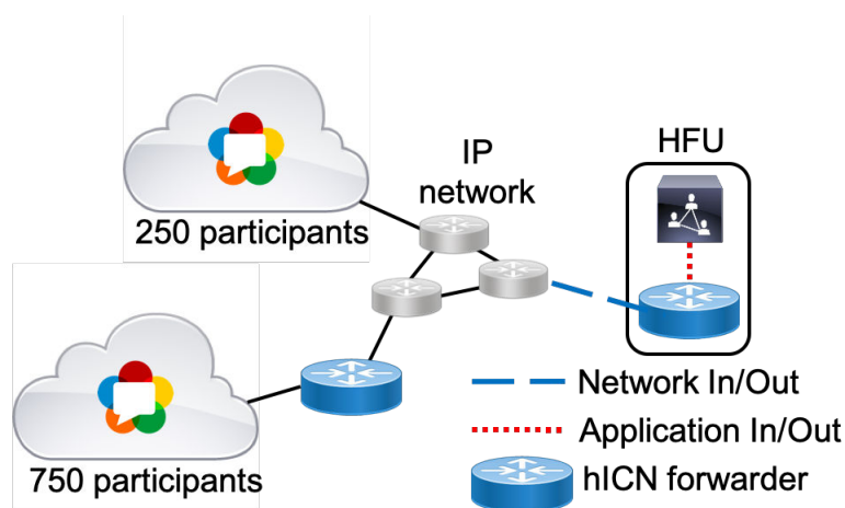
Figure 5.8: Topology used for scalability tests.
