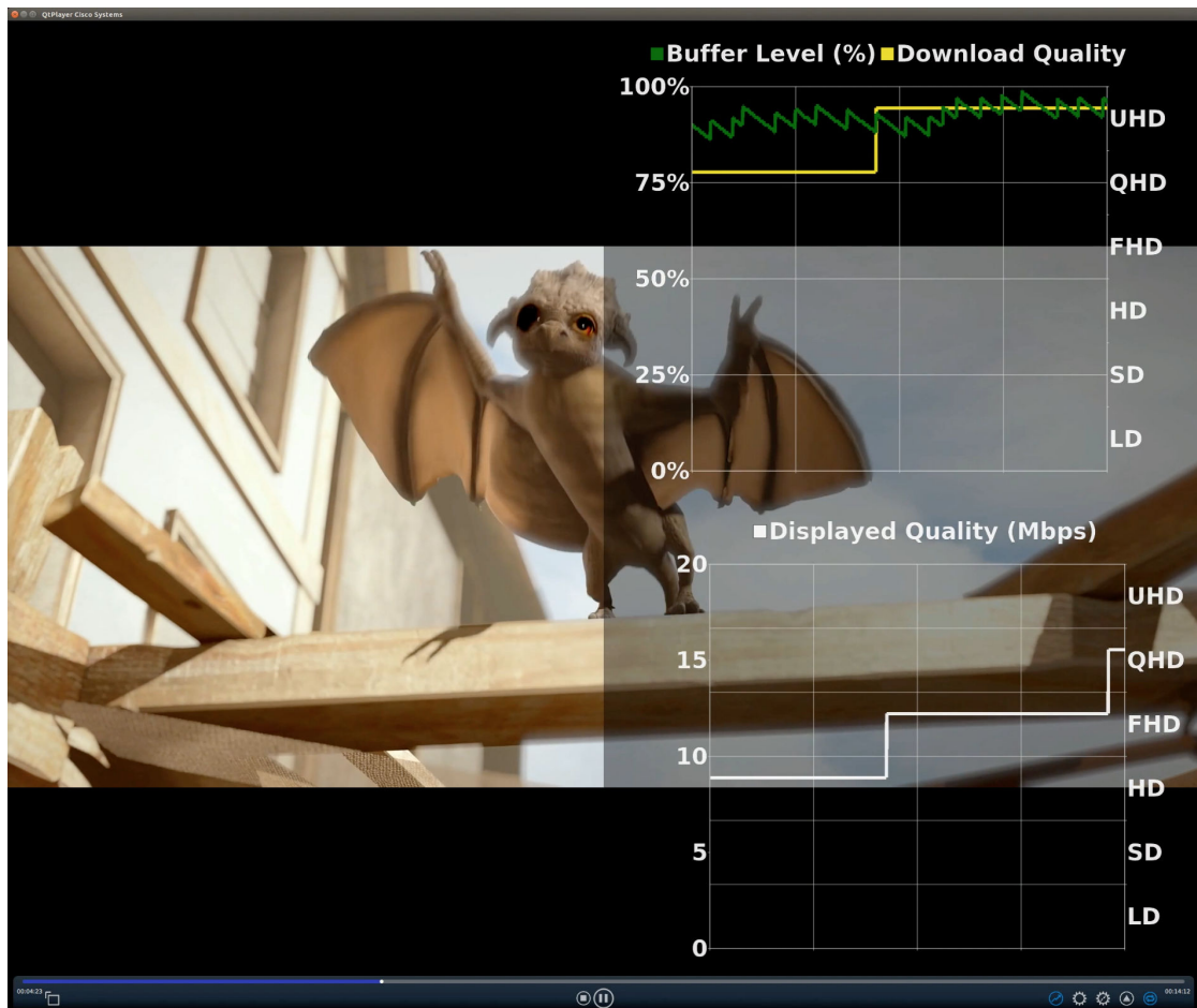
Figure B.1: Screenshot of Viper playing Sintel and displaying in real-time the buffer level, the quality at which current segments are downloaded and the video quality displayed.
