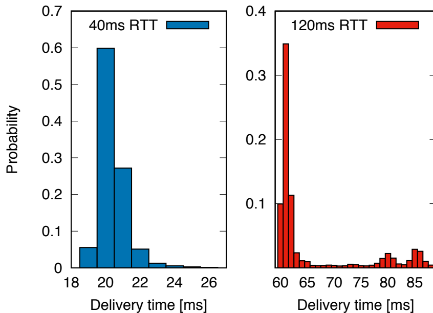
Figure 5.7: Distribution of the time elapsed between the production of an RTP packet and its reception at the consumer
