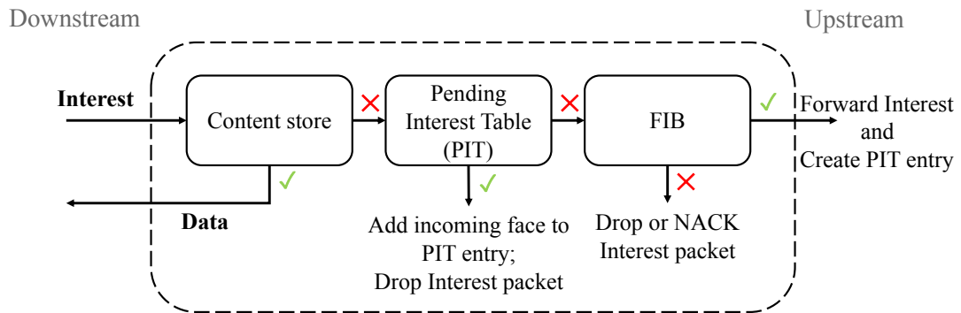
(a) Interest packet forwarding.
