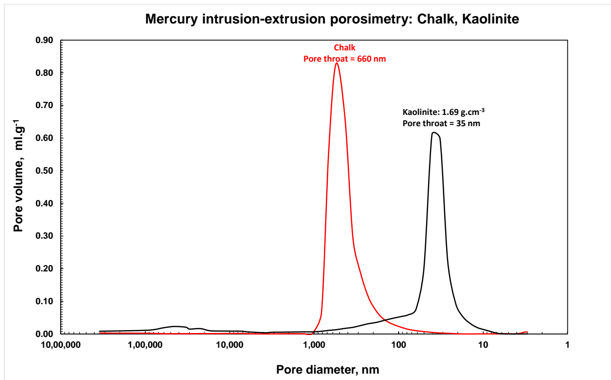
Figure S1: Pore-size distribution derived from mercury porosimetry for chalk and for compacted kaolinite
