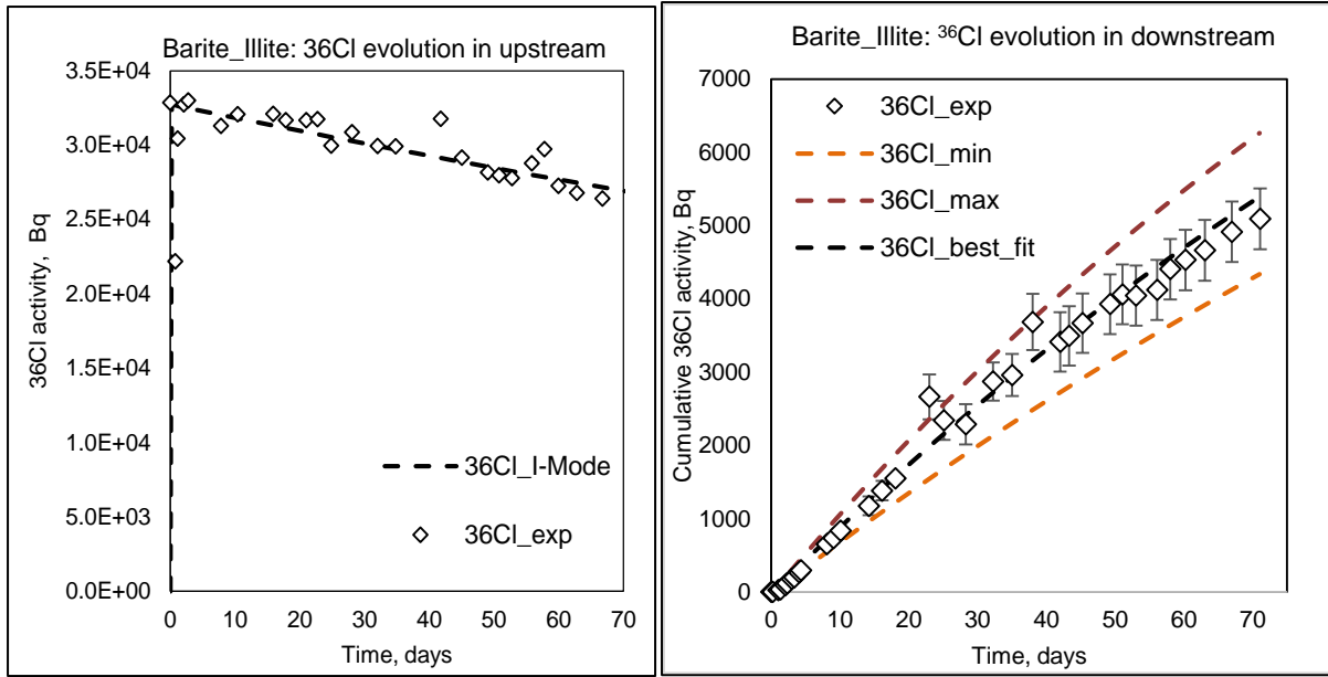
Figure 9: ^{36}\text{Cl} cumulative activity evolution in upstream and downstream after 70 days of barite precipitation experiment in ILL-B. The cumulative data of downstream are reproduced at minimum, best and maximum fits using I-Mode
