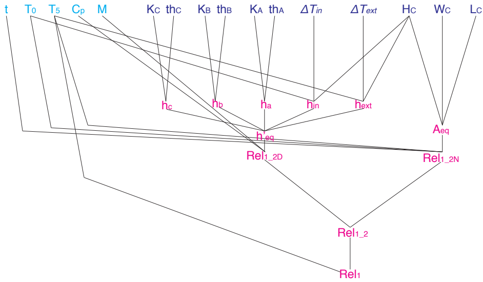
Figure A.14: Rel_1 tree
