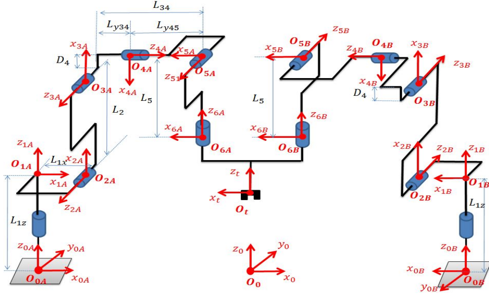
FIGURE 7.13 – The cooperative system
