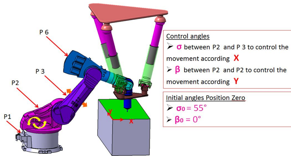
FIGURE 7.37 – Workspace of the hybrid structure
