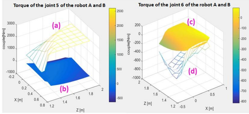
FIGURE 7.33 – Torque of the joints 5 and 6 of the robot A and B during welding, (a) : Torque of the joint 5 of the robot B, (b) : Torque of the joint 5 of the robot A, (c) : Torque of the joint 6 of the robot A, (d) : Torque of the joint 6 of the robot B
