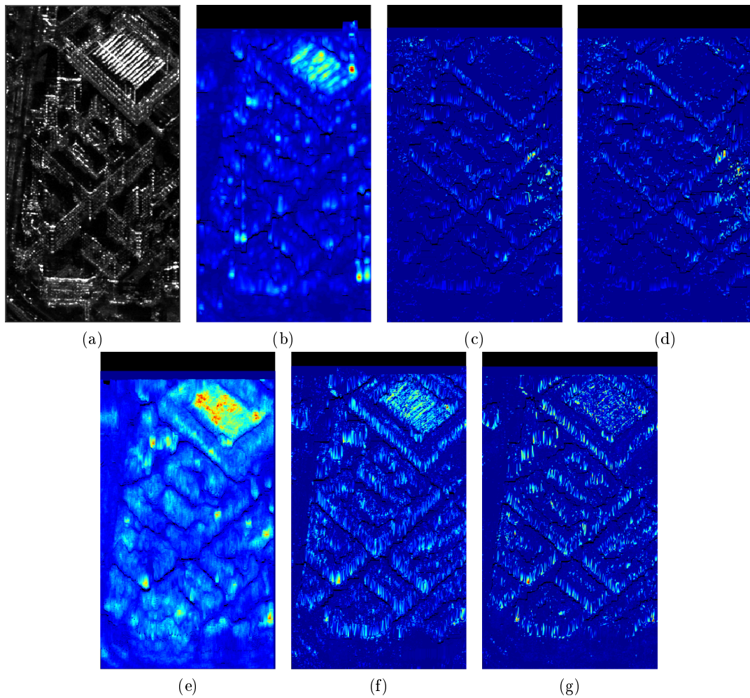
Figure 9.7 – Average amplitude SAR image (a), surface amplitude estimation using SPICE (b), MUSIC (c), WSF (d), Capon beamforming (e), the 3-D inversion (f) and REDRESS (g). For each results, the image shows the surface colored according to its amplitude.
