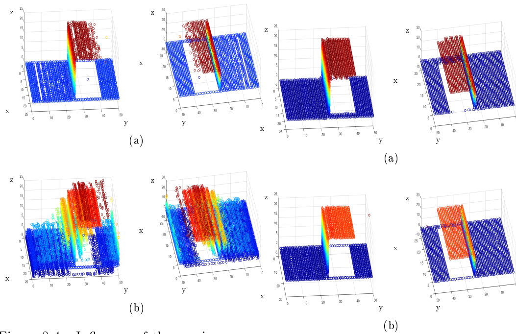
Figure 8.4 – Influence of the parsimony \mu_{l_1} parameter. In (a) the parameter is way above its optimal value resulting in a lot of holes in the structure. In (b) we use a small value of \mu_{l_1} resulting in a high number of outliers.
