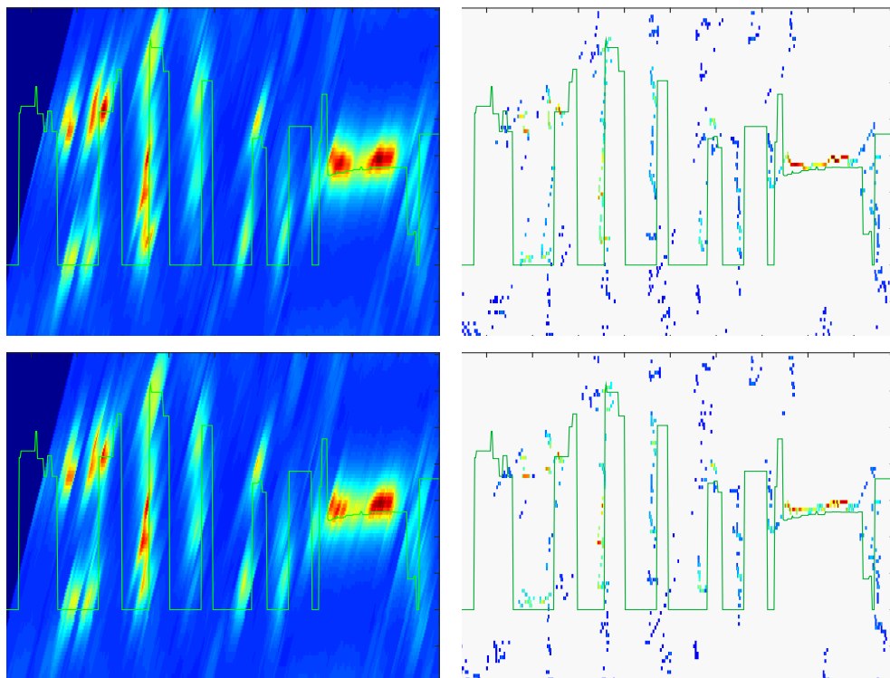
Figure 7.10 – Comparison of the tomographic reconstruction for one profile of consisting of dense buildings. The top row has been obtained using a gausscar kernel whereas the bottom one weighted the samples using the proposed similarity criterion. On the left the results correspond to the MUSIC-PS and on the right to the discrete MUSIC with 3 scatterers for each cell. The ground truth is shown in green.
