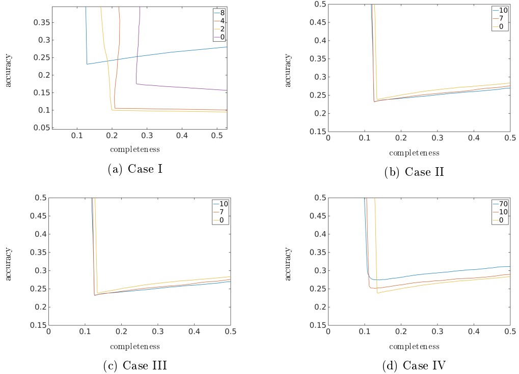
Figure 8.8 – Study of the influence of each parameter on the metrics for the Reg scene (cf. Fig. 6.1 (a)). The plots in (a), (b), (c) and (d) correspond respectively to different values of \mu_{\ell_1} , \mu_x , \mu_y and \mu_z with the three other parameters being fixed.
