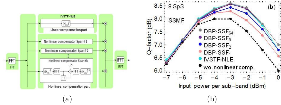
Figure 1.12: (a)Block diagram of IVSTF-NLEs equalizer; and (b) Q-factor vs. input power performance improvement obtained for 400 Gb/s without/with IVSTF-NLEs and DBP-SSFM 1,2,8,64 in SSMF (after [59]).
