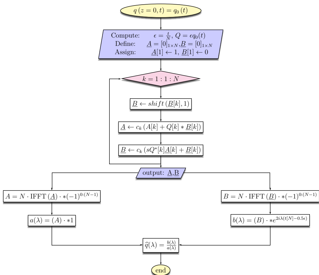
Figure 2.7: Flow chart of NFT algorithm implementation (after [75]).
