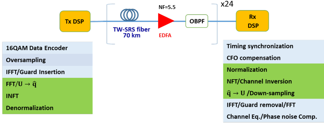
Figure 4.1: Simulation setup.
