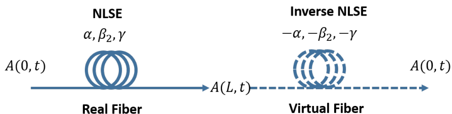
Figure 1.11: Illustration of forward propagation in real fiber governed by NLSE and digital backward propagation (DBP) through virtual fiber using the inverse NLSE.
