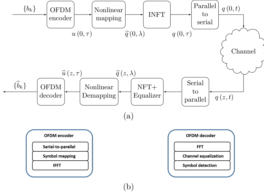
Figure 2.10: The architecture of NFDN transmission system (a) and (b) the corresponding DSP.
