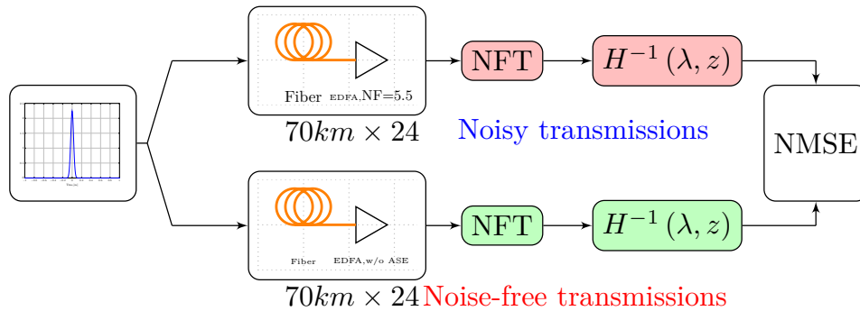
Figure 4.2: The numerical study schematic diagram of a noiseless and noisy evolution of the continuous spectrum over fiber channel.
