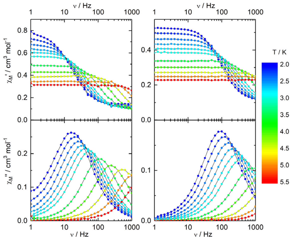
Figure 6: Frequency dependences of the in-phase (top) and out-of-phase (bottom) components of the magnetic susceptibility of 1 (left) and 2 (right) measured under a 600 Oe field for 1 and 800 Oe field for 2 ; the temperature is varying from 2 K to 5.5 K.
