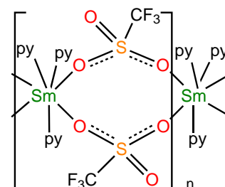
1.4py
