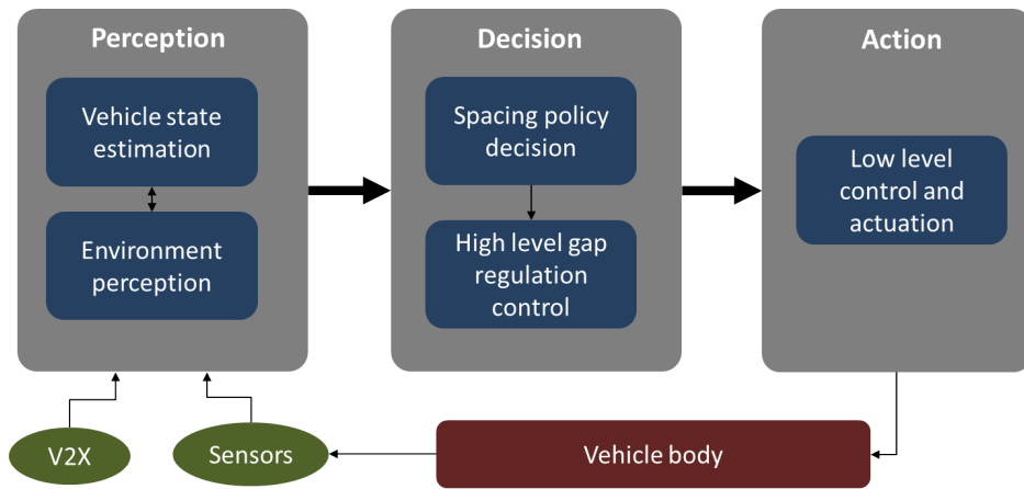
Figure 2.6: General architecture of a cooperative automated vehicle
