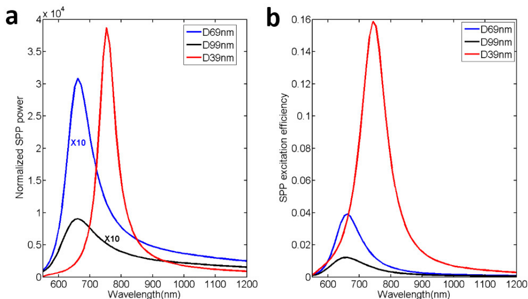
Figure 3.13. (a) Normalized SPP power with 3 different bottom diameters of nanocone; (b) Related SPP excitation efficiency spectra.
