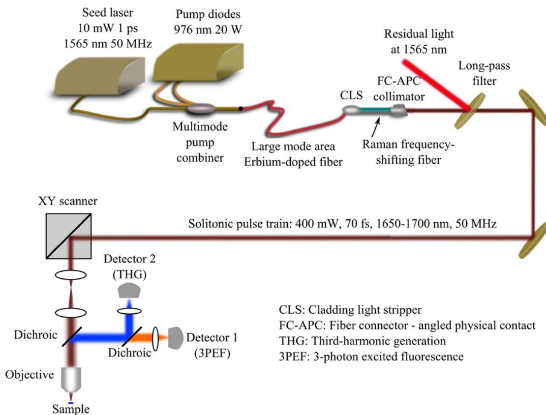
FIGURE 4.6. Experimental setup for 3P microscopy at 1700 nm with a fiber-based laser scheme. Chirped pulses from the seed laser at 1565 nm are amplified directly in a diode-pumped large mode area Er-doped fiber and frequency-shifted in a second large-mode area fiber. A long-pass filter filters out residual light at wavelengths below 1600 nm prior to the three-photon microscope.
