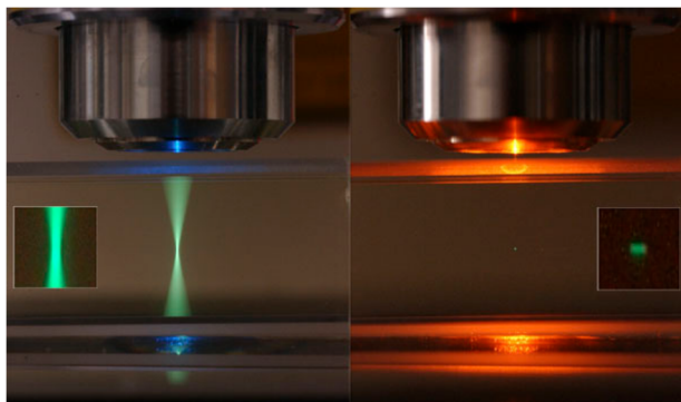
FIGURE 1.4. Optical section in multiphoton microscopy. Left: fluorescein solution excited at 488 nm with a continuous laser. Right: Same solution excited through a 2PEF process with a pulsed laser in the near IR range. Credit: Steve Ruzin and Holly Aron, UC Berkeley.
