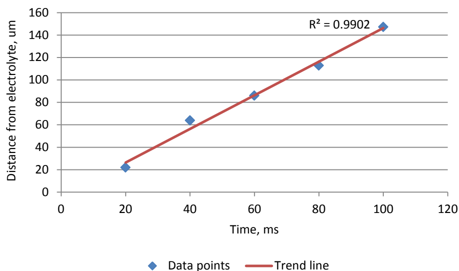
Figure 6.8 – Temporal evolution of the redox front drift length
