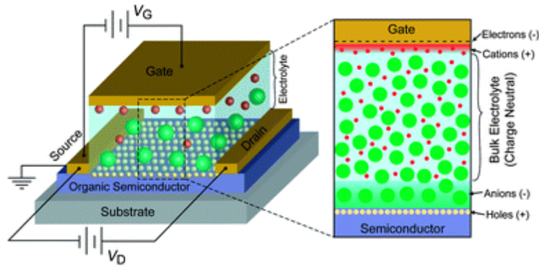
Figure 3.4 – Electrolyte Gated Field Effect Transistor structure[93]
