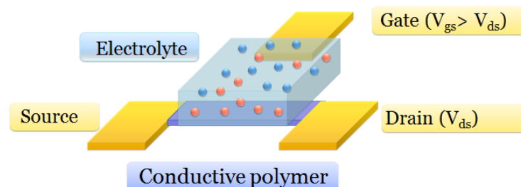
Figure 1.5 – Structure of typical OEET
