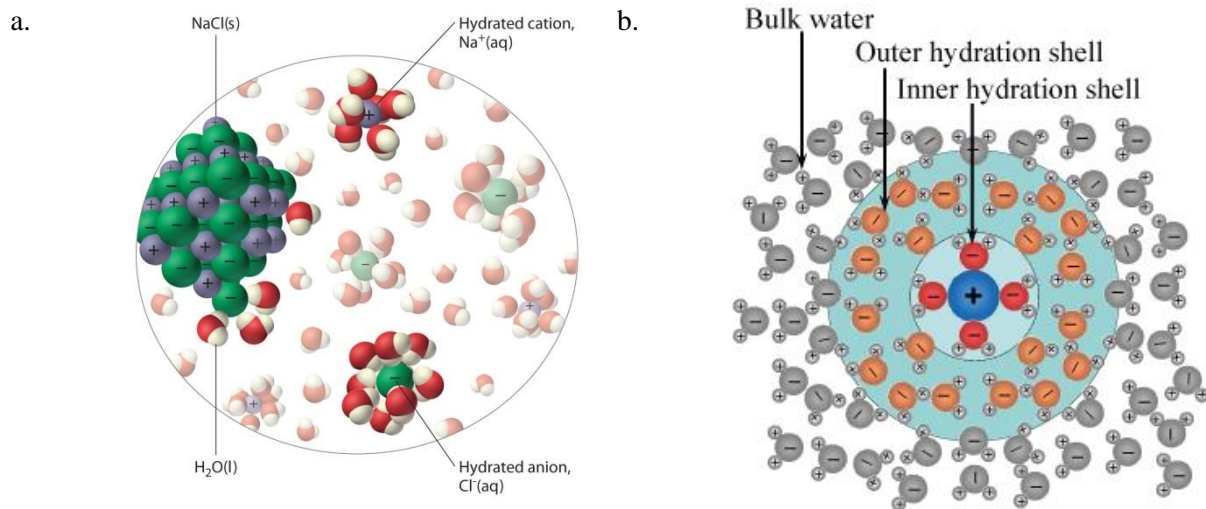
Figure 2.1 – Solvation process in aqueous electrolyte solution: a) Water molecule interaction with NaCl salt crystal; b) Formation of surrounding hydration shells [54]
