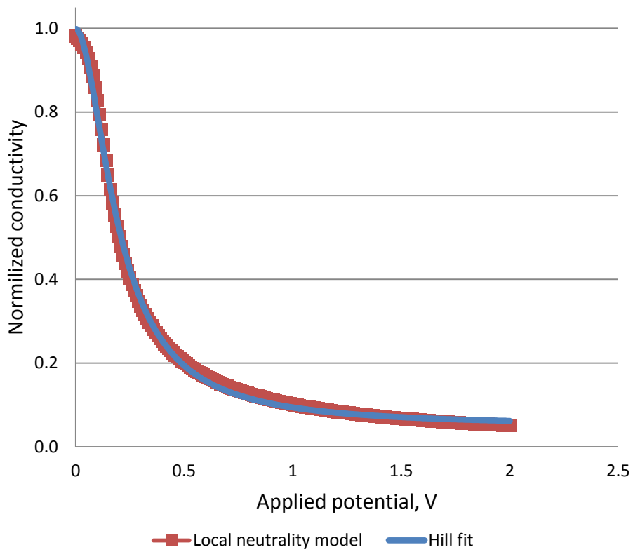
Figure 3.19 – Numerically calculated (red squared) and fitted using Hill function (blue curve) normalized conductivity dependence from applied potential obtained for: a.) Global neutrality model; b.) Local neutrality model
