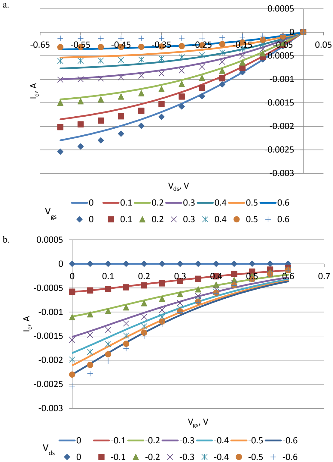
Figure 5.10 – Drain current dependence on applied potential. Continuous line – calculated curve; markers – experimental data points. a) Output curve (Drain current dependent on applied Drain-Source potential for different Gate-Source potentials); b) Transfer curve (Drain current dependent on applied Gate-Source potential for different Drain-Source potentials);
