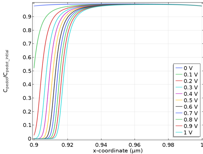
Figure 3.6 – Steady state EGOFET-like model positive species normalized \text{PEDOT}^+ concentration profile inside PEDOT:PSS layer at different applied Gate-Source potentials (from 0 to 1 V)
