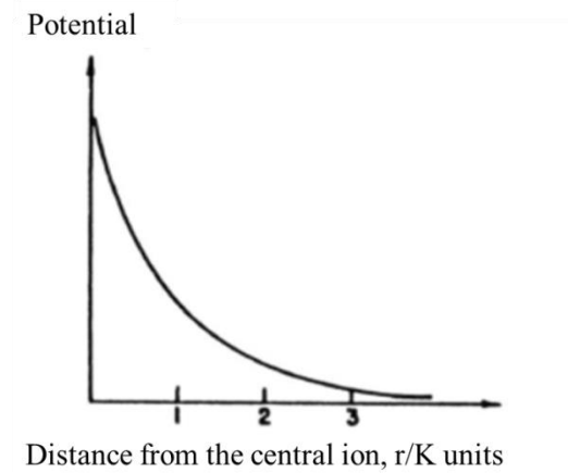
Figure 2.3 – Analytic solution of linearized Poisson-Boltzmann equation. Electric potential dependence from the distance from atom[53]
