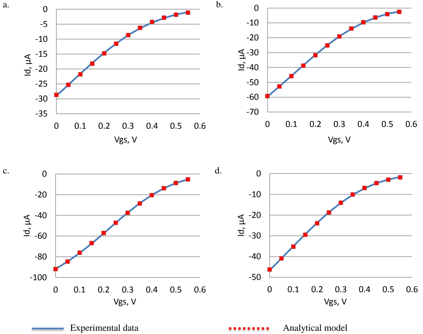
Figure 4.1 – Experimental data and analytical model fit for transistors with different channel dimensions: a) width: 5 \mu m ; length: 100 \mu m ; thickness: 0.03 \mu m ; b) width: 10 \mu m ; length: 50 \mu m ; thickness: 0.026 \mu m ; c) width: 10 \mu m ; length: 25 \mu m ; thickness: 0.018 \mu m ; d) width: 25 \mu m ; length: 250 \mu m ; thickness: 0.016 \mu m
