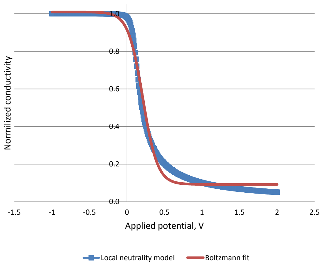
Figure 3.18 – Numerically calculated (blue squared) and fitted using Boltzmann function (red curve) normalized conductivity dependence from applied potential obtained for: a.) Global neutrality model; b.) Local neutrality model
