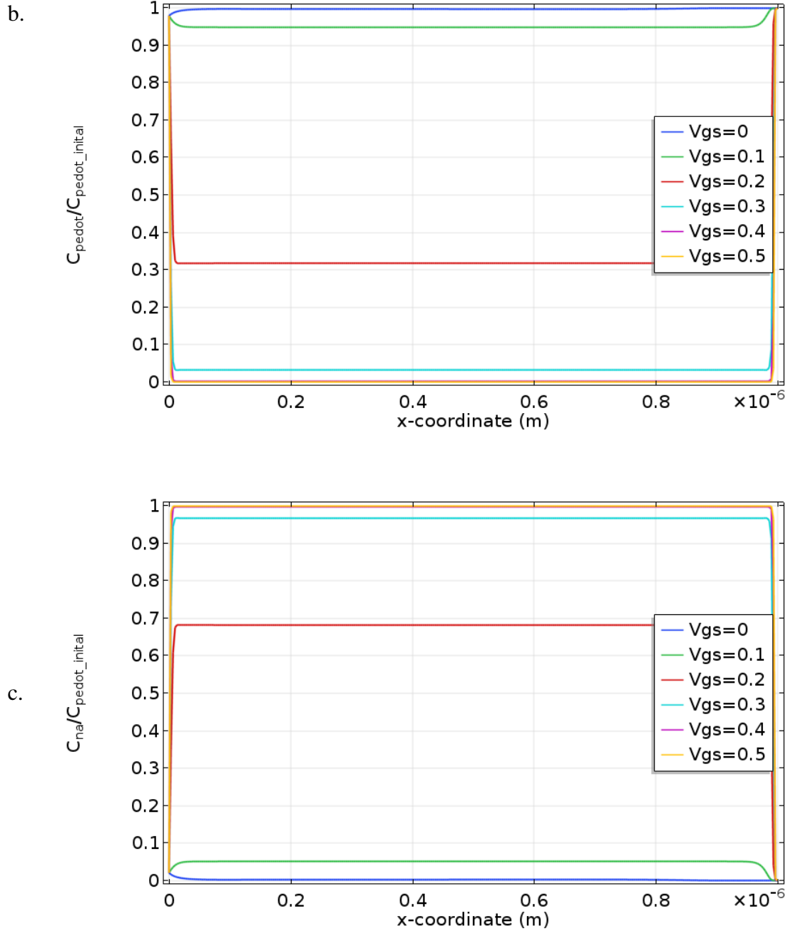
Figure 3.17 – Potential and concentration distribution in the channel at different applied at V_{gs} (in volts) and V_{ds} = -0.5 V. Cut line is parallel to x-axis, cuts PEDOT:PSS layer in the middle: a) Potential profile inside PEDOT:PSS; b) PEDOT + normalized concentration profile; c) Na + normalized concentration profile
