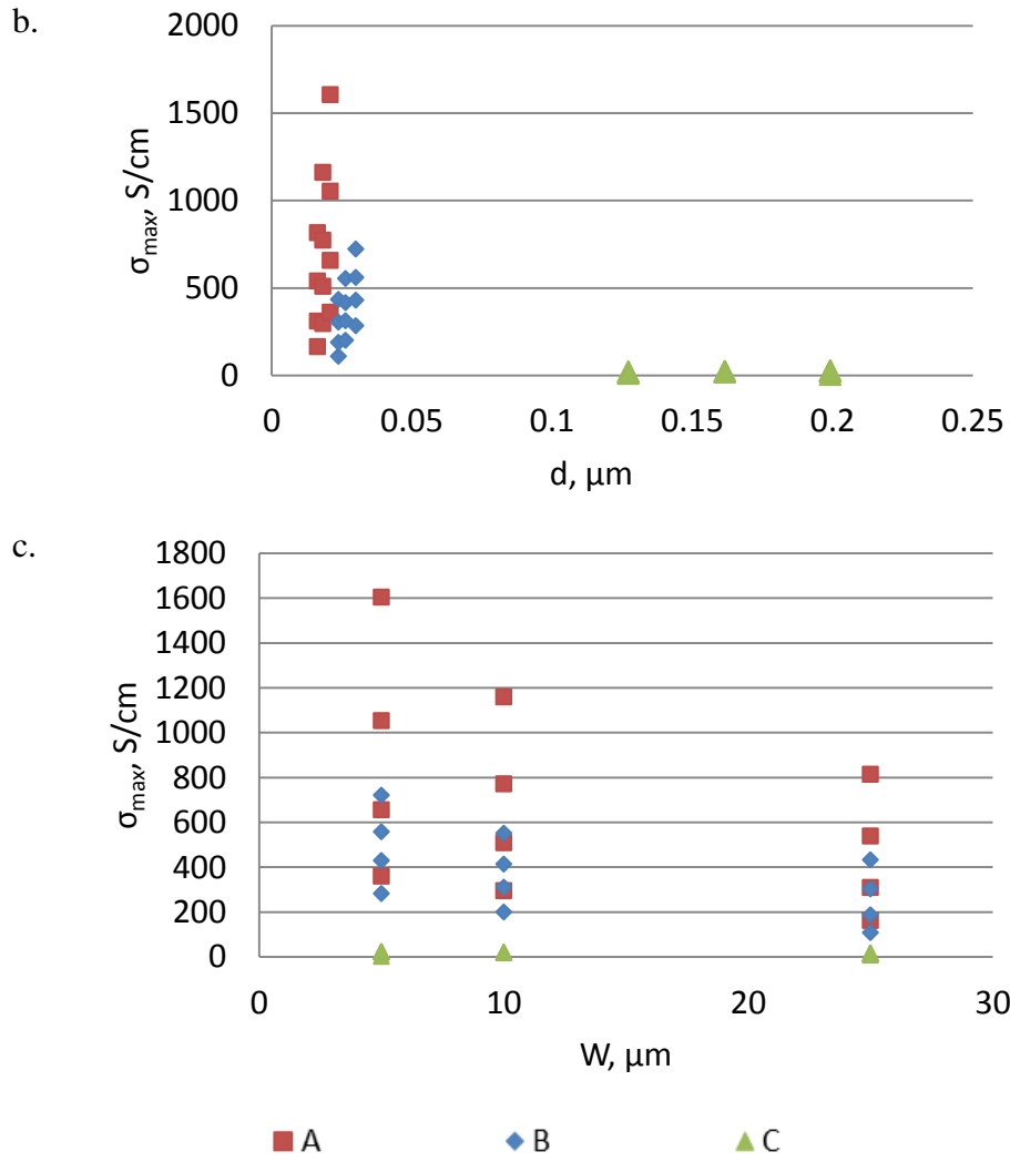
Figure 4.4 – Maximum conductivity correlation with: a) Channel length; b) Channel thickness; c) Channel width; A: Thin channel transistors ( d=16\div20 nm); B: Medium channel transistors ( d=24\div30 nm); C: Thick channel transistors ( d=127\div200 nm)
