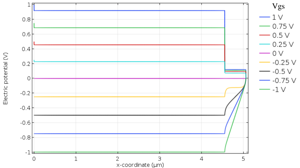
Figure 5.5 – Global Neutrality numerically modelled potential profiles along the whole device. (electrolyte and conductive polymer layers) Curves were modelled for different applied Gate-Source potentials (from -1 to 1 V)
