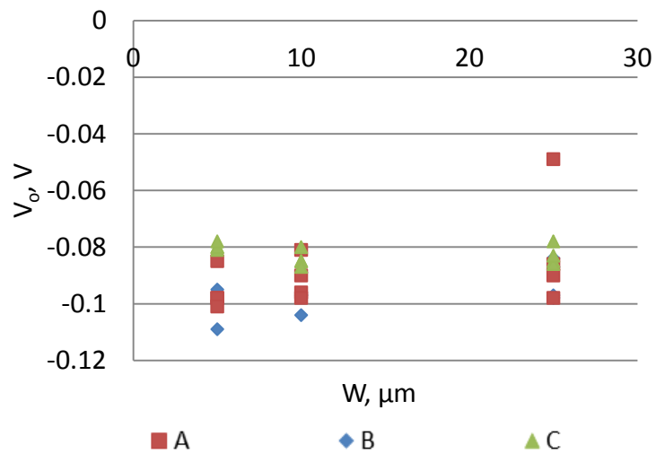
Figure 4.6 – V_0 correlation with: a) Channel length; b) Channel thickness; c) Channel width; A: Thin channel transistors ( d=16\div20 nm); B: Medium channel transistors ( d=24\div30 nm); C: Thick channel transistors ( d=127\div200 nm)
