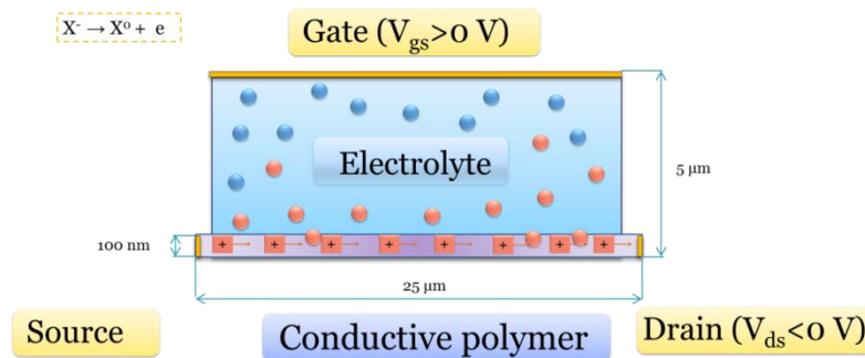
Figure 1.6 – Schematic representation of dedoping process in OEET
