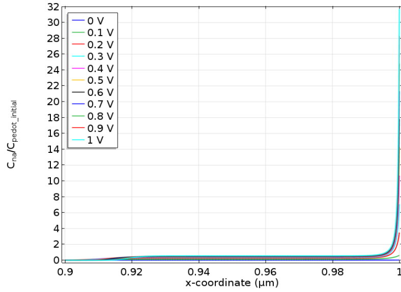
Figure 3.10 – Steady state Global electroneutrality model positive species normalized concentration profile inside PEDOT:PSS layer at different applied Gate-Source potentials (from 0 to 1 V): a) PEDOT + concentration profile; b) Na + concentration profile
