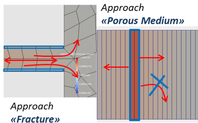
Figure 2-5 Differences between “Fracture” and “Porous Medium” modeling approaches
