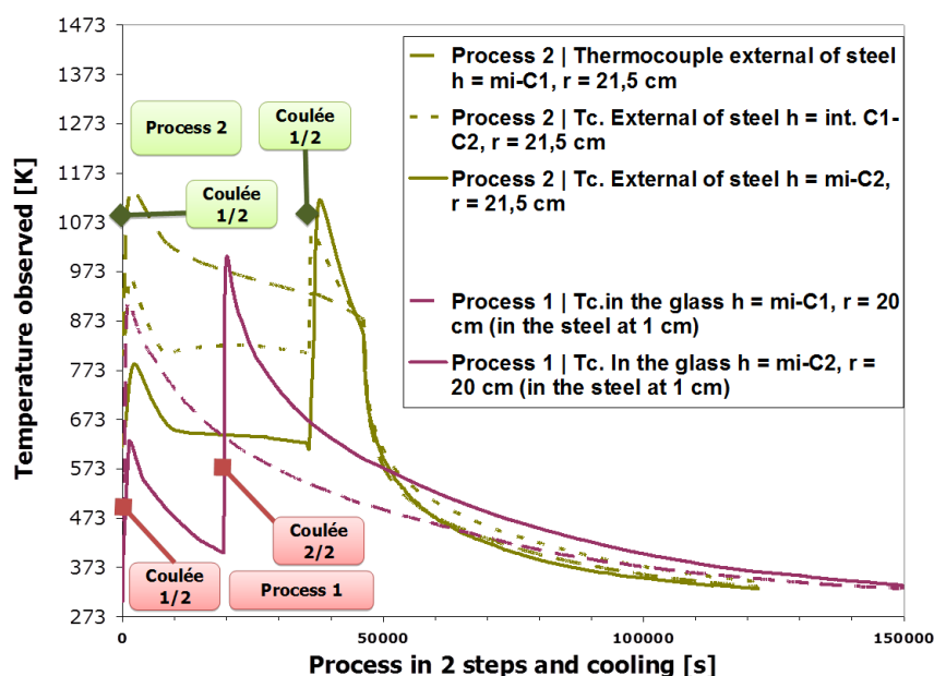
Figure 1-3 External temperature readings (close to steel) of the hot (process 2), and the cold (process 1) crucibles. For both of them the casting is effectuated in two steps, with total mass of a block being 400 kg). Adopted from (Barth 2013).
