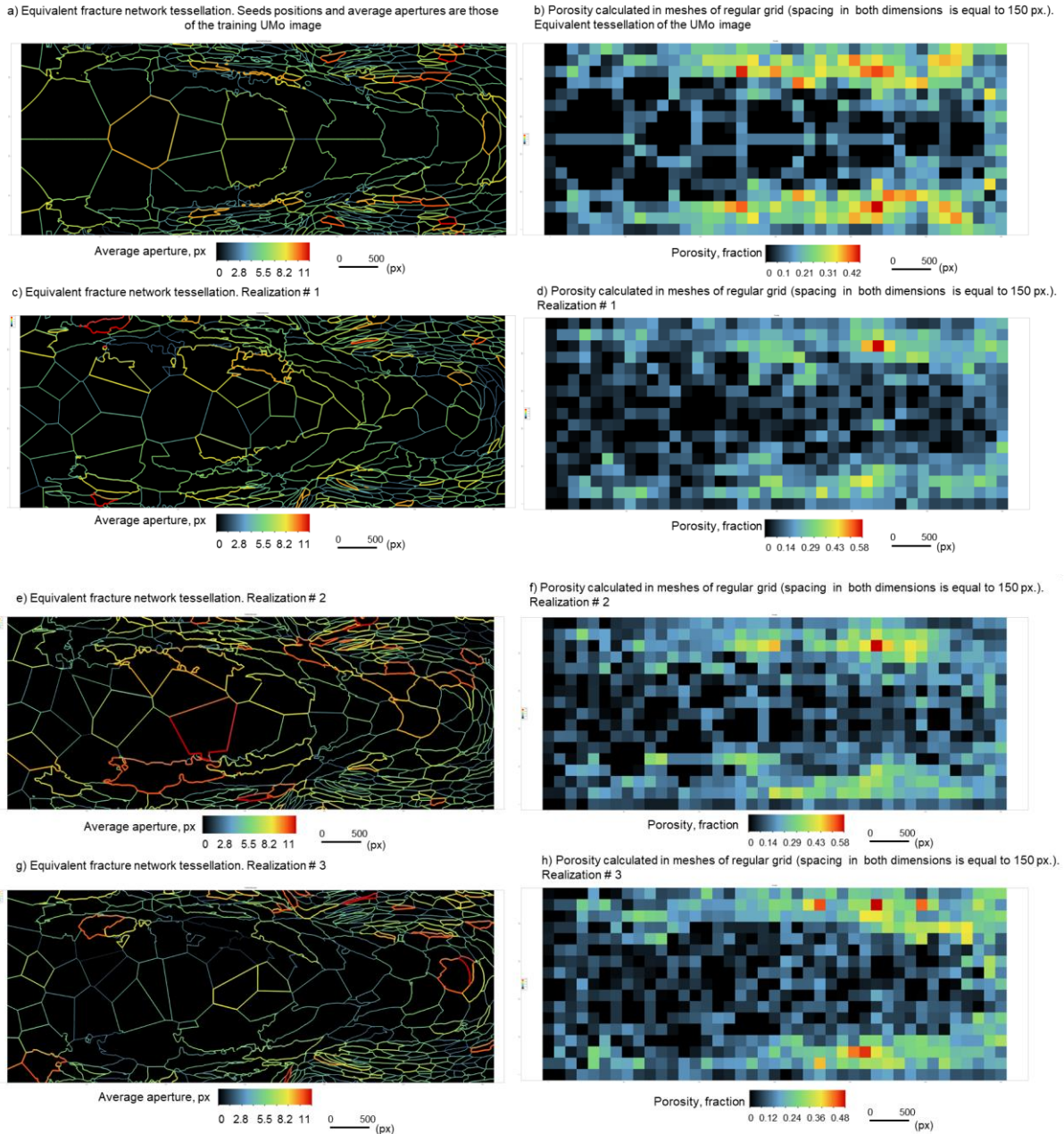
Figure 21 Equivalent fracture network by Voronoi anisotropic tessellation. Left columns including a), c), e), and g): equivalent fracture network tessellation (dimensions are 6145 px × 2430 px with 1 px corresponding to 0.17 mm. Right columns including b), d), f), and h): porosity (defined as the ratio of the surface occupied by fractures to the sum of the surfaces of the glass matrix and the fracture network) calculated for meshes of the 41 × 17 simulation grid.
