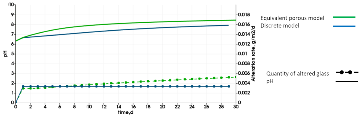
Figure 14 Results of the reactive transport modeling in the case where the impact of the pH and of the affinity term on the glass dissolution rate were not considered: quantity of altered glass obtained from boron concentration averaged over the water zones and evolution of the solution pH.
