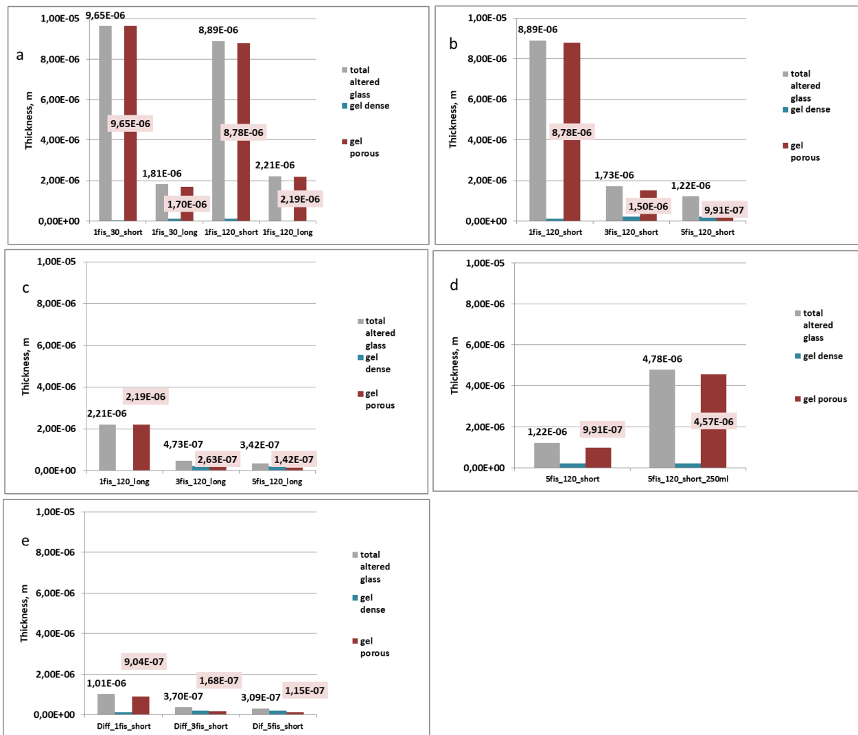
Figure 4-14 Bars charts resumming the results of the reactive transport modeling for the studied cases represented in Table 4-2.
