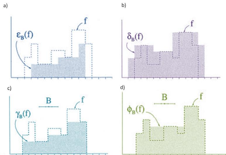
Figure 3-1 Result of morphological a) erosion \varepsilon_B(f) , b) dilation \delta_B(f) , c) opening \gamma_B(f) , d) closing \phi_B(f) of the image f . Structuring element B used for the pairs dilation and closing, erosion and opening is the same. Obtained from (Soille, 2003)
