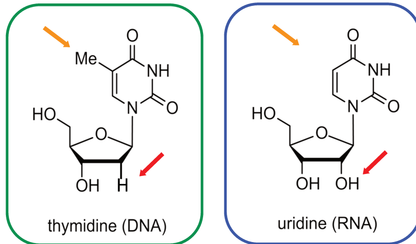
Figure I.3: Chemical structure differences between thymine and uracil bases and between 5 carbon sugars of DNA and RNA molecules. Thymine and uracil differ by a methyl group, which is present in thymine and absent in uracil (orange arrows). The OH group at the second position of the RNA 5 carbon sugar is replaced by a hydrogen atom in DNA (red arrows).
