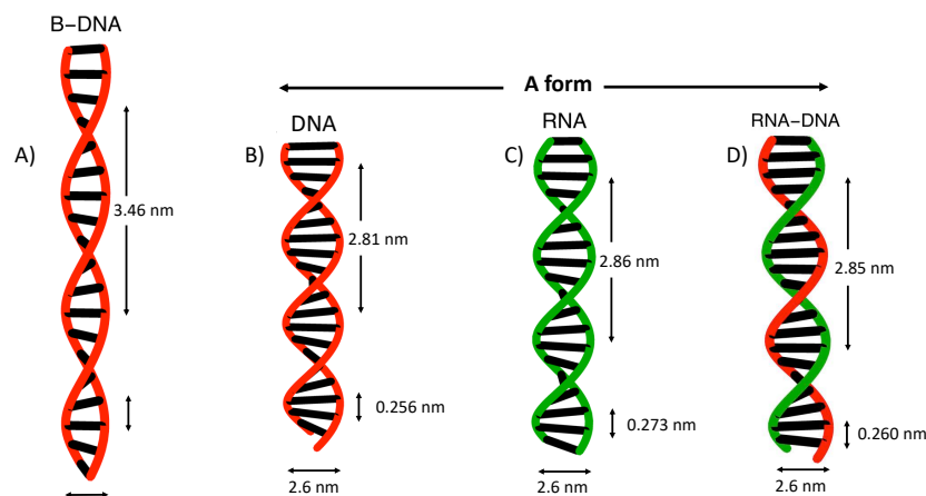
Figure I.4: Physical structures of dsDNA, dsRNA, RNA-DNA hybrid and differences of A and B form helices. In double stranded configuration all three molecules exhibit helical structure. Depending on external conditions dsDNA adopts A or B form, whereas dsRNA and RNA-DNA adopt only A form. Both A and B form helices are right handed. Compared to B form, helices in A form are shorter and wider. A) B-DNA has 2nm diameter and a distance of 0.346nm between two consecutive base pairs. One helical turn is 3.46nm corresponding thus to 10 base pairs. B) A-DNA has a diameter of 2.6nm and a distance between two consecutive base pairs is 0.256nm. One helical turn is 2.81nm corresponding thus to 11bp. C) A-RNA double helix has 2.6nm diameter and 0.273nm distance between two consecutive base pairs. One helical turn is 2.86nm corresponding thus to 10.5bp. D) RNA-DNA hybrid has 2.6nm diameter and 0.26nm distance between two consecutive base pairs. One helical turn is 2.85nm corresponding thus to 11bp.
