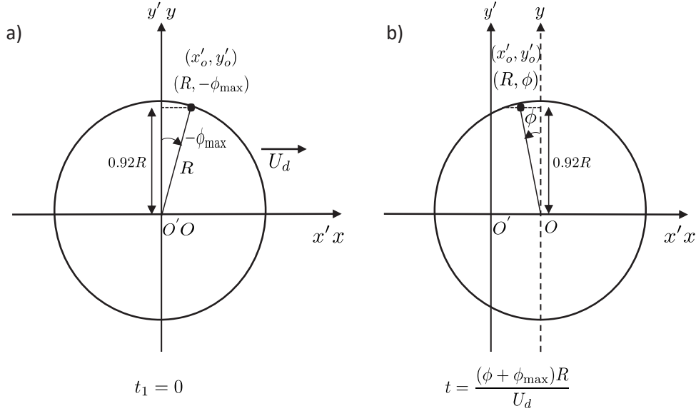
FIGURE 11. Analogy with a soap film deposited along \theta rather than over time. (a) A film of thickness h_\infty(\phi_{\max}) = 1.337H_0Ca^{2/3}(\phi_{\max})^{2/3} is deposited at (R, -\phi_{\max}) = (R, -(\frac{\pi}{2} - \theta_{\max})) and (b) thins until the influence of the rear meniscus is felt.
