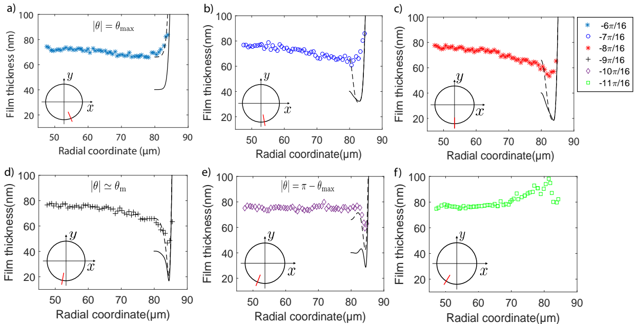
FIGURE 10. Radial profiles for (a) \theta = -\frac{6\pi}{16} , (b) \theta = -\frac{7\pi}{16} , (c) \theta = -\frac{8\pi}{16} (d) \theta = -\frac{9\pi}{16} , (e) \theta = -\frac{10\pi}{16} and (f) \theta = -\frac{11\pi}{16} for Ca = 7.2 \times 10^{-4} . Solid line: solution of (5.4) with the numerical profile h^{\text{num}}(\rho, \theta_{\max}) as initial condition, i.e. the solution of (5.3) for \theta = \theta_{\max} = \frac{\pi}{2} - \delta'_\theta \phi'_{\max} . Dashed line: solution of (5.4) using the experimental profile h^{\text{exp}}(\rho, \theta_{\max}) as an initial condition. Inset: the red line indicates the location of the radial profile for each angle value.
