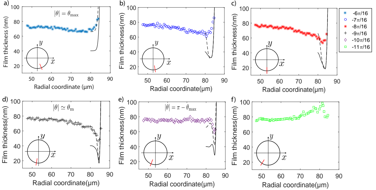
FIGURE 10. Radial profiles for (a) \theta = -\frac{6\pi}{16} , (b) \theta = -\frac{7\pi}{16} , (c) \theta = -\frac{8\pi}{16} , (d) \theta = -\frac{9\pi}{16} , (e) \theta = -\frac{10\pi}{16} and (f) \theta = -\frac{11\pi}{16} for Ca = 7.2 \times 10^{-4} . Solid line: solution of (5.4) with the numerical profile h^{\text{num}}(\rho, \theta_{\max}) as initial condition, i.e. the solution of (5.3) for \theta = \theta_{\max} = \frac{\pi}{2} - \delta'_\theta \phi'_{\max} . Dashed line: solution of (5.4) using the experimental profile h^{\text{exp}}(\rho, \theta_{\max}) as an initial condition. Inset: the red line indicates the location of the radial profile for each angle value.
