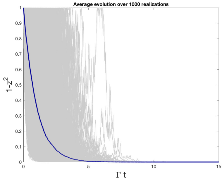
(b) Exponential decay of the qubit system (4.3) towards the set \{\Pi_{Z+1}, \Pi_{Z-1}\} , in terms of the Lyapunov function V(\rho) = 1 - \text{Tr}(\rho\mathbf{Z})^2 . The ensemble average depicted in blue, decays with rate 1, in agreement with Proposition 4.2.1.
