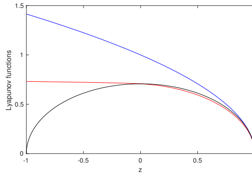
(a) In black: open-loop Lyapunov function (3.3). In blue, closed-loop function (4.6). In red: proposed function (4.11) with \alpha = 0.1 .
