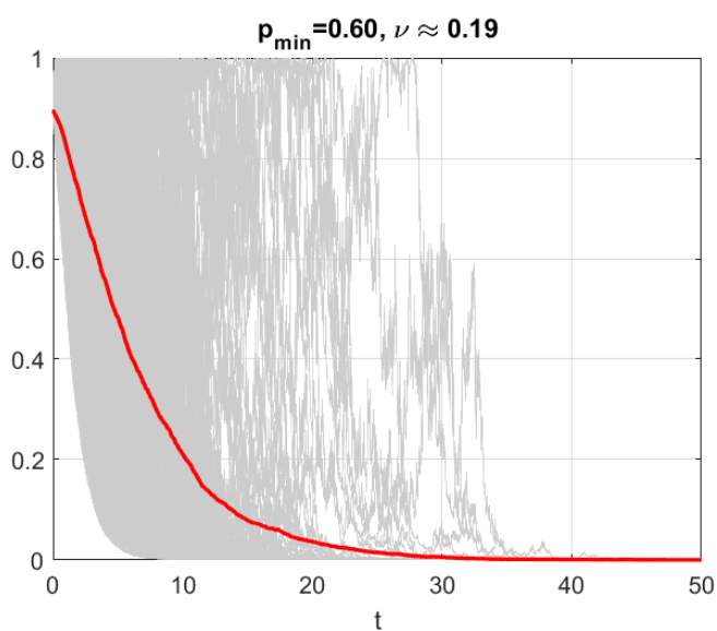
Figure 5.2: Ideal closed-loop simulations with p_{\min} = 0.6 . In gray: selection of 200 individual trajectories t \mapsto \sqrt{1 - \text{Tr}(\Pi_\ell \rho_t)} ; In red: average over 1000 realizations.
