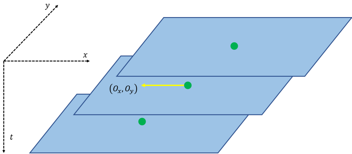
Figure 5.14 – The shape of the patch is a parallelepiped with skew in x and y directions controlled by its optical flow vector.
