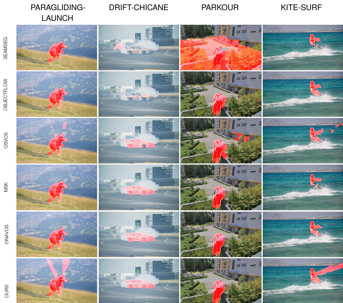
Figure 3.29 – Visual comparison of different single objects video segmentation approaches on DAVIS-2016 dataset. From top to bottom: SeamSeg (Ramakanth and Babu 2014), ObjectFlow (Tsai, M.-H. Yang, and Black 2016), OSVOS (S. Caelles et al. 2017), MSK (F. Perazzi, J. Pont-Tuset, et al. 2016), onAVOS (Voigtlaender and Leibe 2017), ours.
