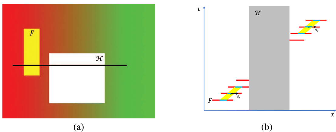
Figure 5.15 – (a) A synthetic video where the foreground (yellow rectangle) crosses the occlusion. (b) x - t profile along the black line slice.
