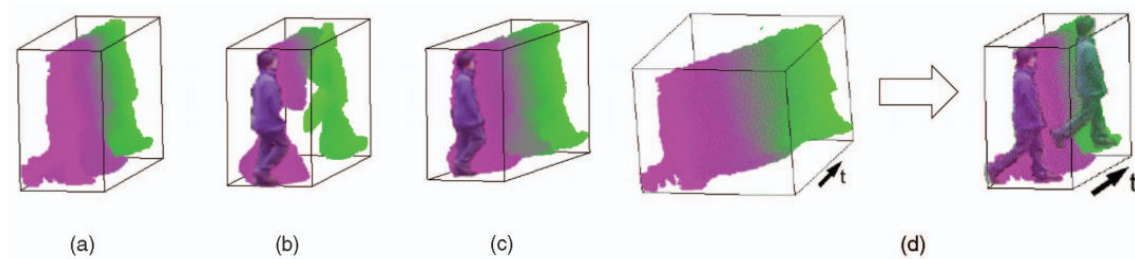
Figure 5.10 – (Jia, Tai, et al. 2006) perform video inpainting by repairing cyclic motions. (a) Sample model, (b) damaged model, (c) repaired model, (d) sample model after wrapping and stabilization. Image taken from (Jia, Tai, et al. 2006).
