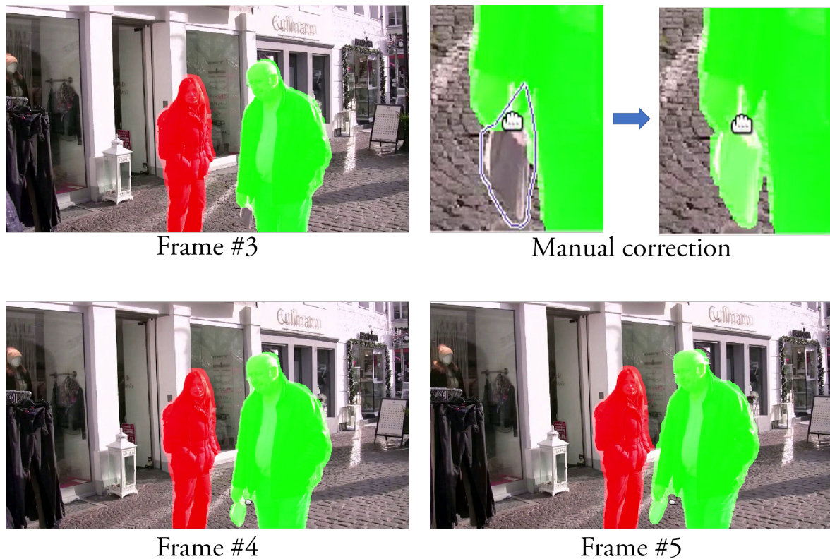
Figure 6.3 – If the users are not satisfied with the segmentation result, they can correct the error manually at one frame and the algorithm will propagation this modification to the next frames.
