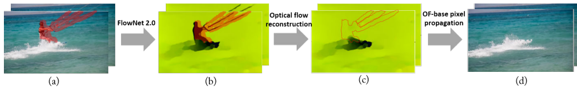
Figure 4.6 – The global pipeline of the optical flow-based propagation approach for reconstructing a static background: From input video (a), forward/backward optical flow fields are estimated by FlowNetv2 (Ilg et al. 2017) (b), they are inpainted by an image inpainting algorithm (c). From these optical flow fields, pixels from the source region are propagated into the missing region (d).
