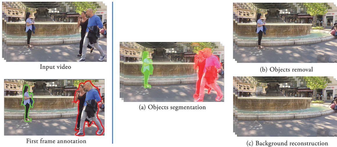
Figure 6.1 – We introduce a complete system for segmenting and removing objects in videos. Given a video and hand-drawn approximate outlines (in one frame) of objects chosen by the user, the system computes accurate segmentation masks of these objects in the whole video (Figure (a)) and then removes all or some of them according to user’s choices. Figures (b) and (c) show the results of removing one particular object (characters in red), or of removing all objects, respectively.
