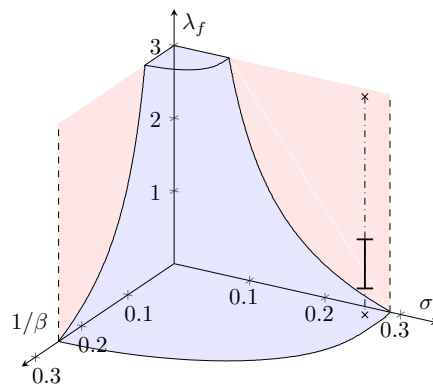
Figure J.1: Phase diagram for uniform distribution
