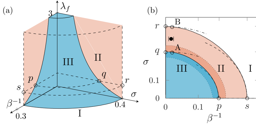
Figure 14.3: (a) Configuration of phases I, II and III in the parameter space (1/\beta, \sigma, \lambda_f) . (b) A section of this phase diagram corresponding to \lambda_f = 0.54 \pm 0.2 ; the shadowed region near the boundary II/III reflects the uncertainty in \lambda_f . The realistic data set for skeletal muscles is presented in (b) by a filled circle with the superimposed error bars indicating uncertainty in temperature. Analytic approximations in (b): dashed-dotted lines – low temperature; dashed lines – low disorder.
