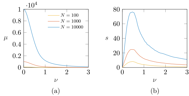
Figure 10.5: (a) Mean number of shocks; (b) Standard deviation of the number of shocks. The statistics consists of 1000 realizations of the quenched disorder (Weibull distribution \rho = 3 ) of several system sizes.
