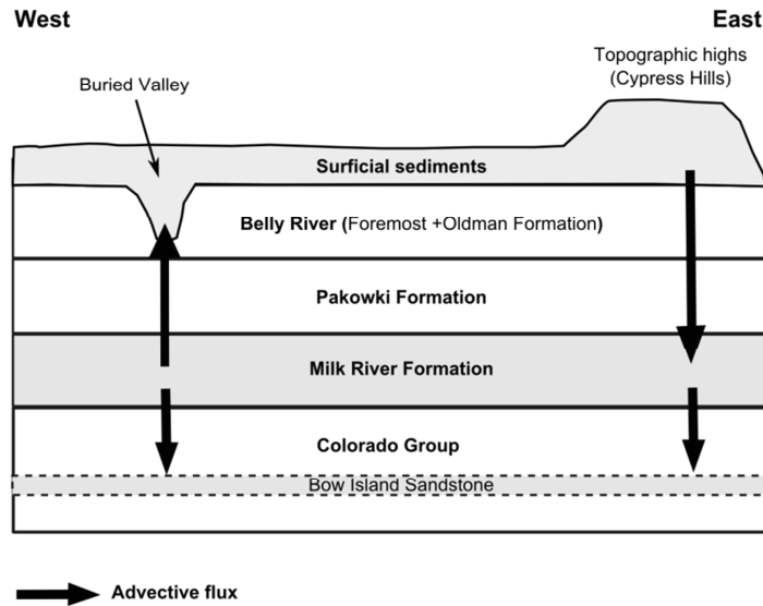
Figure 6.8 Vertical hydraulic gradients in southern Alberta between a overlying surficial sediments and the MRA and b the MRA and the underlying Bow Island Sandstone. Negatives values reflect upward flow. c Vertical flow tendencies schematically represented in the diagram (not to scale)
