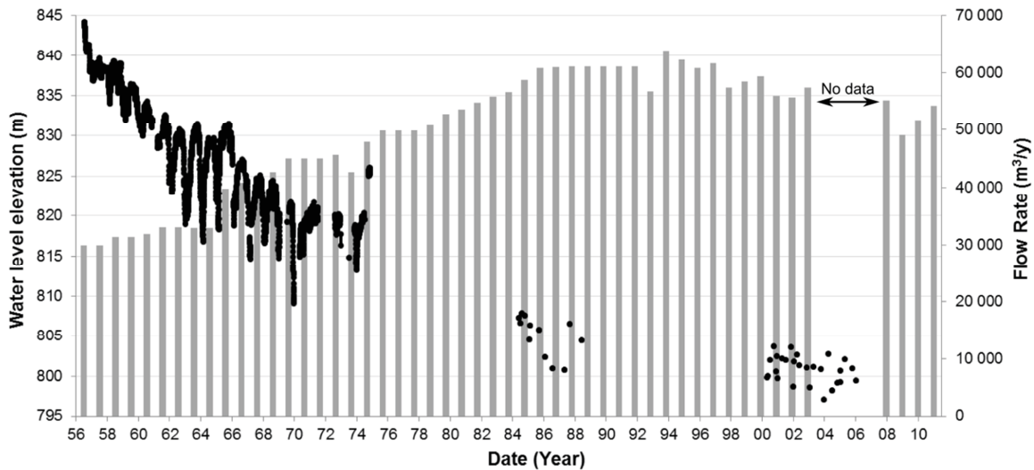
Figure 6.4 Water level of the Foremost observation well (AENV Id #221) (black dots) and annual groundwater diversion (gray bars) for the village of Foremost (HCL consultants 2004; Alberta Environment and Parks 2015)
