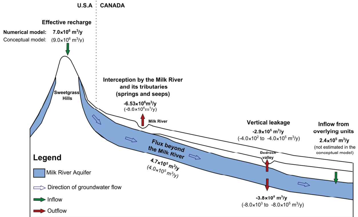
Figure 7.12 Comparison between the groundwater budget components from the conceptual model (Pétre et al. 2016) and the numerical model
