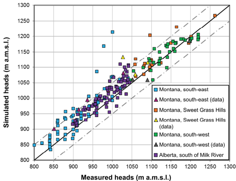
Figure 7.8 Plot of simulated versus measured heads in the Milk River aquifer, for the calibration zones. The calibration target interval ( \pm 50\text{m} ) is also shown (grey dashed lines). The calibration targets derived from monitoring wells are indicated as “data” in the legend. The measured heads in southern Alberta are from Toth and Corbet’s (1986) interpretation.
