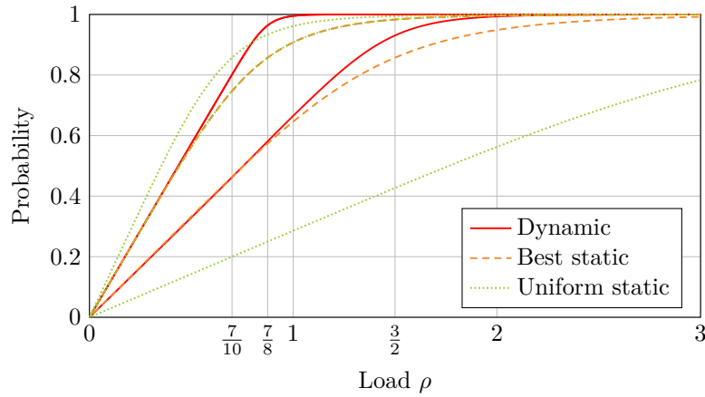
Figure 8.14: Activity probability of each computer in the cluster of Figure 8.11. Under the dynamic and best static schemes, the left and central computers—top curve—have the same activity probability, while the right computers—bottom curve—are active with a lower probability. Under the uniform static scheme, the central computers—top curve—have the highest activity probability, followed by the left computers—middle curve—and the right computers—bottom curve.
