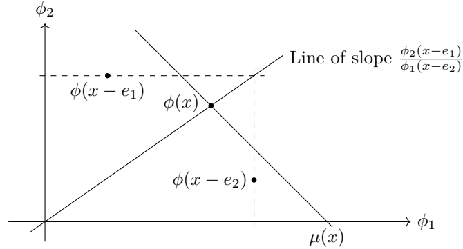
Figure 1.6: Recursive construction of the vector of service rates \phi(x) in the Whittle network of Figure 1.1. This vector is the point of intersection of the line of slope \phi_2(x - e_1)/\phi_1(x - e_2) and the line of equation \phi_1 + \phi_2 = \mu(x) . To generalize this approach in higher dimensions, we can work on each pair of queues separately.
