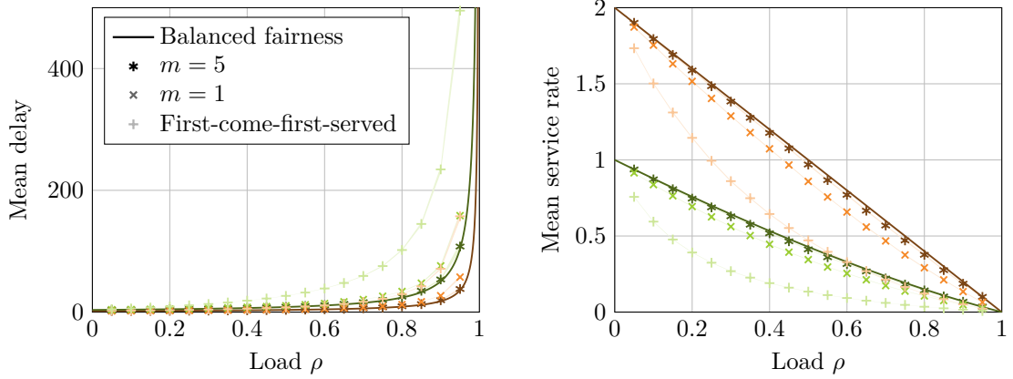
(c) Zipf number of exponentially distributed phases.
