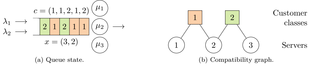
Figure 4.1: A multi-server queue with I = 2 customer classes and S = 3 servers.
