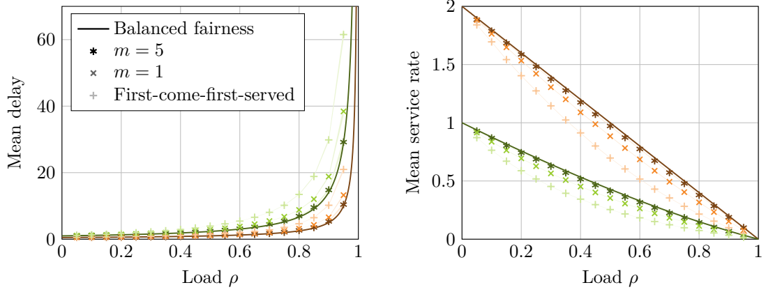
(a) Bimodal number of exponentially distributed phases.
