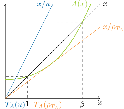
Figure C.1: Equation T_A(u) = u A(T_A(u)) .
