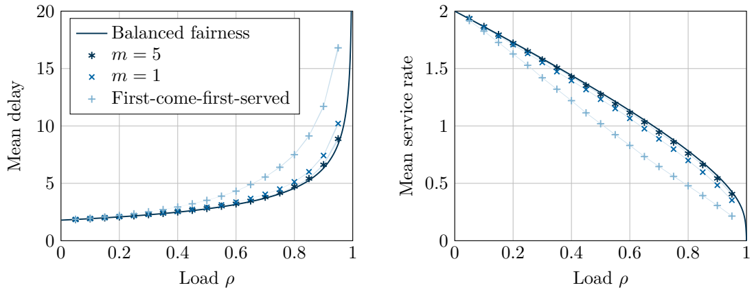
(c) Zipf number of exponentially distributed phases.
