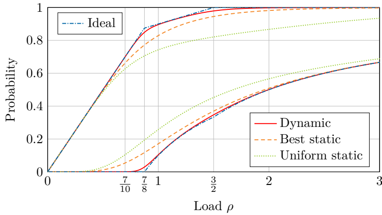
Figure 8.12: Average loss probability—bottom curve—and activity probability—top curve—in the cluster of Figure 8.11.
