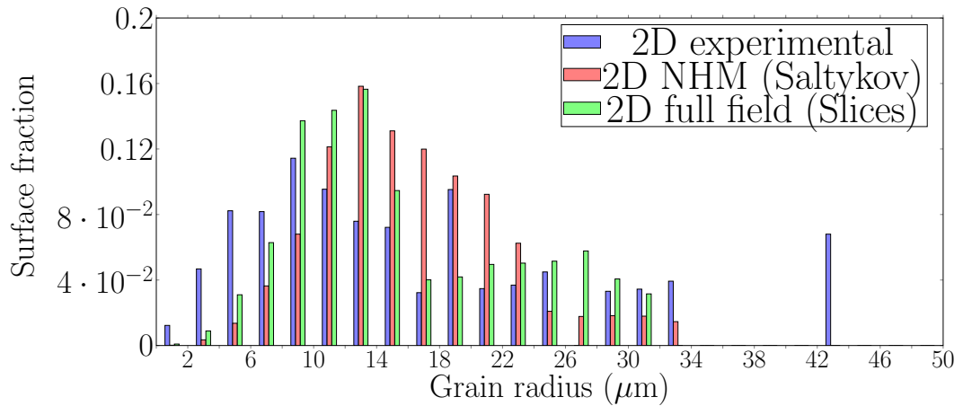
(c) T=1373\text{K} , \dot{\varepsilon}_{\text{VM}}=0.014\text{s}^{-1} , \varepsilon_{\text{VM}}=1.35 , X_{\text{expe}}=72.5\%
