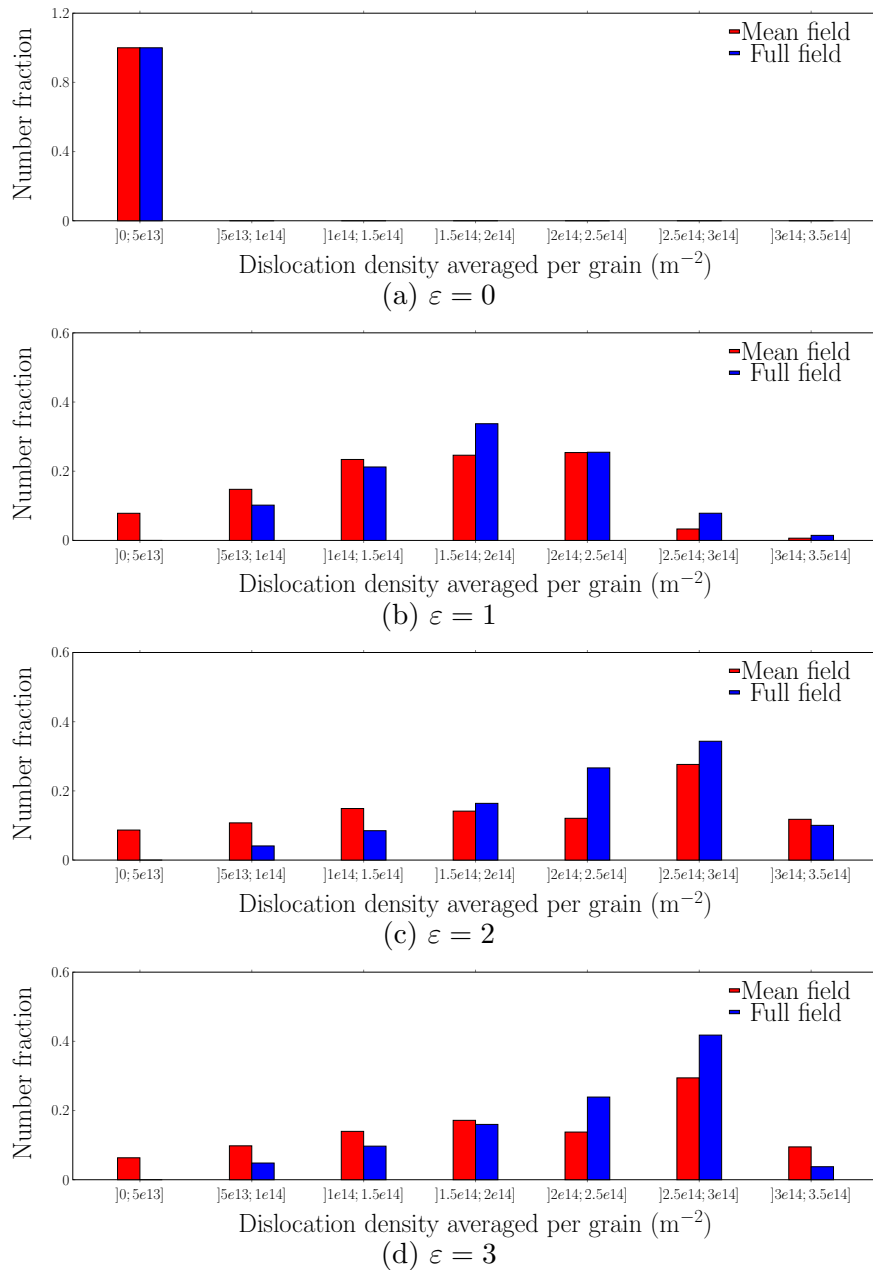
Fig. 3.15. Comparisons, at different instants, of the dislocation density distributions ((a) to (d)) obtained during a DRX process using the present full field model and the mean field model of Beltran et al. [50] introduced in first chapter. The simulated process is a channel-die compression at 1273K, at a strain rate of 0.01s^{-1} during 300s.
