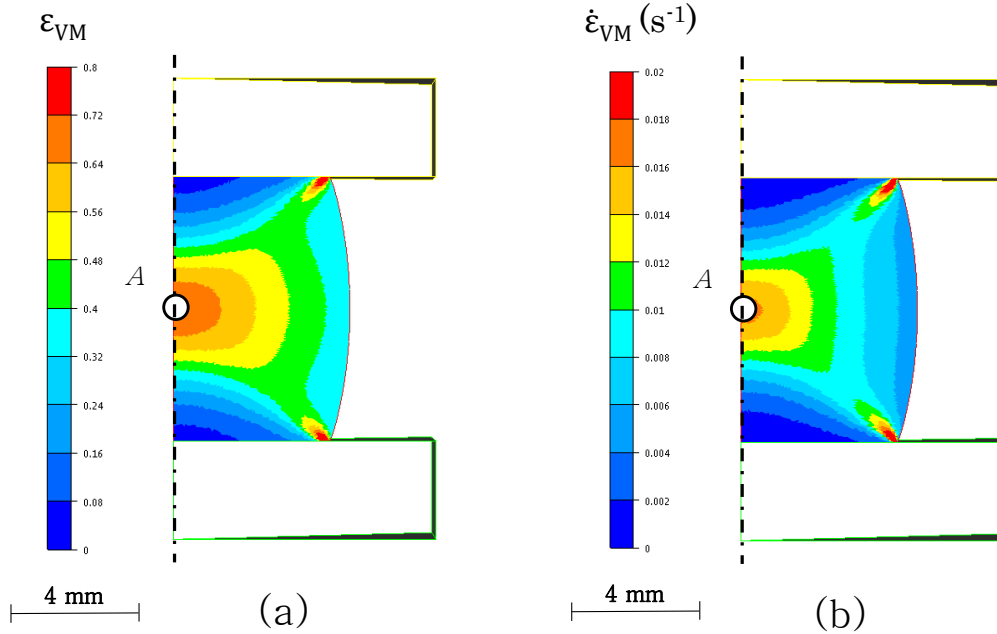
Fig. 5.4. Finite element simulations performed on a cylindrical sample at T = 1273K and \dot{\varepsilon} = 0.008s^{-1} at the final stage of the simulation ( h_f \simeq 2/3h_0 ). Presented fields are (a) equivalent plastic strain and (b) equivalent plastic strain rate.
