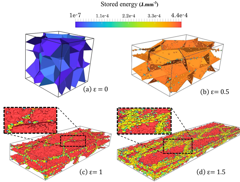
Fig. 4.8. Illustrated case of a DRX simulation using the full field model of chapter 3. The simulated process is a channel-die compression on a 304L steel at a temperature of 1273K and a strain rate of 0.01s^{-1} .
