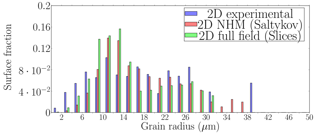
(b) T=1373\text{K} , \dot{\varepsilon}_{\text{VM}}=0.014\text{s}^{-1} , \varepsilon_{\text{VM}}=1 , X_{\text{expe}}=51.3\%
