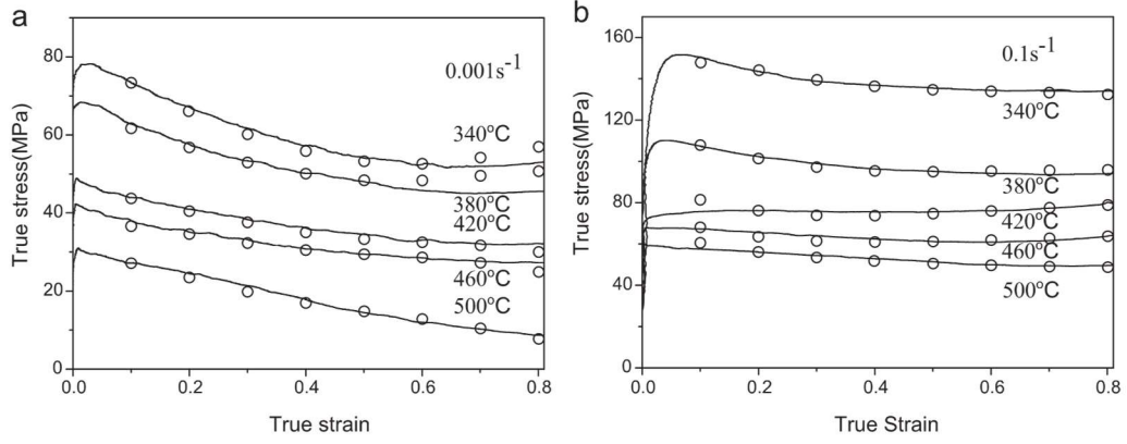
Figure II-20 Comparisons between the experimental (solid lines) and predicted (points) flow stress of Al-Cu-Mg-Ag alloy at (a) 0.001 s -1 and (b) 0.1 s -1 [84]
