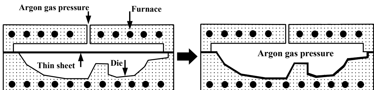
Figure I-2 Principle of Superplastic Forming (SPF) [7]
