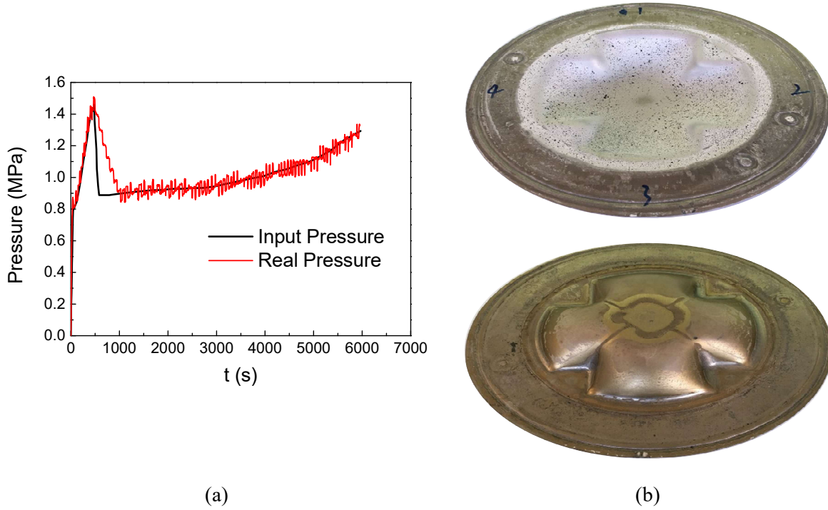
Figure V-11 (a) Experimental pressure evolution and (b) the deformed plate for the cross die deformed at changed strain rate
