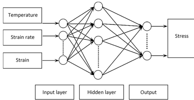
Figure II-19 Schematic structure of back propagation neural network [84]
