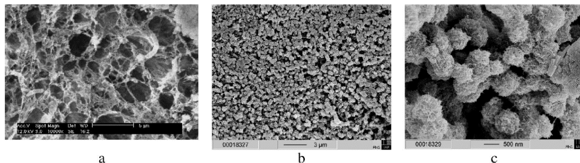
Figure 1.15 – Morphology of cellulose aerogels depending on solution state before coagulation from NMMO dissolution. Aerocellulose prepared from solid (a) and molten (b, c) Solucell950/NMMO solution regenerated in water at 25 °C with further water to acetone exchange and dried in supercritical conditions. Reprinted with permission from Gavillon and Budtova (2008). Copyright (2008) American Chemical Society.
