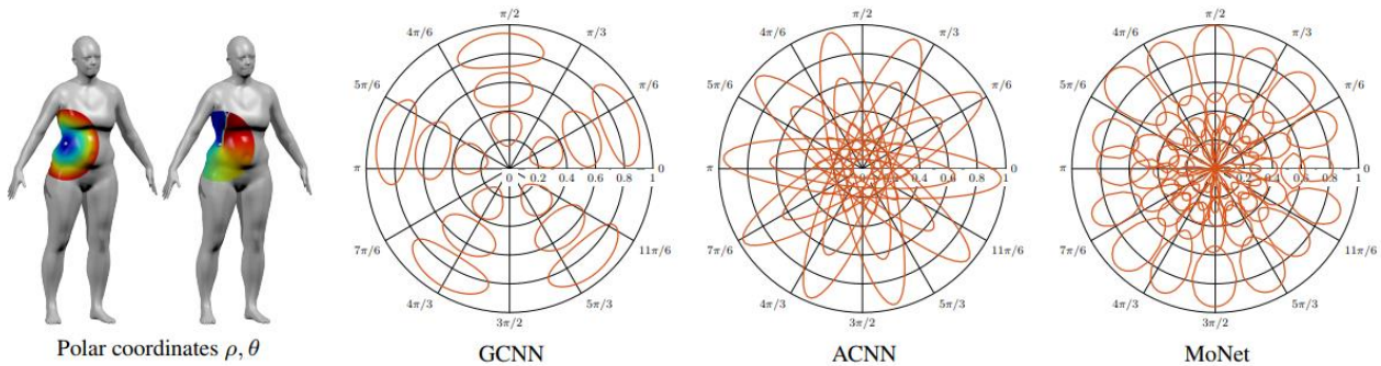
Figure 40. Illustration of the patch operators from methods using polar coordinates to define their filters. Figure from (Monti et al., 2017).
