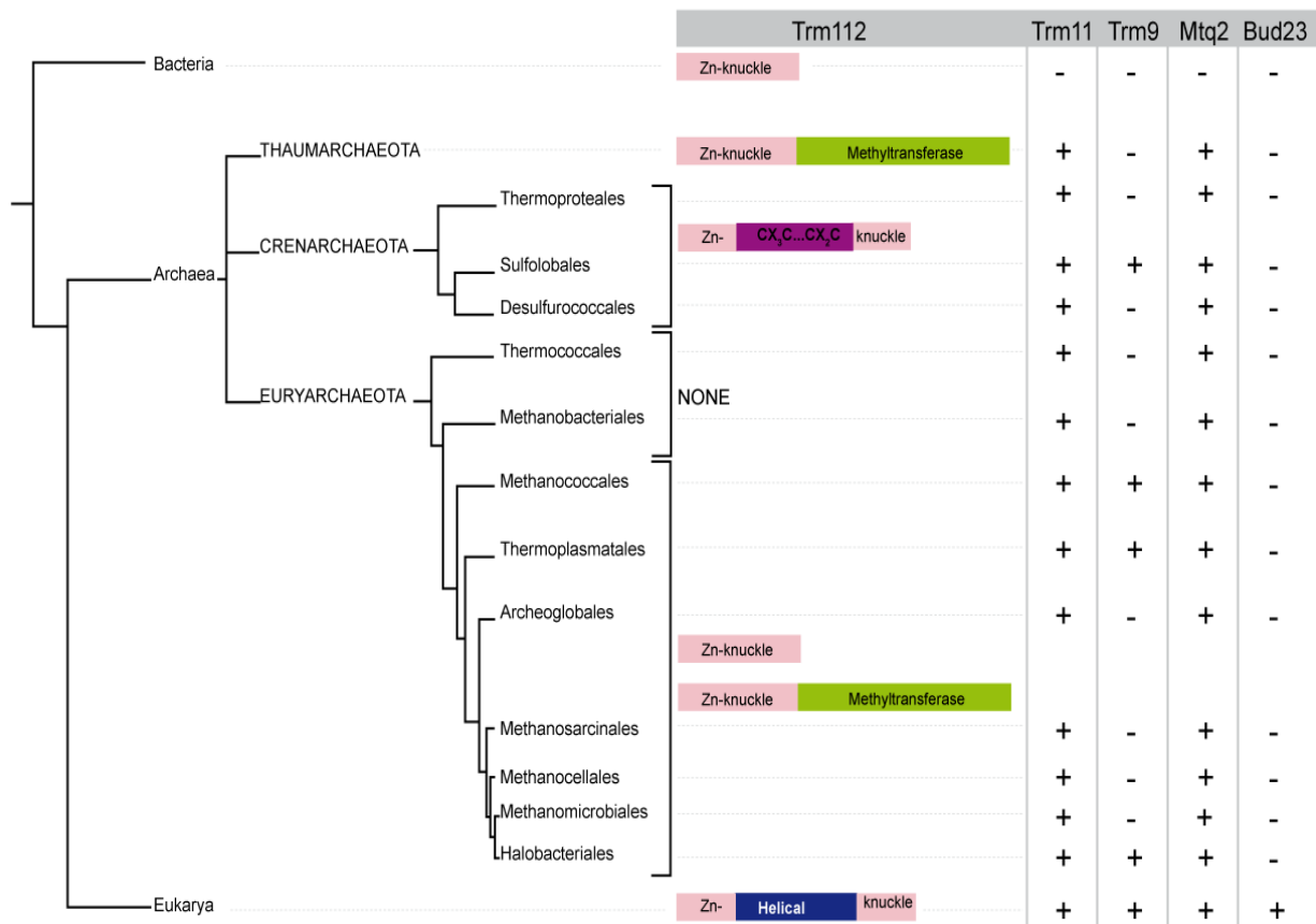
Figure 22. Trm112 is present in the three domains of life. Simplified phylogenetic tree of Trm112. Emphasis is given to archaeal phylogeny. The distribution of Trm11, Trm9, Mtq2 and Bud23 proteins within the three domains of life is indicated. The various Trm112 forms identified are schematically depicted.
