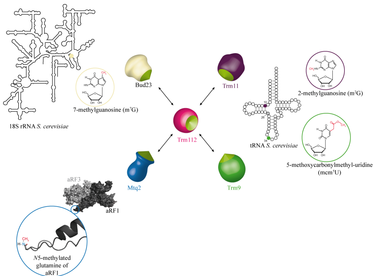
Figure 17. Schematic representation of Trm112-MTase interaction network and of the substrates of these complexes. The surface representation of the aRF1-aRF3 complex from Aeropyrum pernix archaean was generated using PDB code 3VMF (Kobayashi et al., 2012). Positions 10, 26 and 34 on a tRNA molecule are shown in purple, grey and green, respectively. Position of G 1575 on 18S rRNA is shown as a beige sphere.
