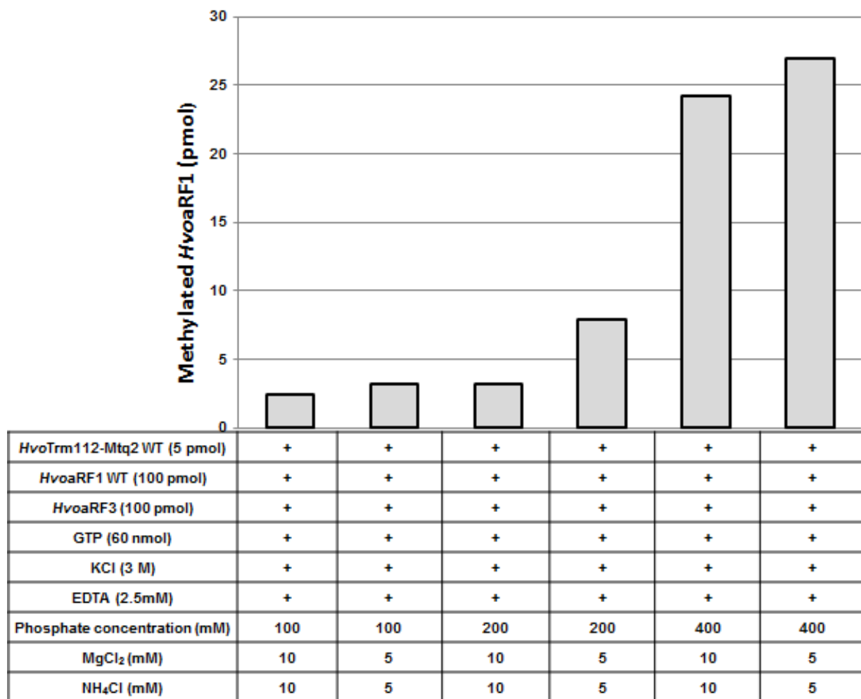
Figure 32. Buffer optimization for enzymatic activity of Hvo Mtq2-Trm112. Different buffer conditions tested were indicated in the table below the graph.
