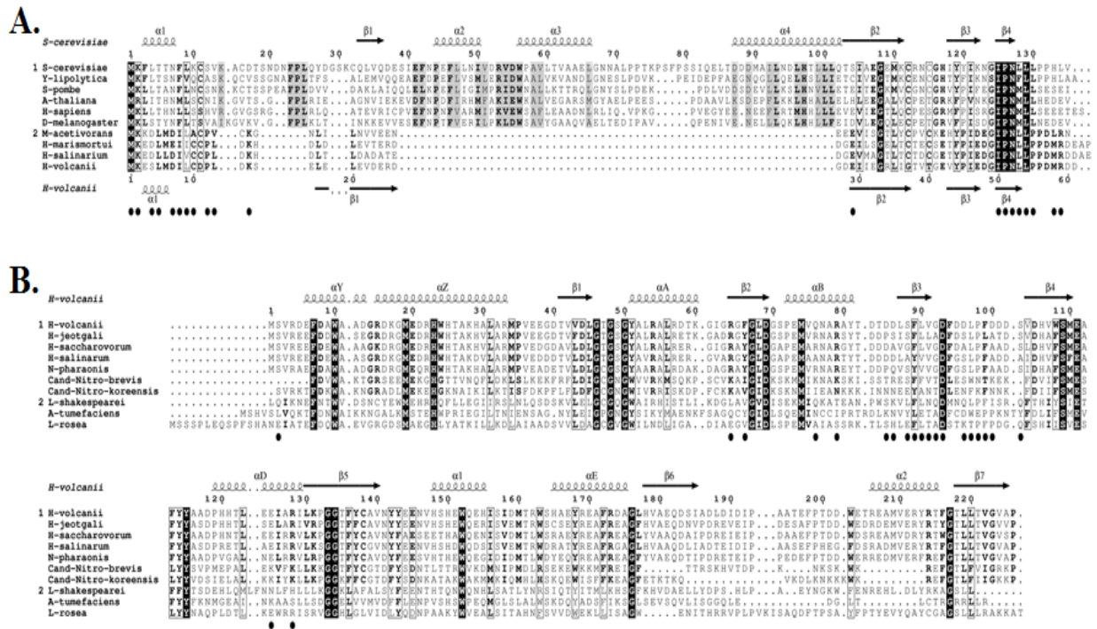
Figure 43. Sequence alignment of HvoTrm112 and HVO_0019 sequences.
