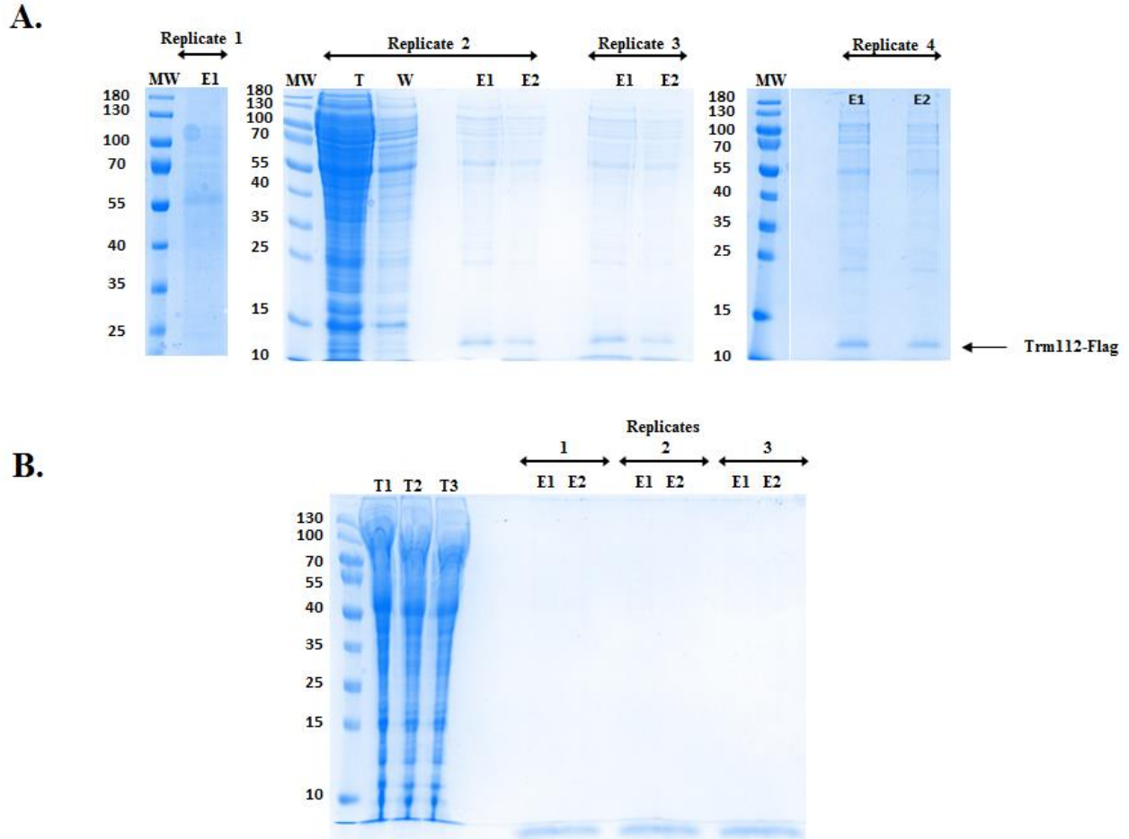
Figure 26. Co-IP experiments.
