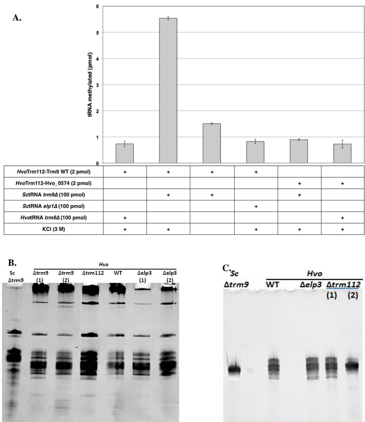
Figure 37. Enzymatic assay for HvoTrm112-Trm9 complex. (A). Enzymatic activities of HvoTrm112-Trm9 complex. The conditions (proteins, salt and ligand) used for each experiments are indicated in the table below the graph. The number of methylated substrate (in pmol) after a 2 h reaction is indicated for every condition. Errors bars have been calculated from the results of three independent experiments. (B). Total RNA purification from different H. volcanii strains by phenol-chloroform extraction; (C). tRNA purification from different total RNAs by polyacrylamide-urea gel extraction.
