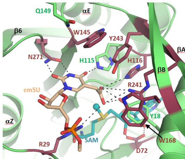
Figure 47. Docking model of \text{cm}^5\text{U} into the active site of Y. lipolytica Trm9. The residues are numbered based on the S. cerevisiae protein. A manually docked \text{cm}^5\text{U} nucleotide is shown as beige sticks and potential hydrogen bonds that it could form with Trm9 active site residues are depicted by dashed black lines. The modeled SAM molecule is shown as blue sticks and the methyl group to be transferred is shown as a sphere (Letoquart et al., 2015b).
