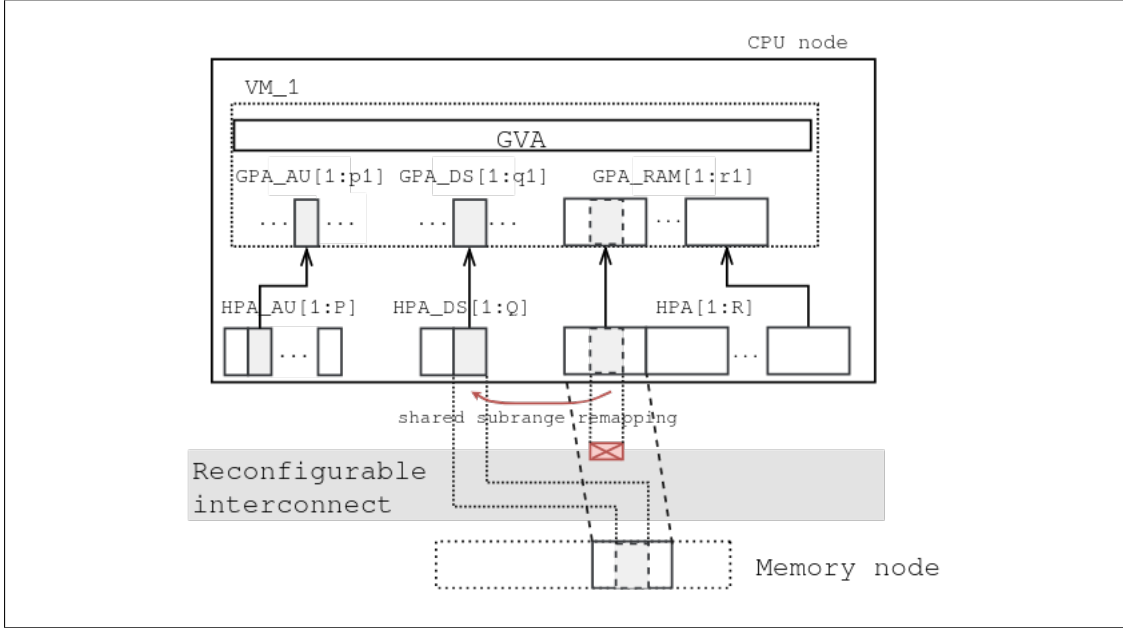
Figure 4-6: Dedicated slot initialization from an existing RAM
