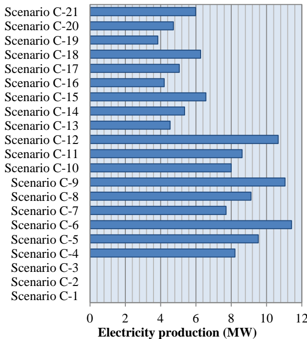
Figure 4.20. Electric power generation from CS_{3, set q}^{wood}
