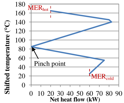
Figure 1.10. Grand composite curve
