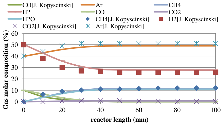
Figure 3.21. Gas composition profile in the methanation unit
