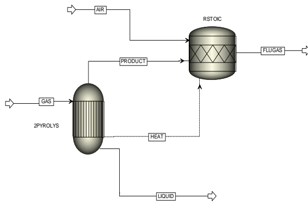
Figure 3.24. Furnace assembly on Aspen plus ®
