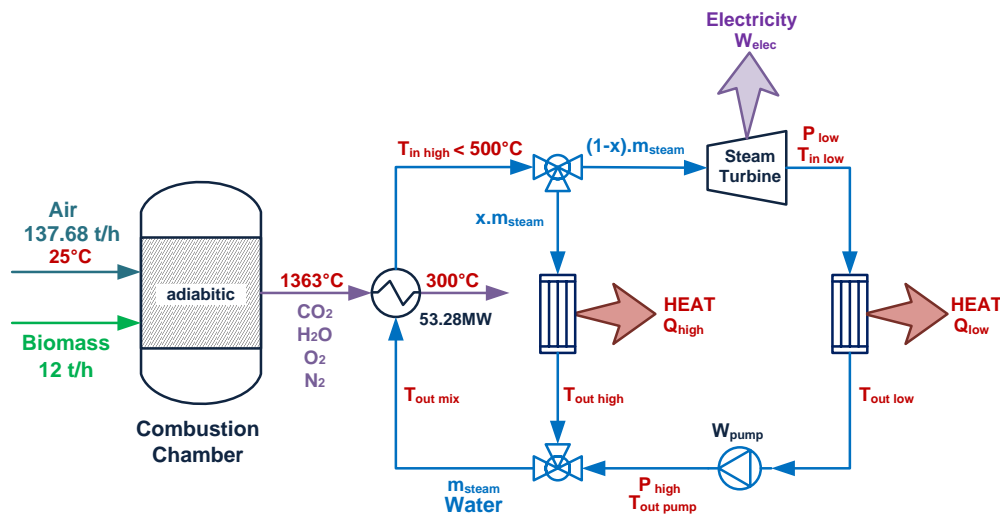
Figure 4.7. Wood cogeneration process flow sheet
