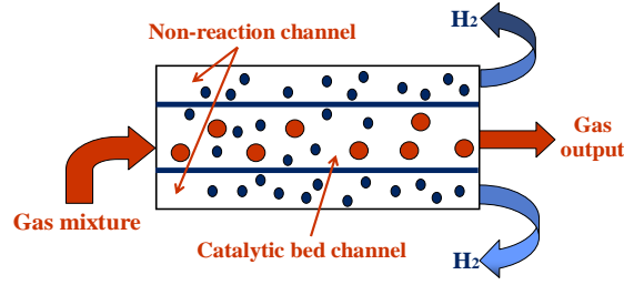
Figure 3.15. Water Gas-Shift membrane reactor
