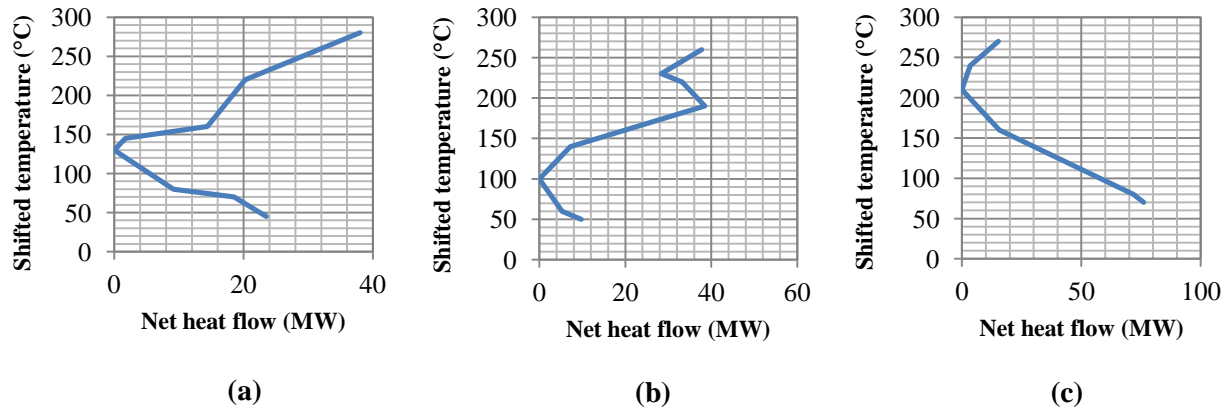
Figure 3.2. Grand Composite Curves of each actor of the territory (a) Site 1, (b) Site 2, (c) Site 3
