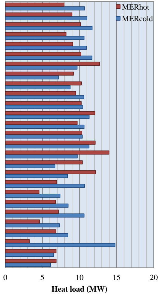
Figure 4.17. MER_{hot} and MER_{cold} of CS_{2, set q}^{wood}
