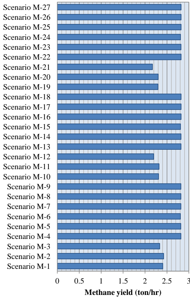
Figure 4.16. Methane yield from CS_{2, set q}^{wood}
