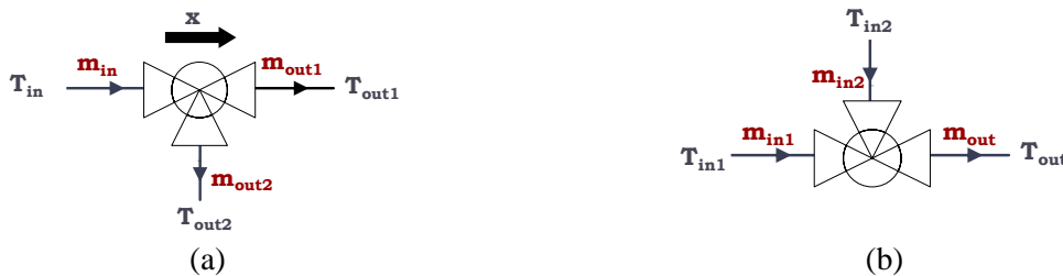
Figure 3.25. (a) Splitter unit, (b) mixer unit
