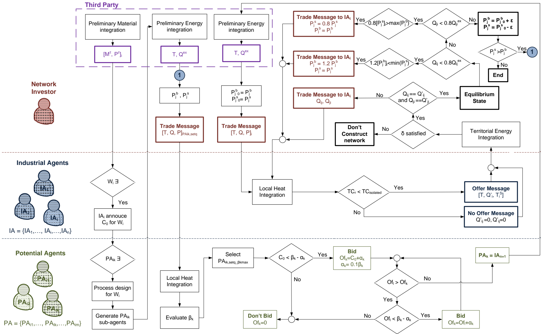
Figure 2.12. Agent interactions work flow framework for the territorial integration of conversion systems in a non-cooperative scheme
