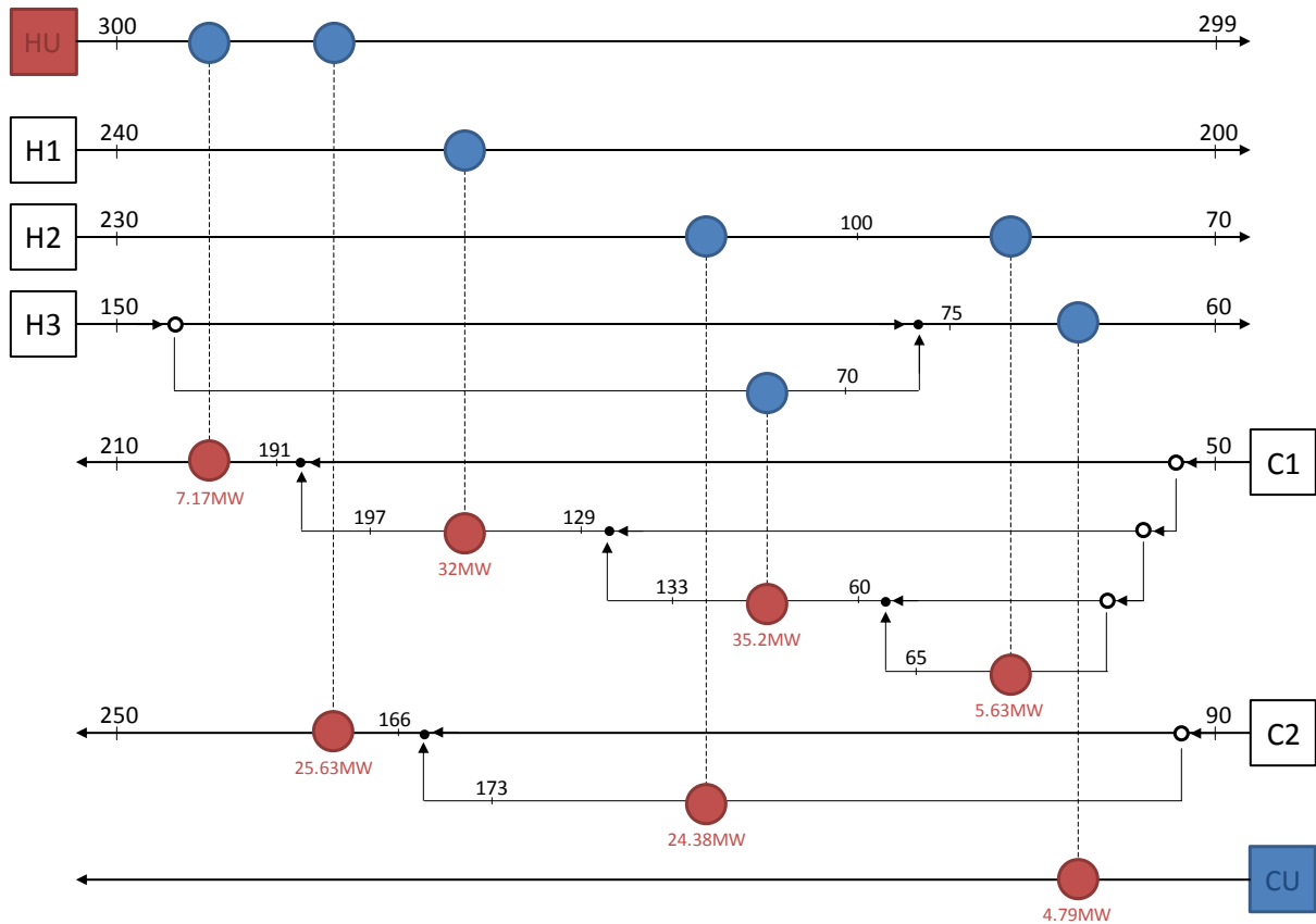
Figure 4.2. HEN of Site 2 as an isolated industrial actor
