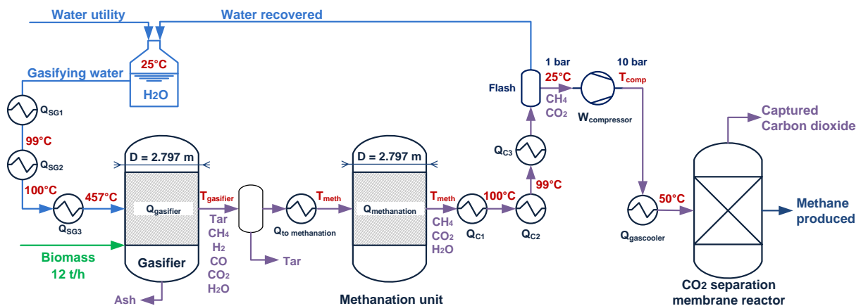
Figure 4.6. Wood to methane conversion process flow sheet
