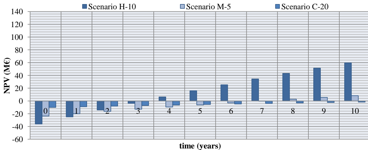
Figure 4.29. NPV over ten years for the best scenario of each pathway with 100€ the ton of wood
