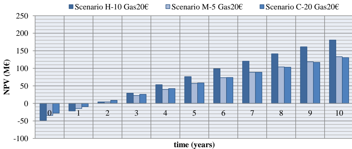
Figure 4.31. NPV over ten years for the best scenario of each pathway with a low gas market price
