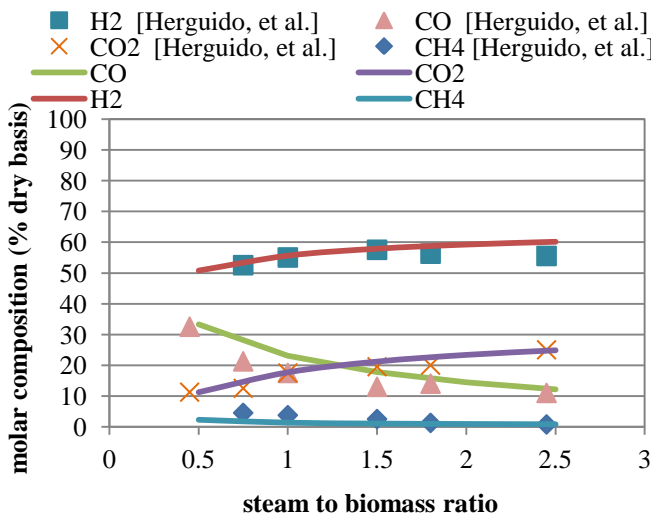
Figure 3.11. Steam to biomass effect on gas composition
