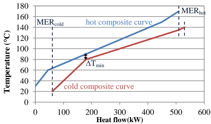
Figure 1.9. Hot and cold composite curves representation
