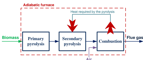
Figure 3.23. Adiabatic furnace block diagram
