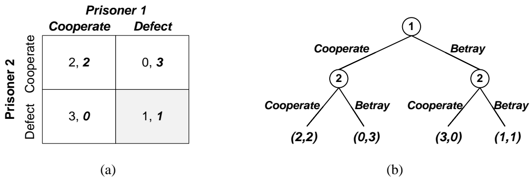
Figure 2.11. The prisoner's dilemma: a) normal form, b) extensive form
