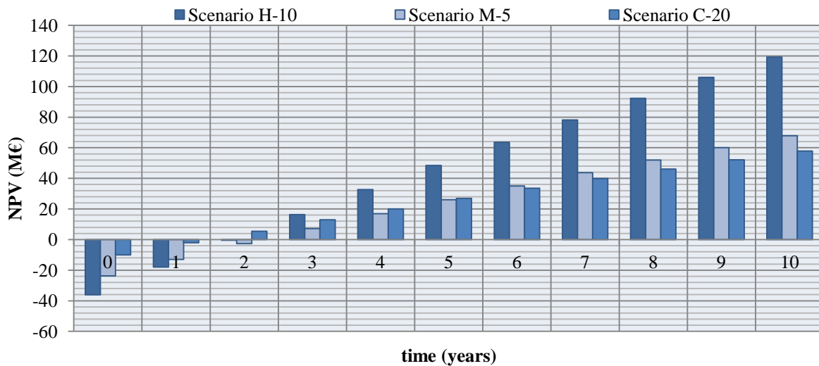
Figure 4.23. Comparison of the NPV over ten year period for the best scenario of each pathway
