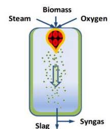
Figure 3.7. Entrained flow gasifier
