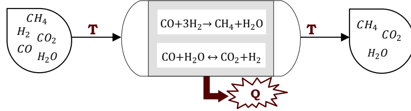
Figure 3.20. Methanation unit
