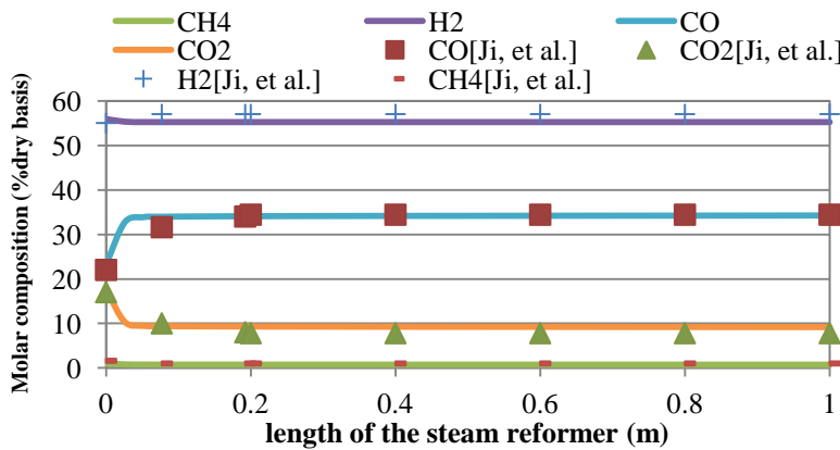
Figure 3.14. Gas composition profile along the steam reformer
