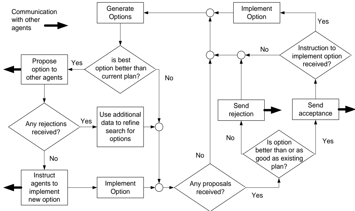
Figure 2.9. Agent principled negotiation (Wangermann & Stengel, 1999)
