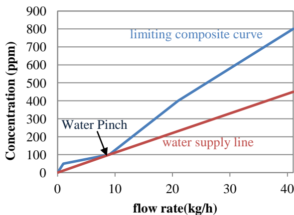
Figure 1.12. Limiting composite curves- water pinch
