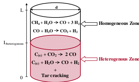
Figure 3.8: The chemical reactions taking place in the gasifier
