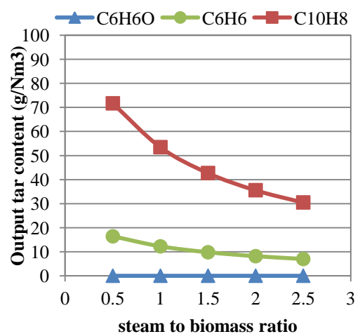
Figure 3.12. Steam to biomass effect on the tar content of the gasifier's output
