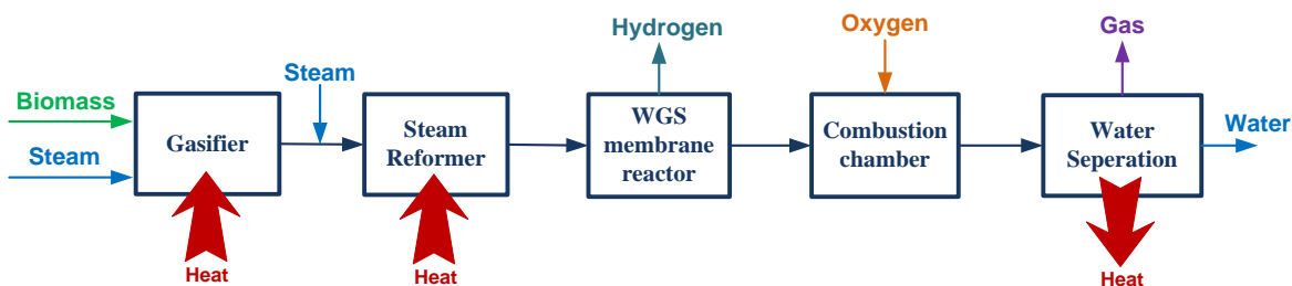
Figure 3.4. Block flow diagram of wood waste conversion to hydrogen
