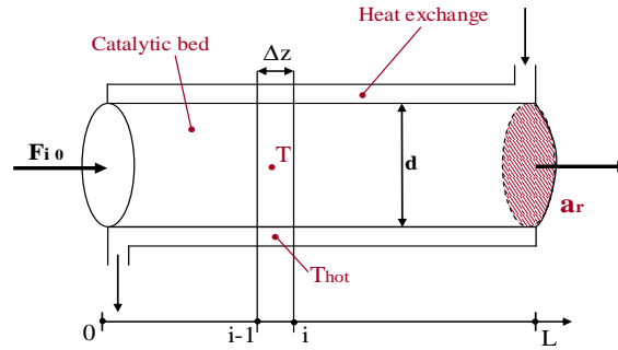
Figure 3.13. Steam reformer geometric form
