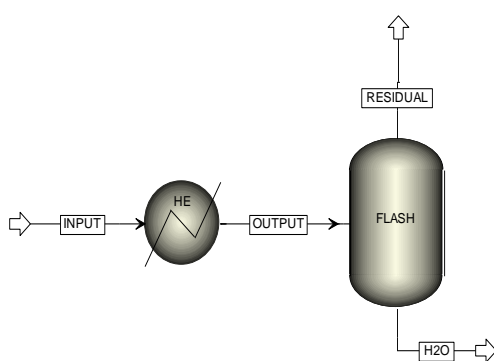
Figure 3.18. Separation unit on Aspen plus®
