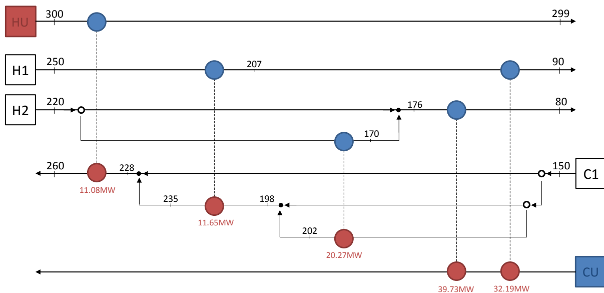
Figure 4.3. HEN of Site 3 as an isolated industrial actor
