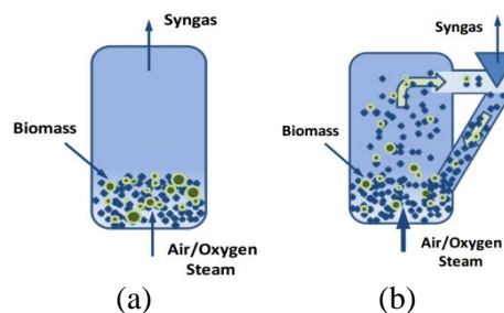
Figure 3.6. Fluidized bed gasifier: (a) bubbling, (b) circulating
