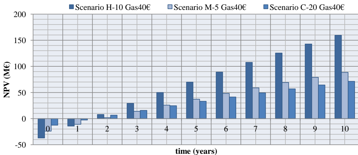
Figure 4.32. NPV over ten years for the best scenario of each pathway with a high gas market price
