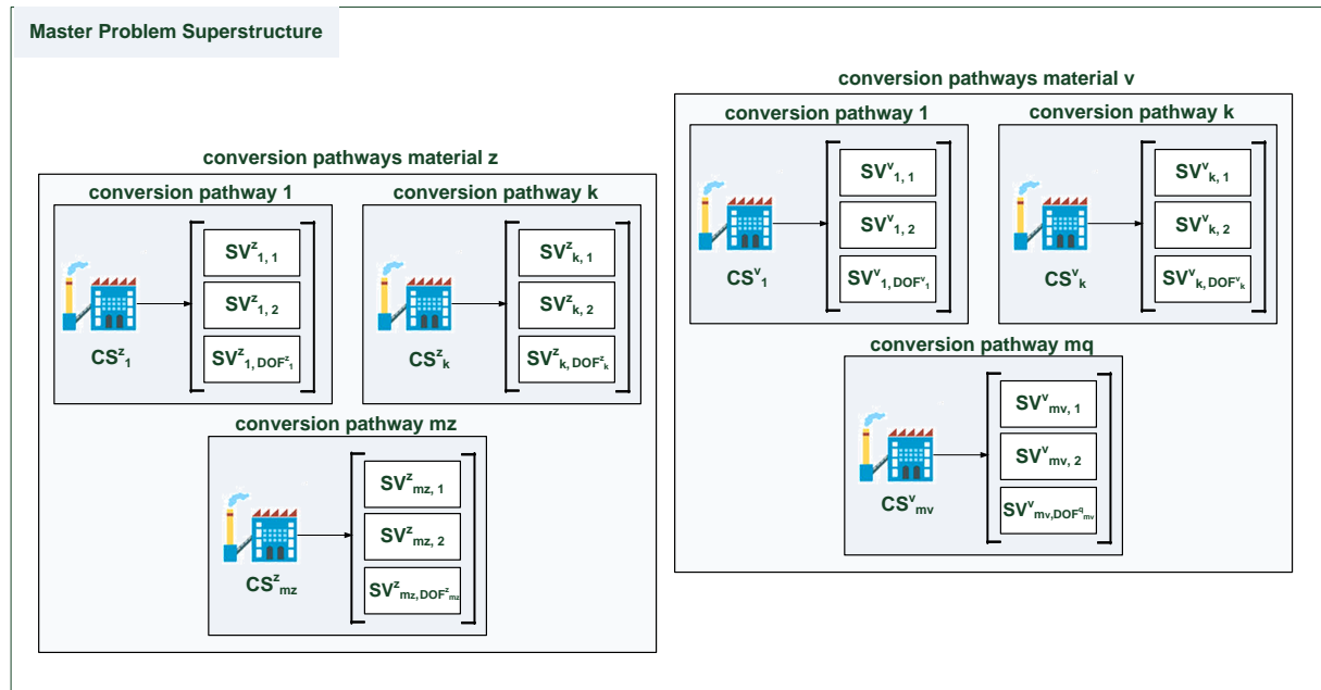
Figure 2.5. Master Problem superstructure of the conversion pathways
