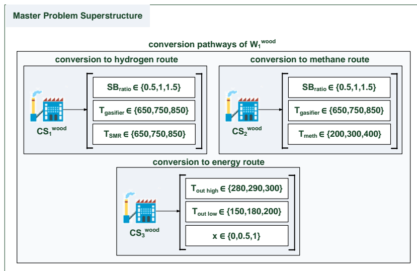
Figure 4.8. Superstructure of W 1 wood conversion pathways
