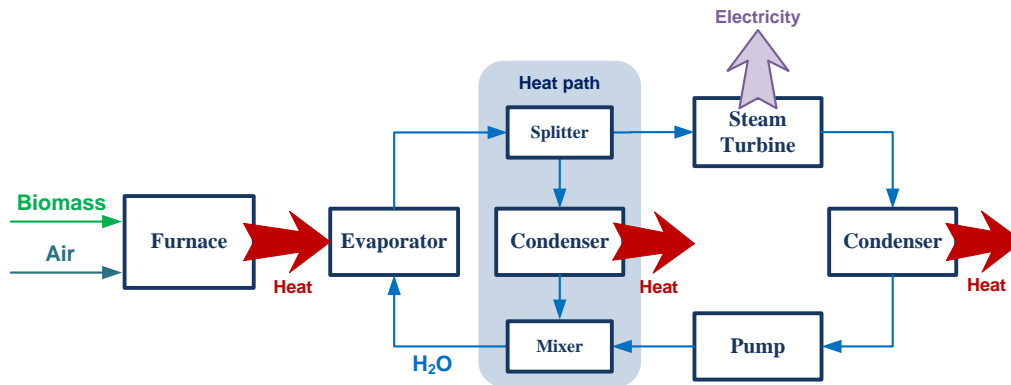
Figure 3.22. Block flow diagram of wood waste conversion to electricity and heat
