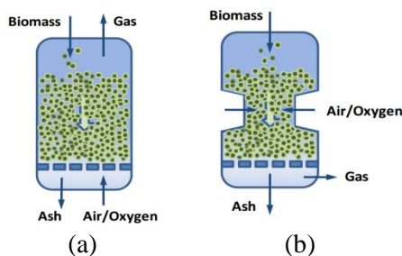
Figure 3.5. Fixed bed gasifier: (a) updraft, (b) downdraft
