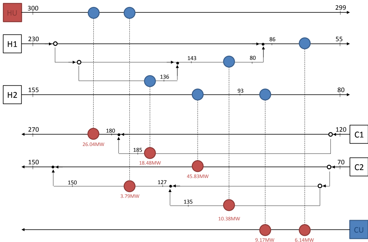
Figure 4.1. HEN of Site 1 as an isolated industrial actor
