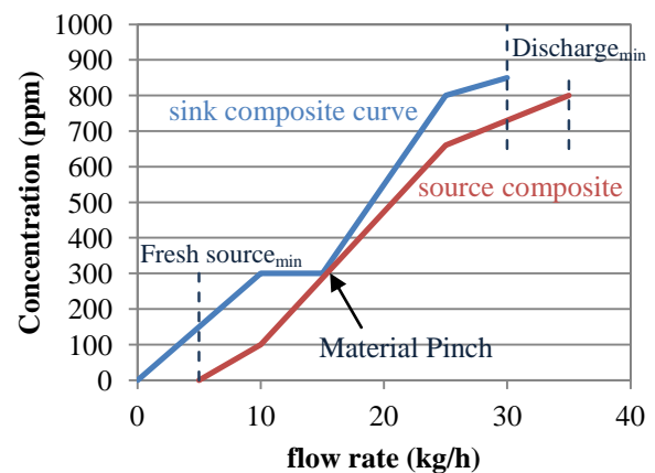
Figure 1.13. Source/sink composite curves
