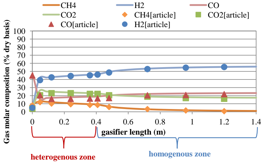
Figure 3.10. Gas composition profile along the gasifier length
