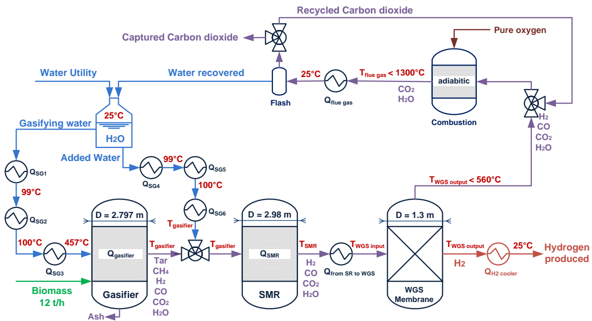
Figure 4.5. Wood to hydrogen conversion process flow sheet
