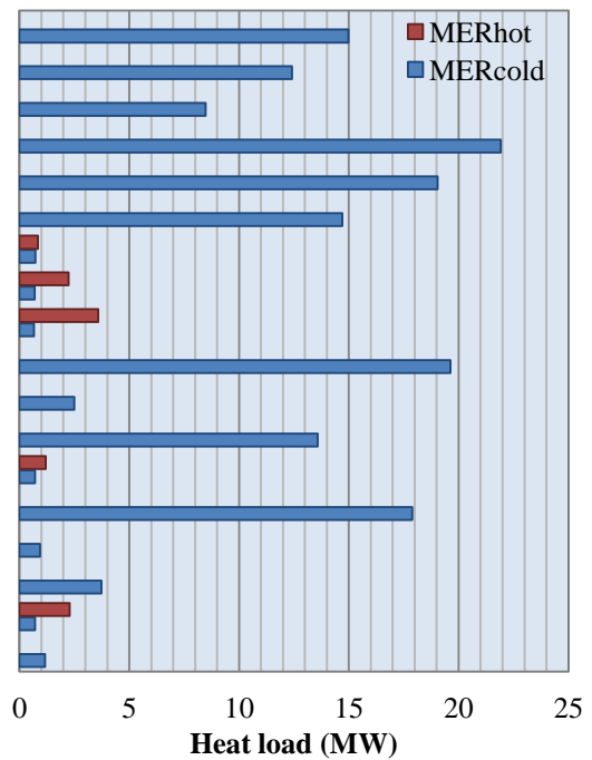
Figure 4.13. MER_{hot} and MER_{cold} of CS_{1, set q}^{wood}
