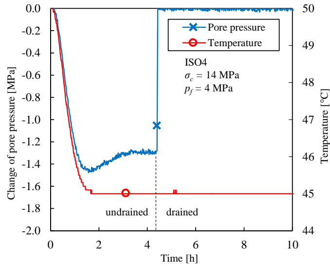
Fig. 5.3.: Typical three stage thermal test on ISO4: response in pore pressure resulting from an undrained decrease in temperature from 50 to 45 °C, followed by drainage opening and pore pressure dissipation
