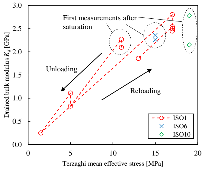
Fig. 4.6.: Measured stress dependent drained bulk modulus K_d on samples ISO1, ISO6 and ISO10, illustrating the reversible reduction of stiffness with decreasing effective stress
