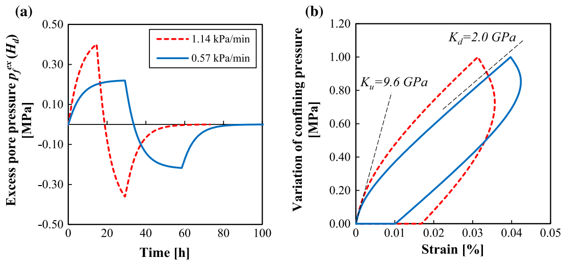
Fig. 3.28.: a) Calculated pore pressures in the specimen centre and b) measured volumetric strains for the fast loading path (red dotted line) and the slow loading path (blue solid line)
