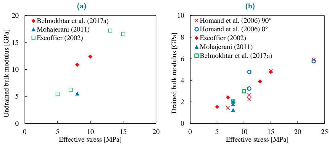
Fig. 2.6.: a) Undrained bulk modulus and b) drained bulk modulus with respect to effective stress
