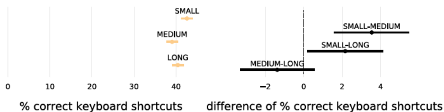
Figure 5.10: (A): Mean rate of correct keyboard shortcuts per command length. (B): Mean rate difference of correct keyboard shortcuts between command lengths. All error bars are 95% CIs.
