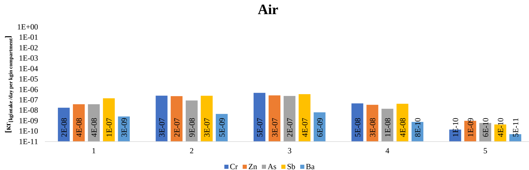
Figure 90. Exposure factor calculated for Cr, Zn, As, Sb, Ba for the surveyed areas, exposure through air, \text{kg}_{\text{intake}}/\text{day per kg}_{\text{in compartment}} , Lg scale
