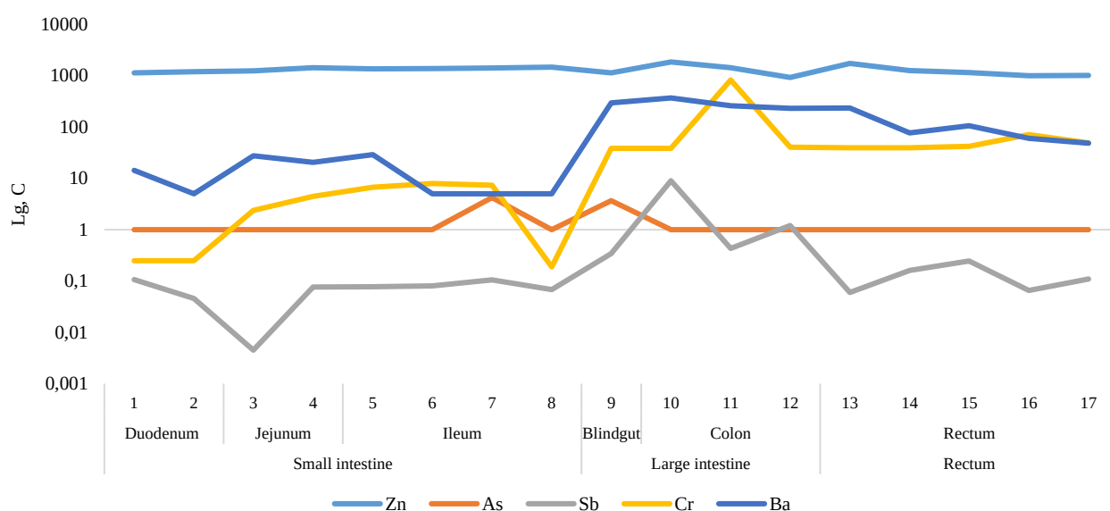
Figure 58. The content of Zn, As, Sb, Cr, Ba in the intestines of domestic pigs ( Sus scrofa domesticus ), Ekibastuz, mg/kg ash residue, LgC
