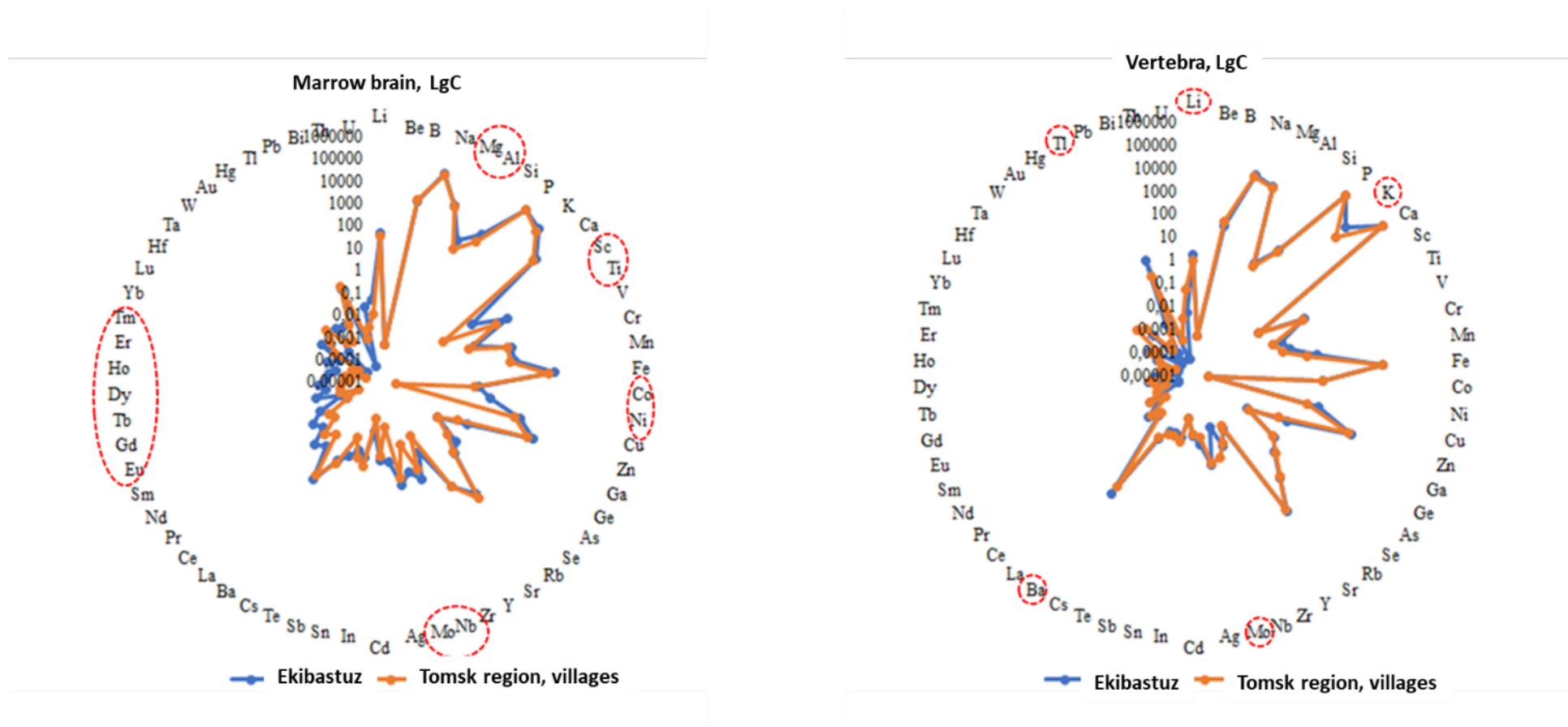
Figure 33. The content of chemical elements in the bone and spinal cord of domestic pig ( Sus scrofa domesticus ) according to the results of ICP-MS analysis
