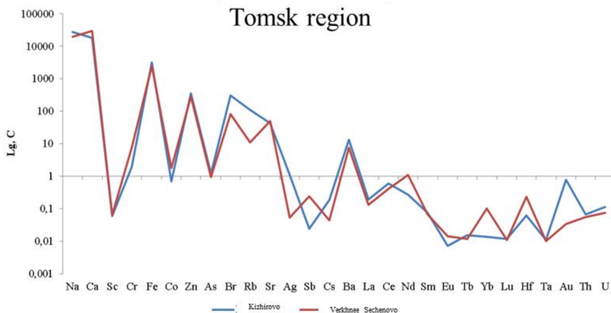
Figure 22. The elemental composition of the biological material of/from domestic pigs ( Sus scrofa domesticus ) in Tomsk region, LgC ash residue
