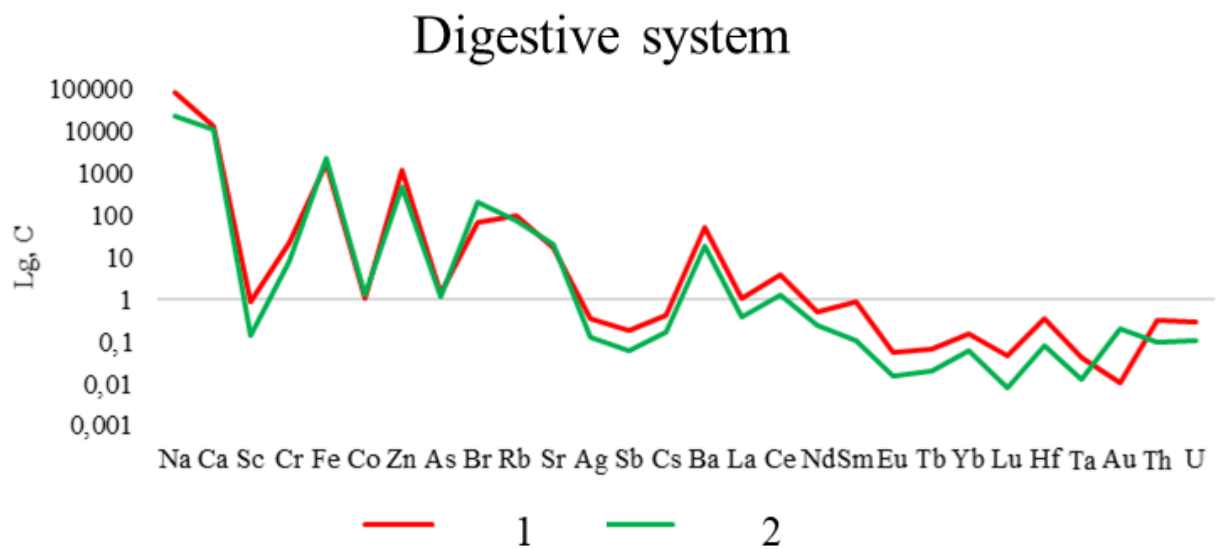
Figure 40. The content of chemical elements in the gastrointestinal tract of domestic pigs ( Sus scrofa domesticus ), mg/kg
