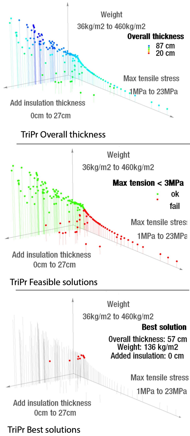
Figure 4.7: Pareto fronts comparison, Triangle prisms tessellation
