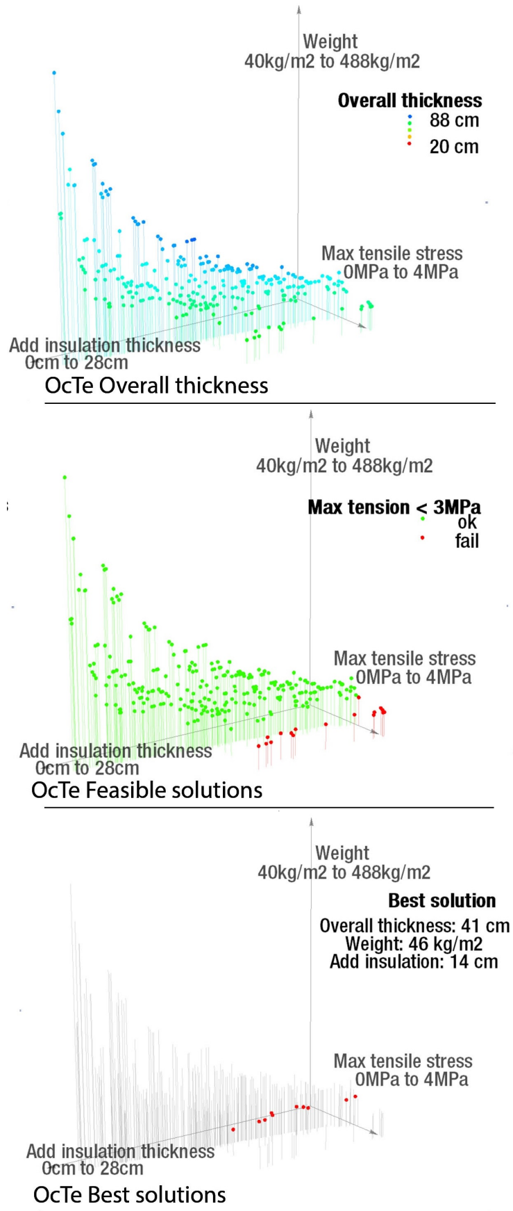
Figure 4.6: Pareto fronts comparison, Octahedra and tetrahedra tessellation
