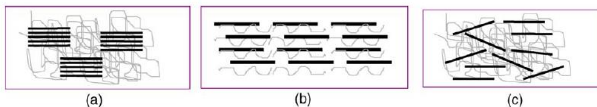
Fig. 1.2. Typical dispersion state of polymer/layered nanoclay composites: (a) no chain penetration (i.e., microcomposite), (b) chain intercalation, and (c) nanoclay exfoliation (i.e., nanocomposite) [44]. Copyright 2006, Reproduced with permission from Elsevier Ltd.
