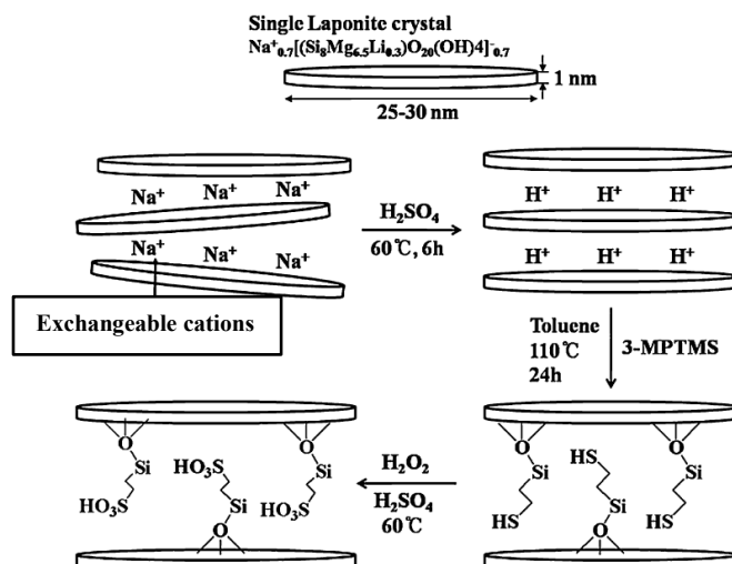
Fig. 1.39. Laponite sulfonated using \text{H}_2\text{SO}_4 and \text{H}_2\text{O}_2 through exchangeable cations [90]. Copyright 2012, Reproduced with permission from Elsevier Ltd.
