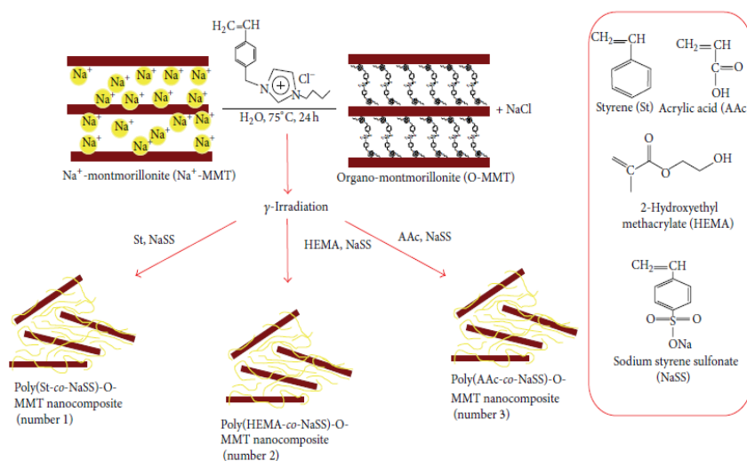
Fig. 1.16. Schematic diagram of three kinds of vinyl polymer/Cloisite \text{Na}^+ nanocomposite prepared by radiation-induced polymerization [142]. Copyright 2014, Reproduced with permission from Hindawi.
