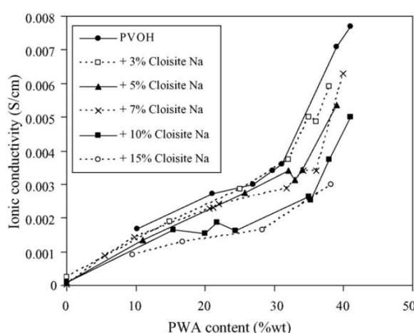
Fig. 1.10. Proton conductivity of pristine PVOH, PVOH/Cloisite Na^+ and PVOH/Cloisite Na^+ /phosphotungstic acid membranes [44]. Copyright 2006, Reproduced with permission from Elsevier Ltd.
