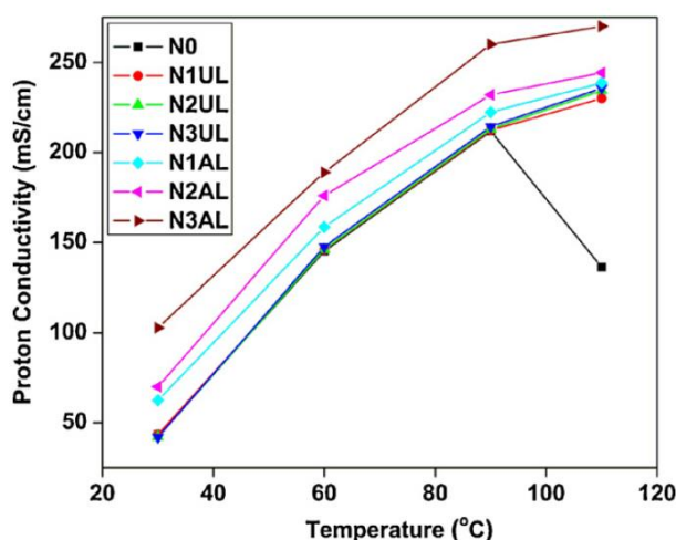
Fig. 1.41. Proton conductivity of (a) pristine Nafion (i.e., N0), (b) Nafion/ \text{Na}_4\text{P}_2\text{O}_7 -activated Laponite (i.e., NxUL series) and (c) \text{H}_3\text{PO}_4 -activated Laponite (i.e., NxAL series) membranes [41]. Copyright 2012, Reproduced with permission from Elsevier Ltd.
