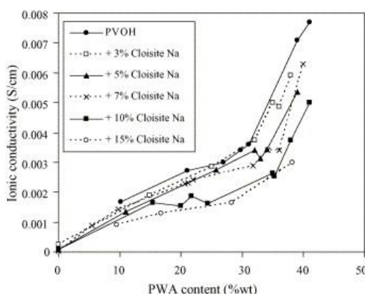
Fig 1.31. Proton Conductivity of PVOH composite membranes according to the content of phosphotungstic acid and Cloisite Na + . Copyright 2005, Reproduced with permission from Elsevier Ltd [44].
