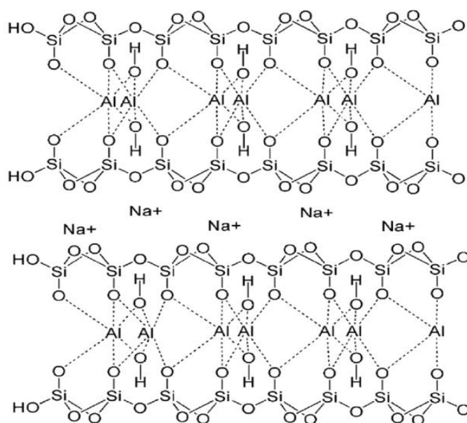
Fig. 1.1. Structure of unmodified montmorillonite nanoclay (trade name: Cloisite \text{Na}^+ ) [86]. Copyright 2015, Reproduced with permission from Elsevier Ltd.
