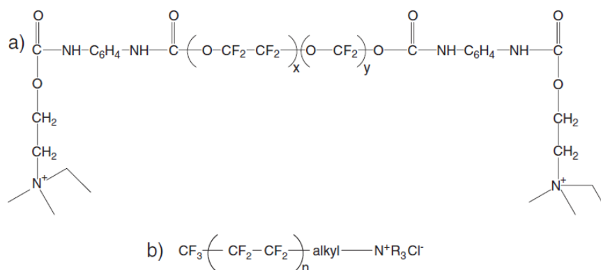
Fig. 1.26. Chemical structure of (a) PFPE- \text{NR}_3 ( x = y = 14 ) and (b) Zonyl ( n = \pm 5 ) [8]. Copyright 2006, Reproduced with permission from Elsevier Ltd.
