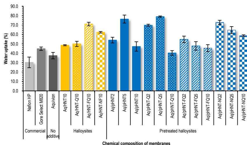
Fig. 5.9. Data on water uptake: commercially available Nafion HP and Gore Select M820, and pristine Aquivion and Aquivion composite membranes containing quercetin-grafted halloysites. Yellow and blue bars represent non-pretreated and pretreated nanoclays, respectively.
