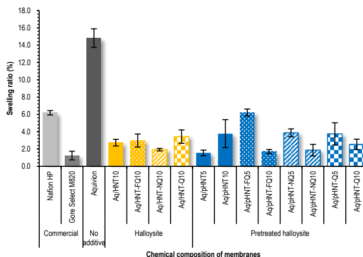
Fig. 5.10. Data on swelling ratio: commercially available Nafion HP and Gore Select M820, and pristine Aquivion and Aquivion composite membranes containing quercetin-grafted halloysites. Yellow and blue bars represent non-pretreated and pretreated nanoclays, respectively.
