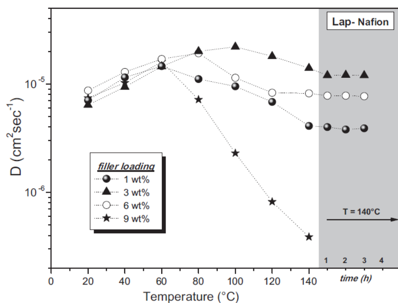
Fig. 1.35. Self-diffusion coefficients based on different temperature and laponite loadings within composite membrane prepared using DMF [35]. Copyright 2012, Reproduced with permission from Elsevier Ltd.
