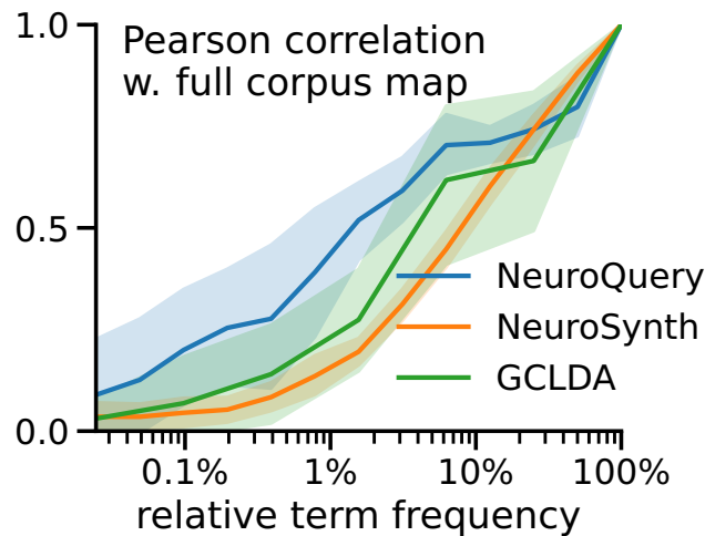
Figure 8.5: Convergence of maps toward their value for the full corpus, as the number of occurrences increases. Averaged over 13 words: “language”, “auditory”, “emotional”, “hand”, “face”, “default mode”, “putamen”, “hippocampus”, “reward”, “spatial”, “amygdala”, “sentence”, “memory”.
