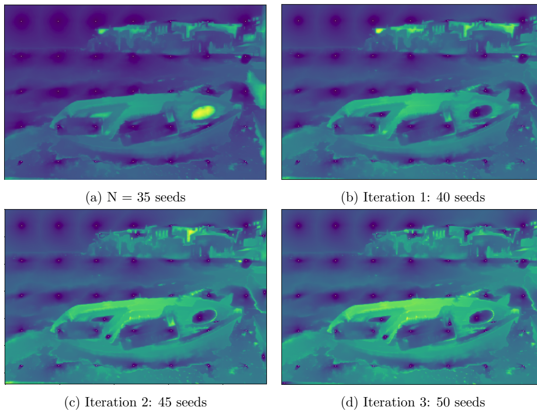
Figure 2.6 – Illustration of the refinement on an image of the BSDS500. Each figure displays the arrival time at each pixel. At each step, new seeds are added at superpixels where the arrival time is maximal.
