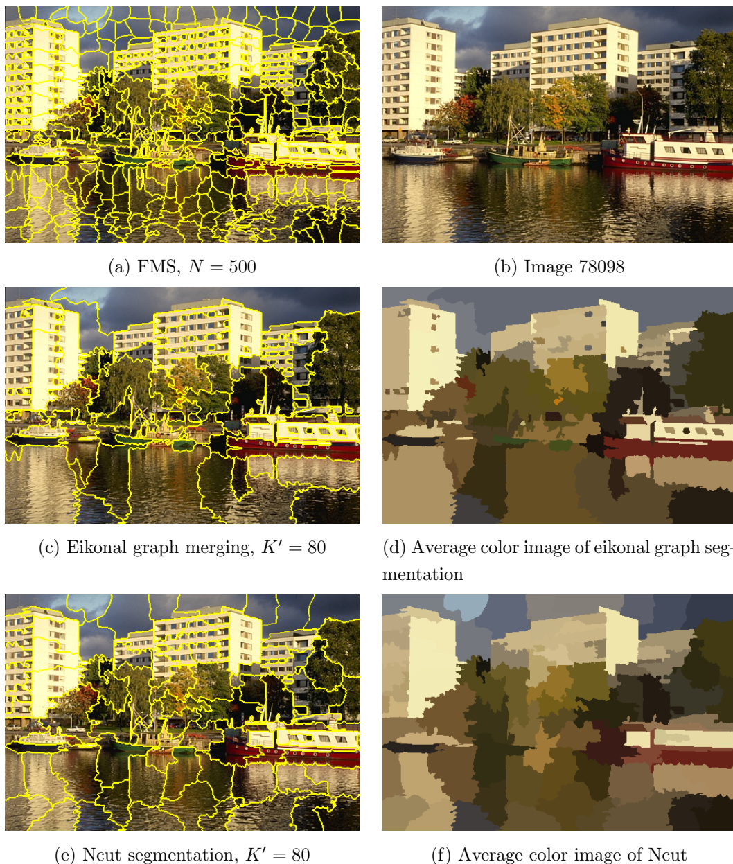
Figure 5.2 – One-stage segmentation of a test image of the BSD using Eikonal algorithm. For this image, the boundary recall is 0.69 (Eikonal) and 0.63 (Ncut), the boundary precision is 0.30 (Eikonal) and 0.26 (Ncut).
