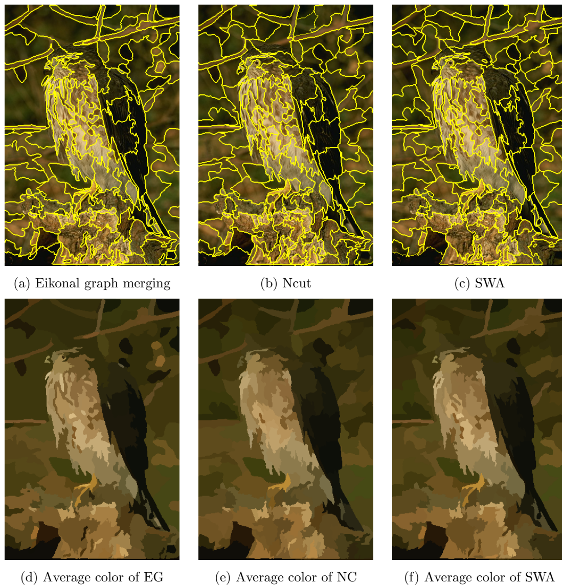
Figure 5.3 – Result of the first stage of the segmentation of a test image of the BSD using the Eikonal graph, normalized cut and SWA algorithm. Images in the second row show the average color of each segment. “EG” represents Eikonal graph merging, “NC” for Ncut. The boundary recall are 0.84, 0.80, 0.80; the boundary precision are 0.15, 0.13, 0.13, and the final partition comprises 153, 150, and 154 segments respectively.
