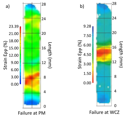
Figure 2.43: \varepsilon_{PP} fields for a PM Ti5553 specimen and a cross-weld Ti5553 specimen Dalgaard et al. (2012a).
