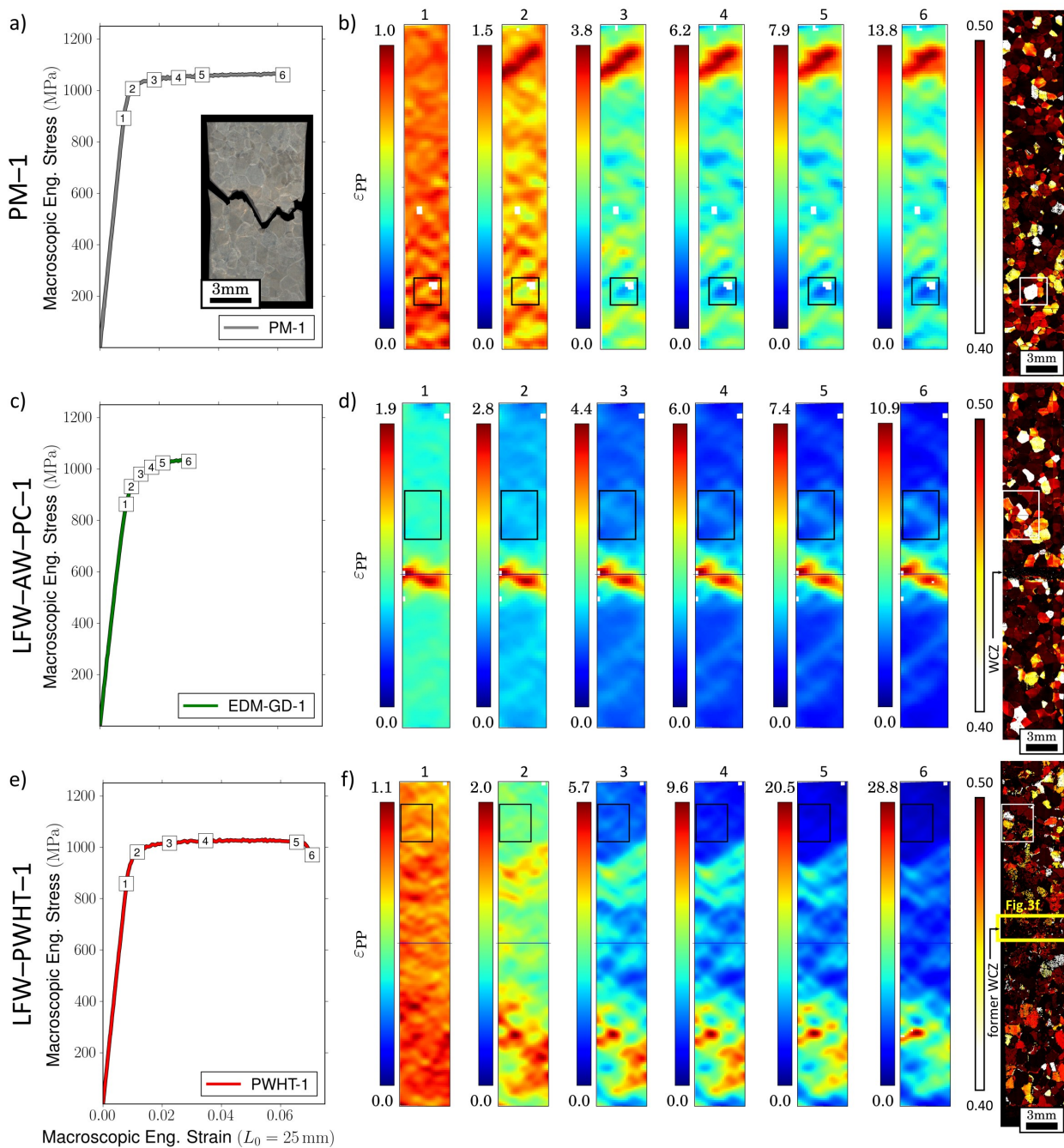
Figure 7.5: a-c-e) Tensile tests, b-d-f) \epsilon_{PP} cumulated strain fields and Schmid's factor mappings for the tensile specimens: a-b) PM-1, c-d) LFW-AW-PC-1 and e-f) PWHT-1.
