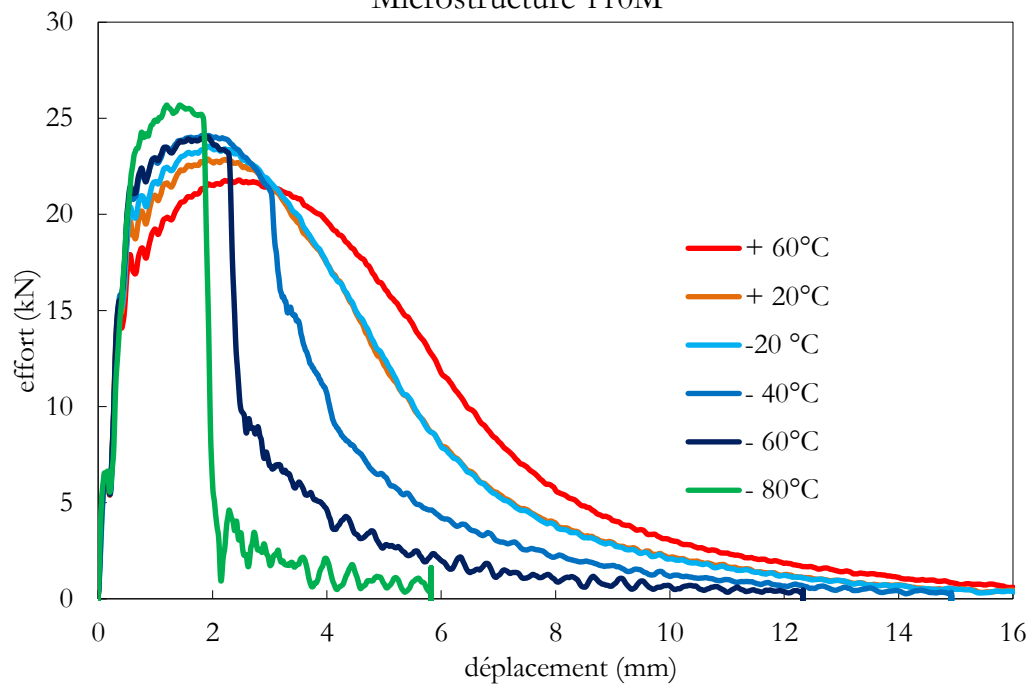
Microstructure 110M
