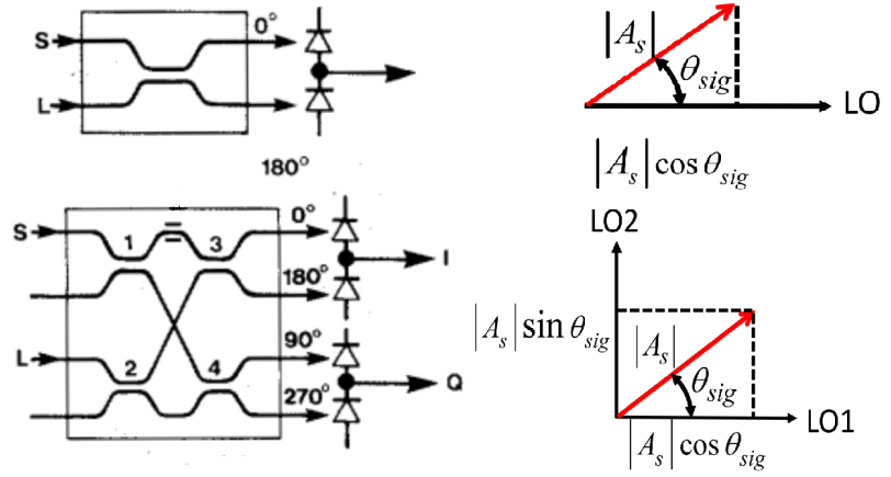
Figure 2.1: Optical hybrid scheme. Functional representation of 180^\circ (top) and 90^\circ hybrids with photodetectors in balanced configuration. The signal phasors with respect to the LO are represented in the right side for each case. Figure adapted from [74, 75].
