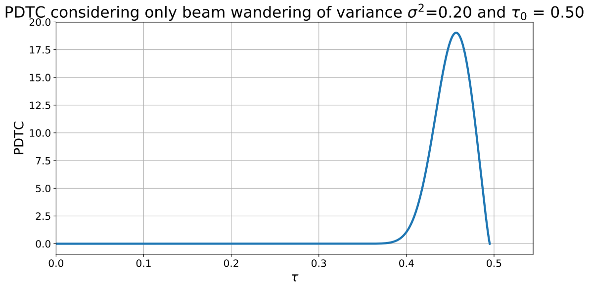
Figure 8.6: PDTC \mathcal{P}(\tau) for a receiver with aperture radius a = 0.75 m, beam width at receiver W = 2.0 m and beam wandering variance \sigma^2 = 0.2 m 2 .
