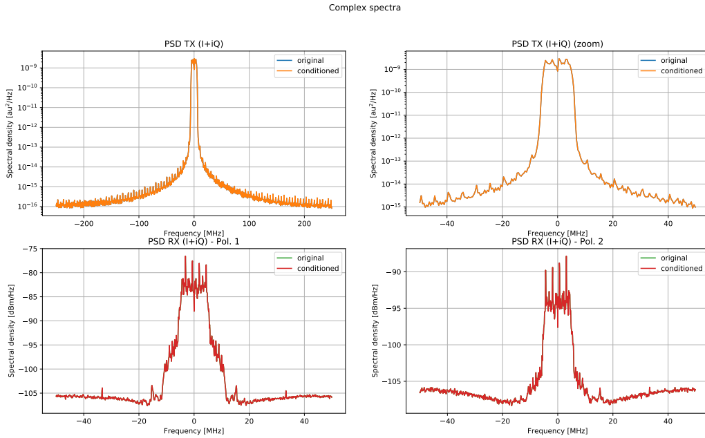
Figure 4.1: Power spectral densities at Alice's output and Bob's input. The complex spectrum corresponding to the I and Q components entering Alice's DAC is represented in the upper part of the figure (note that at this point the vertical units are arbitrary). The polarization diverse complex signals corresponding to the four inputs of Bob (I and Q for 2 polarizations) are displayed in the bottom part of the figure. They comprise the effects of transmitter, channel, detector (with TIA) and ADC. Note the clear spectral peaks observable in the detector response. Signal conditioning is off (original and conditioned are equal).
