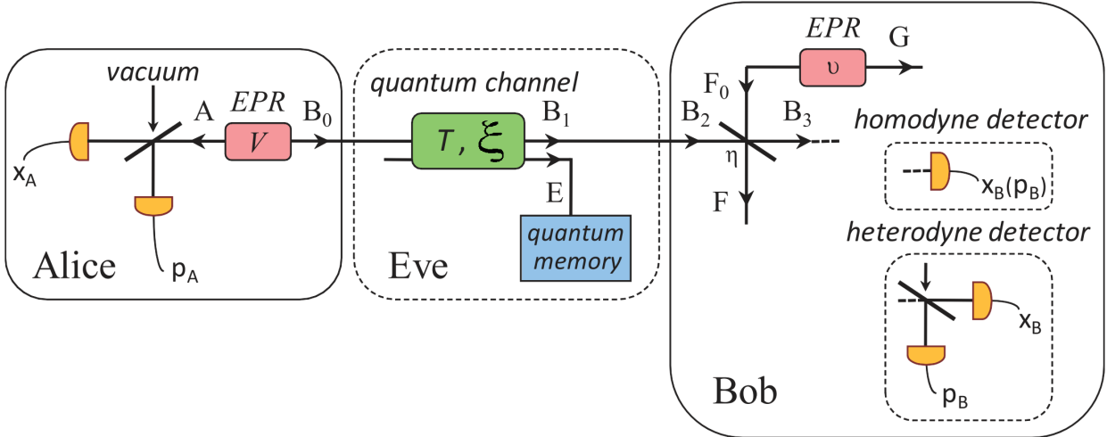
Figure 2.5: Entanglement version of the protocol including detector imperfections. Single (homodyne) and double (heterodyne) projections are considered. Each yellow block comprises a coherent detector as in figure 2.3.
