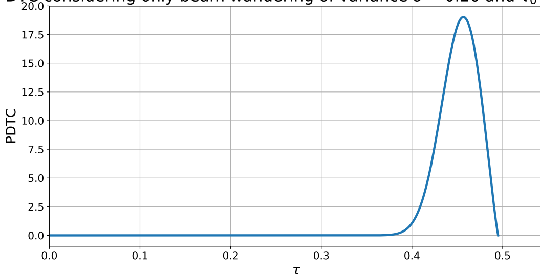
Figure 8.6: PDTC \mathcal{P}(\tau) for a receiver with aperture radius a = 0.75 m, beam width at receiver W = 2.0 m and beam wandering variance \sigma^2 = 0.2 \text{ m}^2 .
