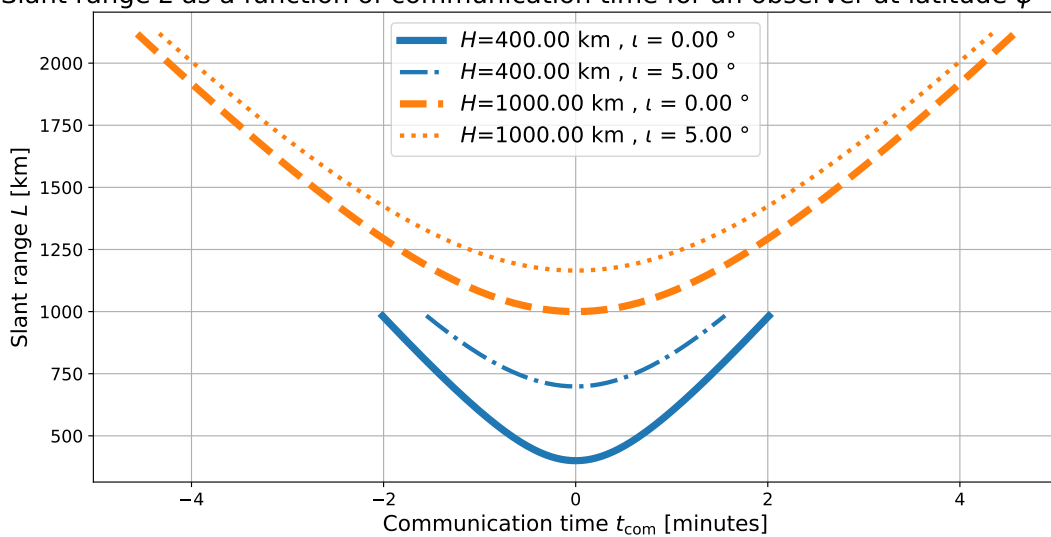
Slant range L as a function of communication time for an observer at latitude \psi=48.85^\circ
