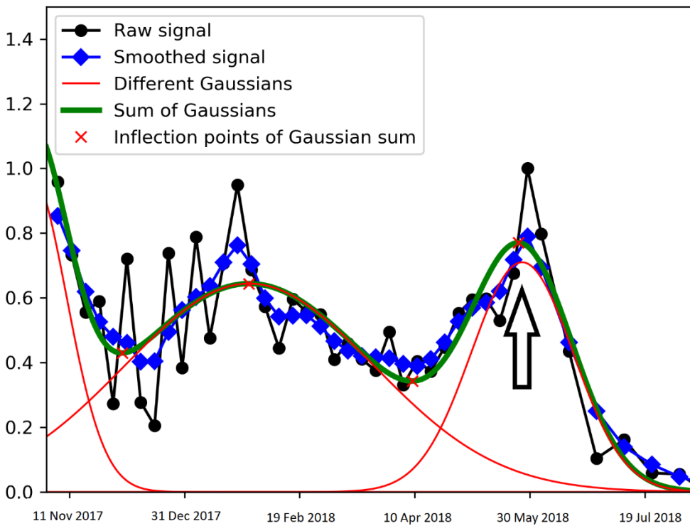
Figure 8 Gaussian fitting of the S1-VH temporal series of a winter wheat plot at the West Bekaa plain of Lebanon. The incidence angle is 43^{\circ} – 45^{\circ} . The x -axis represents the date and the y -axis refers to the normalized signal. The black arrow indicates the inflection point where soft dough had taken place.
