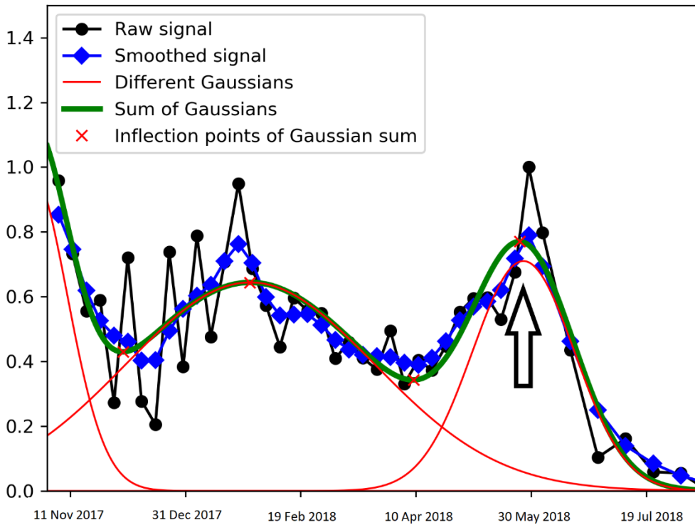
Figure 8 Gaussian fitting of the S1-VH temporal series of a winter wheat plot at the West Bekaa plain of Lebanon. The incidence angle is 43^{\circ} – 45^{\circ} . The x-axis represents the date and the y-axis refers to the normalized signal. The black arrow indicates the inflection point where soft dough had taken place.
