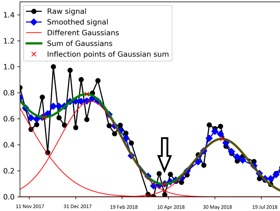
Figure 7 Gaussian fitting of the S1-VV temporal series of a winter wheat plot at the West Bekaa plain of Lebanon. The incidence angle is 32^{\circ} – 34^{\circ} . The x-axis represents the date and the y-axis refers to the normalized signal. The black arrow indicates the inflection point where heading had taken place.
