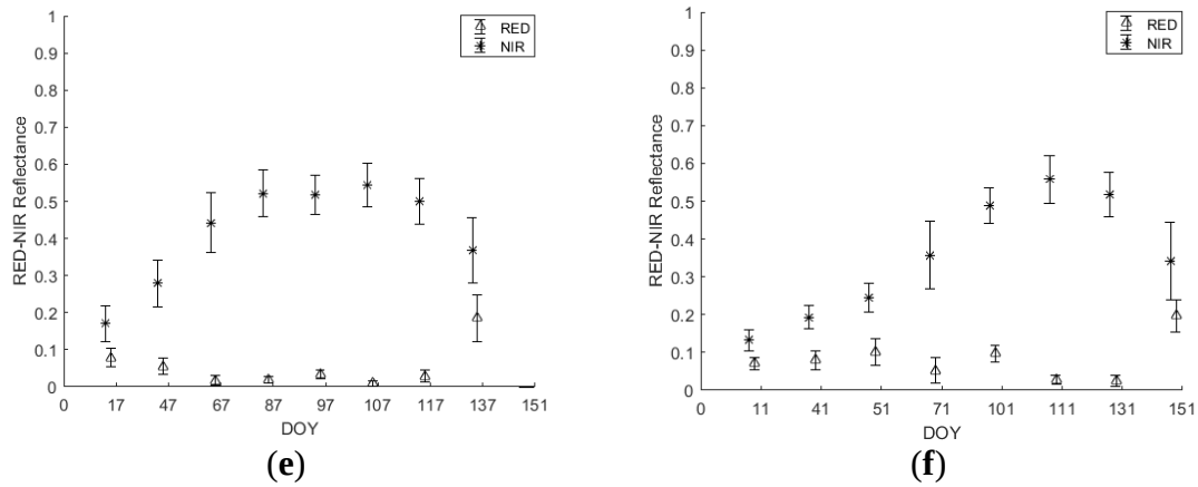
Figure 5 Mean \pm standard deviation of \rho RED and \rho NIR temporal profiles of Wheat (a) 2016 and (b) 2017; Barley (c) 2016 and (d) 2017 and Triticale (e) 2016 and (f) 2017.
