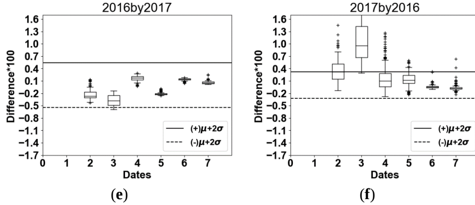
Figure 8 Differences of wheat reference segments when using the thresholds [\mu + 1\sigma] (a) 2016 when calibrated by 2017 and (b) 2017 when calibrated by 2016, [\mu + 1.5\sigma] (c) 2016 when calibrated by 2017 and (d) 2017 when calibrated by 2016 and [\mu + 2\sigma] (e) 2016 when calibrated by 2017 and (f) 2017 when calibrated by 2016.
