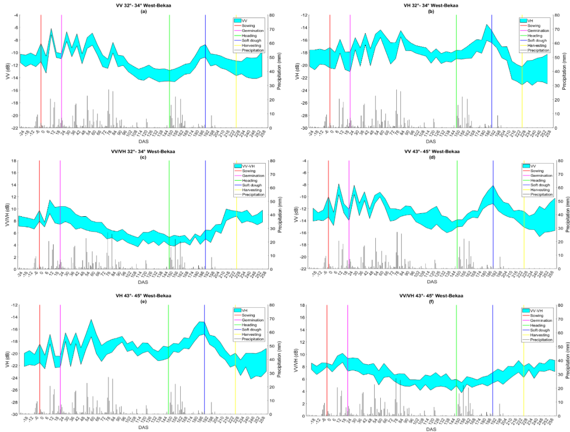
Figure 4 Winter wheat S1 (left y-axis) temporal profiles, which consist of VV (a and d), VH (b and e) and VV/VH (c and f) at low ( 32^\circ – 34^\circ ) and high ( 43^\circ – 45^\circ ) incidence angles of West Bekaa for the 2017–2018 cropping season versus time expressed as days after sowing (DAS) on the x-axis. On the temporal profiles, the daily precipitation is shown (right y-axis). On each profile, each of the three main phenological phases is denoted by a vertical line, in addition to sowing and harvesting dates.
