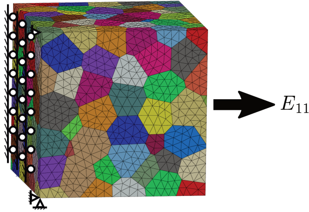
Figure 4.2: The starting mesh containing 256 equiaxed grains, 110,000 nodes and quadratic elements
