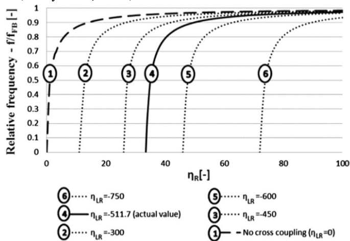
(b) Relative frequency as a function of non-dimensional rotational stiffness for several values of cross-coupling stiffness (Arany et al., 2015)
