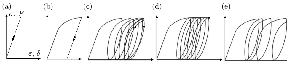
Figure 2.8.: Sketch of typical cyclic behaviour encountered during stress (or load) controlled cyclic tests (a) Purely elastic (b) Adaptation (c) Accommodation (d) Perfect ratcheting (e) Unstable ratcheting after Di Prisco and Muir Wood (2012)
