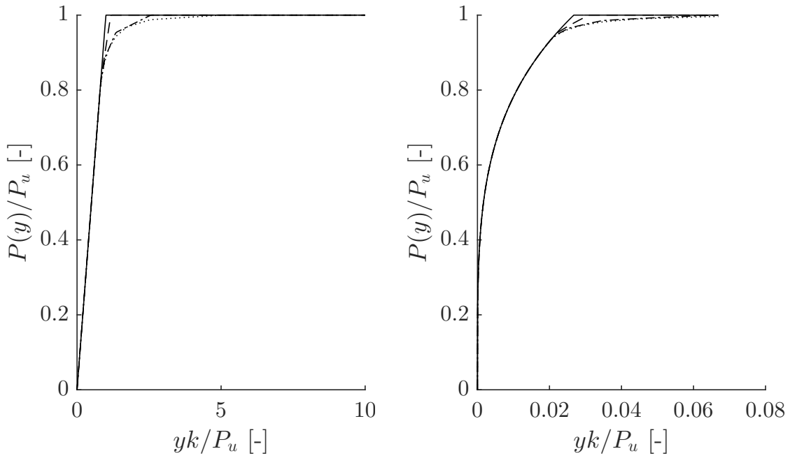
(a) for elasto-plastic P - y curve
