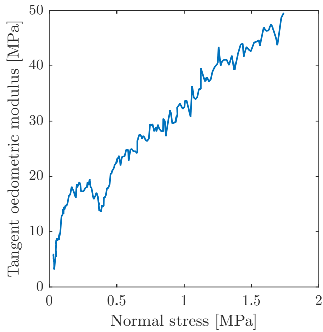
Figure 3.17.: Evaluation of the tangent oedometric modulus of the crushed rock at lows normal stresses
