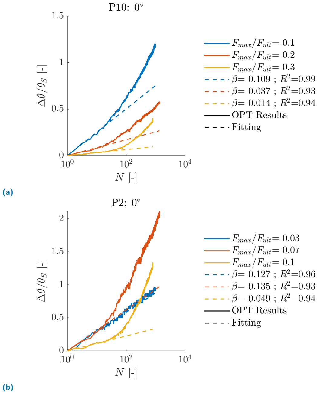
Figure 3.10.: Results of the fitting using Equation 3.3 for the accumulated rotations measured for pile P10 (top) and pile P2 (bottom)
