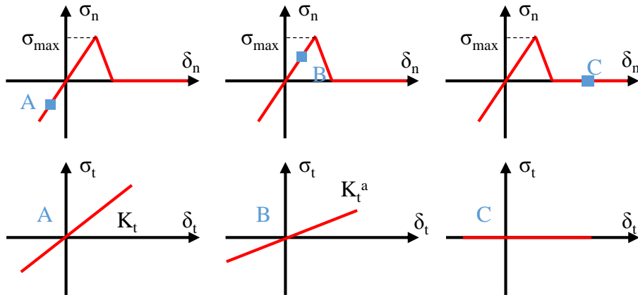
(b) Graphical representation of the coupling between the normal opening of the joint and the tangential component with K_t^a = \left(1 - \frac{\delta_n}{\kappa_{rupt} \tan \alpha \pi/4}\right) with \alpha \in ]0, 2]
