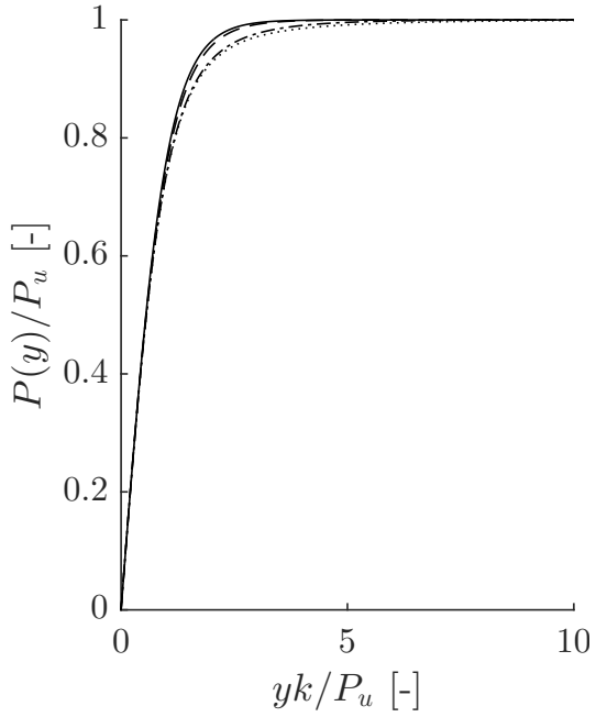
(c) for hyperbolic tangent P - y curve
